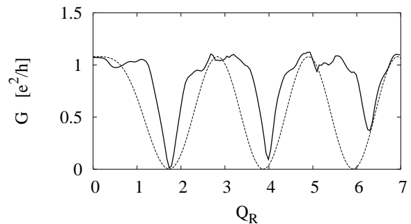
FIG. 4: Numerical calculation of the conductance modulation profile (solid line) of a single-mode 2D ring (Fig. 3, aspect ratio w/r_0 \approx 0.3 ) as a function of the dimensionless Rashba strength Q_R in the absence of an external magnetic field ( \mathbf{B} = 0 ). Dashed line: corresponding 1D result, Eq. (14) (same as solid line in Fig. 2) including a fitting prefactor at Q_R = 0 for comparison.
