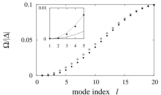
FIG. 6: Dispersion of low-energy spin excitations in a single-subband DMS quantum well for in-plane momentum \mathbf{k} = 0 , ferromagnetic coupling ( \Delta < 0 ), and dimensional cut-off N^+ = N^- = 20 , as a function of the mode index l (see text). The full circles depict the excitation energies \Omega_{(l)}^+(\mathbf{k} = 0) of even modes \omega_{(l)}^+ , while the empty circles correspond to \Omega_{(l)}^-(\mathbf{k} = 0) for odd modes \omega_{(l)}^- . The inset corresponds to two extreme quadratic fittings (dashed and dotted curves, see text) to the dispersion of even modes (full circle) for small l . The curves differ by a prefactor of order 3.5.
