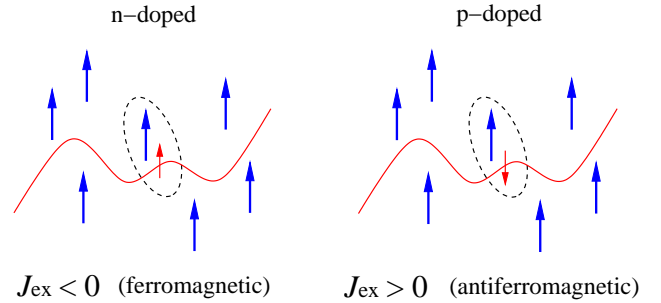
FIG. 1: Schematic representation of the exchange coupling between itinerant-carrier and localized magnetic-impurity spins in n-doped and p-doped DMSs. When the local moments are parallel to each other and the band system is spin-polarized, the exchange energy can be minimized for either ferromagnetic or antiferromagnetic interactions.
