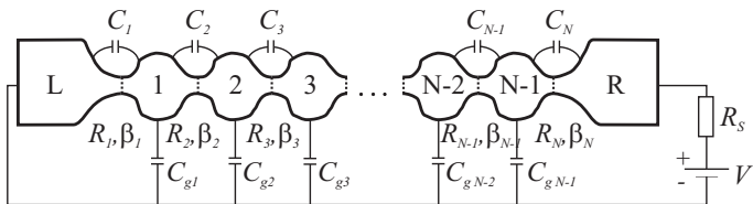
FIG. 1: 1D array of chaotic quantum dots. The array consists of N - 1 dots and N barriers. The n -th dot is characterized by mean level spacing \delta_n and gate capacitance C_{gn} . The n -th barrier is described by its Landauer conductance 1/R_n , capacitance C_n and Fano factor \beta_n . The array is placed in-between two big metallic reservoirs which are connected to the voltage source via Ohmic resistor R_S .
