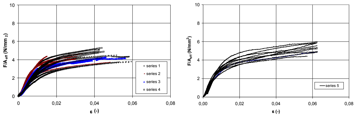
Figure 4: Stress-strain-diagrams for support loading (case 4).
