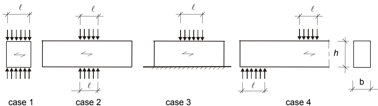
Figure 1: Different loading situations in compression perpendicular to the grain
