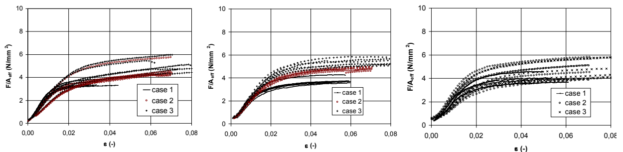
Figure 3: Stress-strain-diagrams for tests with h = 200 (left), 100 (middle) and 50 mm (right).
