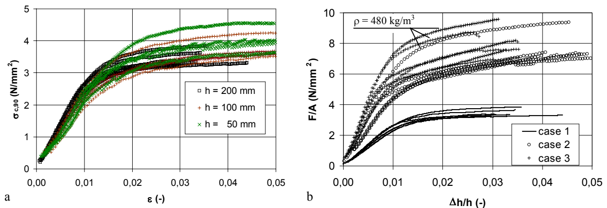
Figure 2: Stress-strain-diagrams, a) Case 1, h = 50, 100 and 200 \text{ mm} b) Cases 1, 2 and 3 with h = 200 \text{ mm}
