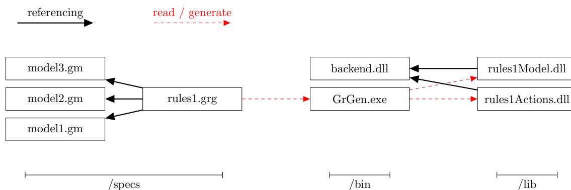
Figure 1.2: Generating a graph rewrite system
