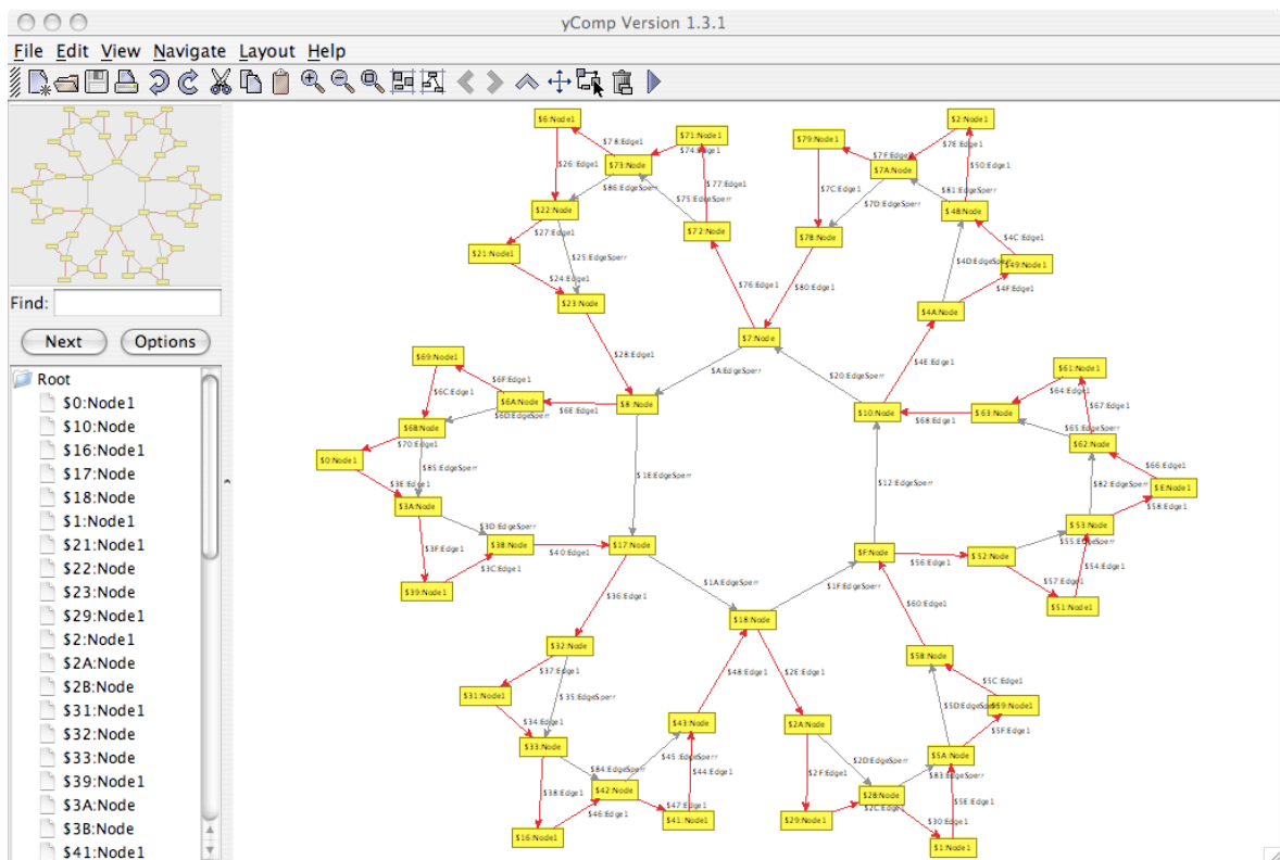
Figure 6.2: Koch snowflake
