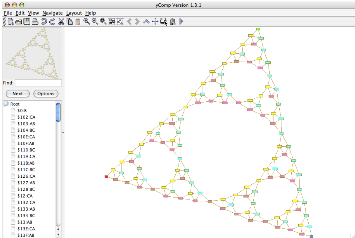
Figure 6.1: Sierpinski triangle
