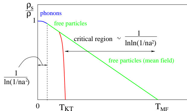
FIG. 6 Schematic phase diagram of a uniform dilute Bose gas. \rho_s is the superfluid density, normalized by the mass density of the gas \rho = mn , T_{KT} is the critical temperature of the Kosterlitz-Thouless transition, T_{MF} is the mean-field temperature, calculated perturbatively. Size of the transition critical region is defined by a parameter 1/\ln \ln(1/na^2) , where a is characteristic s-wave scattering length. The region, dominated by phononic quasi-particle behaviour is of the width 1/\ln(1/na^2) .
