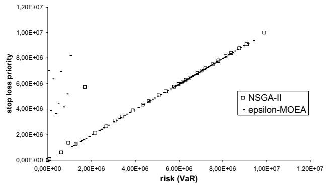
Abbildung 6.19: Stop loss L (Problem 4)
