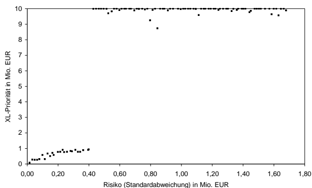
Abbildung 6.11: Excess of Loss R (Problem 2)
