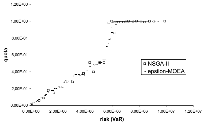
Abbildung 6.17: Quote a (Problem 4)
