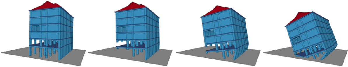
Figure 4: Visualization of the FE-simulation results at t_1 = 0 s, t_2 = 4.4 s, t_3 = 4.8 s, t_4 = 5.2 s
