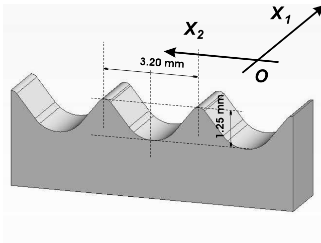
Figure 2: Geometrical structure of the corrugated rubber mat. Wavy periodical profile, CAD model.
