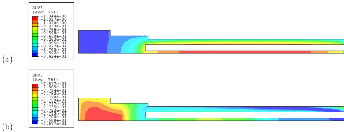
Figure 8.13: Calculated profile of the effective thermal conductivity: (a) at Step 6; (b) after unloading (unit, W/mK ).
