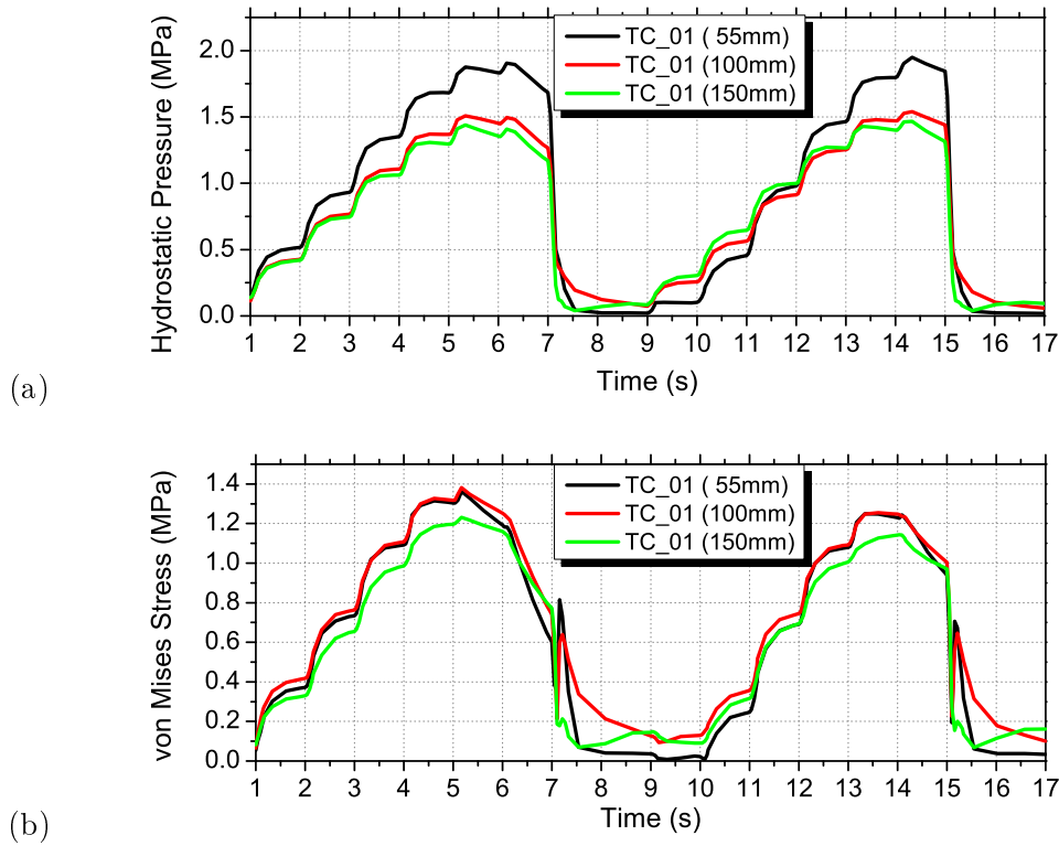
Figure 8.6: Stresses over time during two cycles: (a) hydrostatic pressure; (b) von Mises stress (unit: MPa ).
