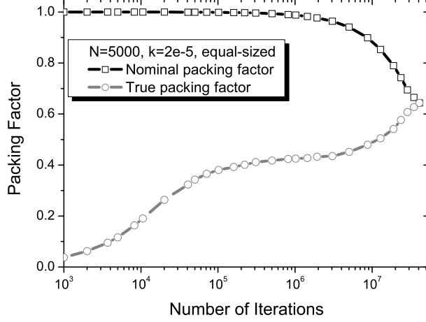
Figure 3.6: The evolution of the nominal and true packing factors over the number of iterations.
