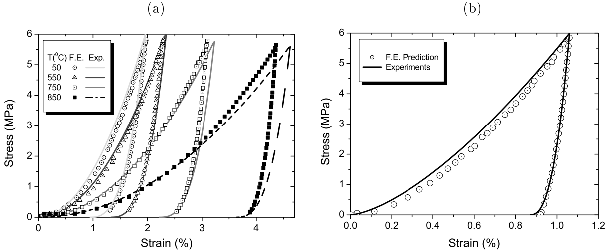
Figure 5.5: Uniaxial compression tests of: (a) \text{Li}_4\text{SiO}_4 under 50-850 °C; (b) beryllium pebble beds, comparison between FEA (dots) and empirical curves (lines).
