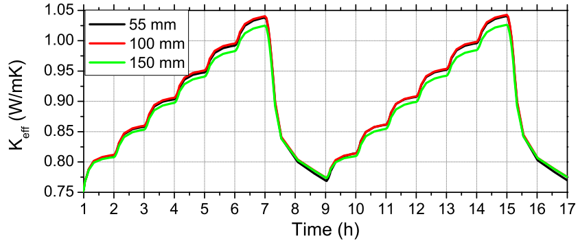
Figure 8.12: Effective thermal conductivity of the \text{Li}_4\text{SiO}_4 pebble bed over time at 55/100/150 mm of symmetric axis (unit, W/mK ).
