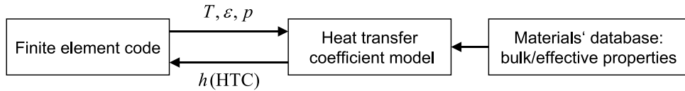
Figure 7.1: Interface between the HTC model and a finite element code.
