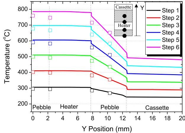
Figure 8.11: Temperature distributions at the cross-section 100\text{ mm} , at different steps. Solid lines, calculation; dots, measurements.
