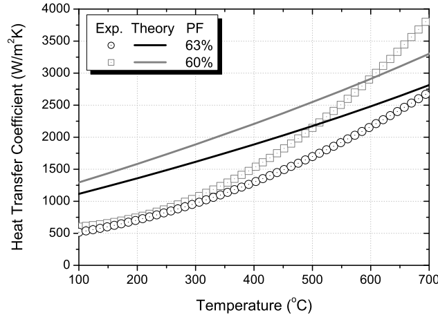
Figure 7.7: Comparison of the HTC model with data from Dalle Donne et al. (2000): the Be/stainless steel interface.
