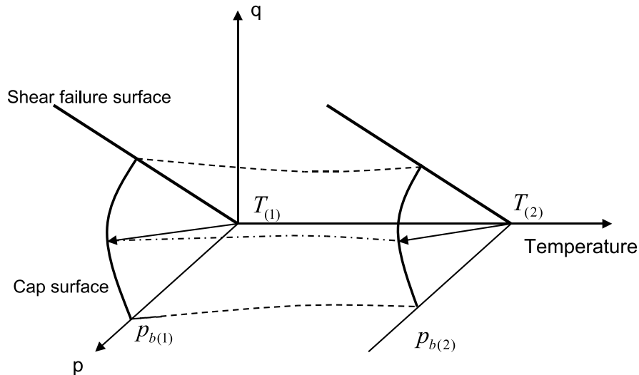
Figure 5.12: A sketch of the Drucker-Prager-Cap yielding/failure surfaces of thermo-plasticity.
