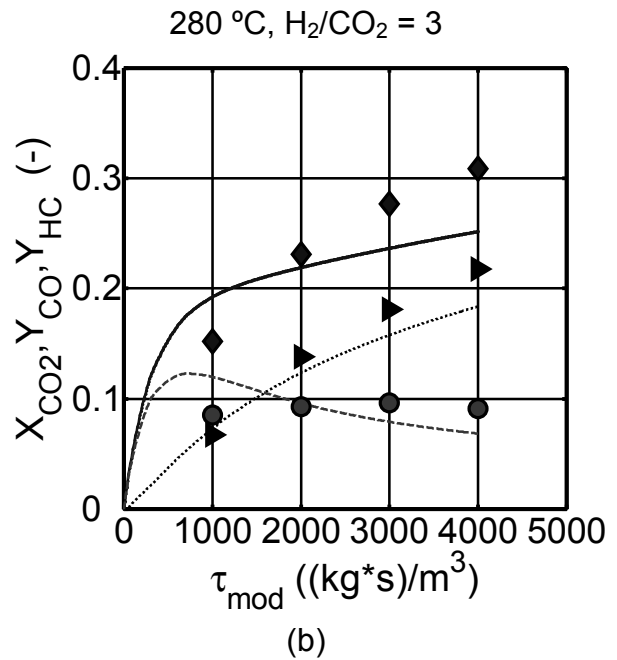
Fig. 12.13: CO 2 conversion (diamonds, solid curve), CO (circles, dashed curve) and hydrocarbons (triangles, dotted curve) yield. Catalyst: K-promoted Fe. Points: experimental, curves: calculated with kinetic model (Tab. 6.2, Eq. 5.31-5.32). p = 1 MPa.
