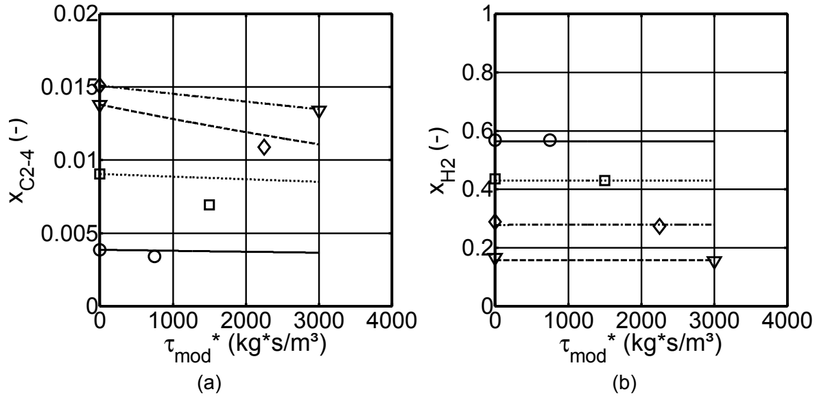
Fig. 7.7: Calculated and experimental molar fractions (curves, symbols) of n-C 2-4 (a) and H 2 (b) in Pt/ZSM-5 catalyst layer below the Co/Al 2 O 3 catalyst layer (dual-layer configuration). Reaction conditions and kinetics: see Fig. 7.4.
