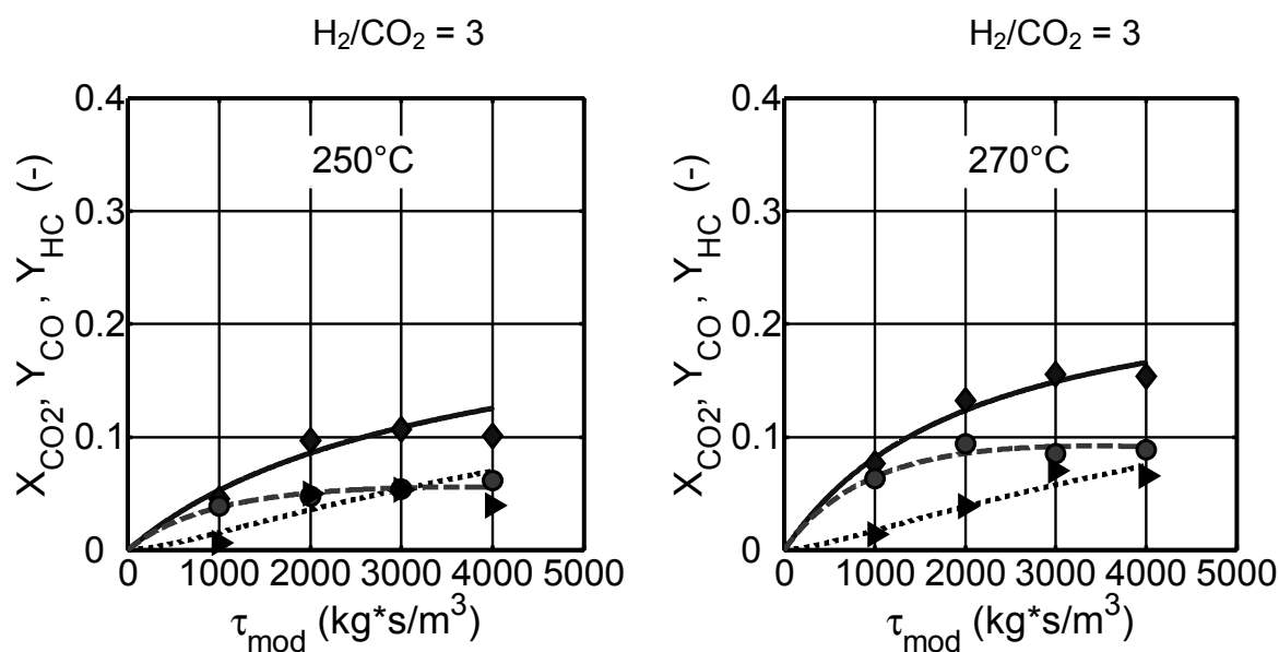
Fig. 6.18: Effect of temperature on CO 2 conversion (diamonds, solid curves), CO (circles, dashed curves) and hydrocarbons (triangles, dotted curves) yield versus modified residence time. Catalyst: K-promoted Fe. Points: experimental, curves: calculated with kinetic model (Tab. 6.2, Eq. 5.31-5.32). Reaction conditions see Table 5.9.
