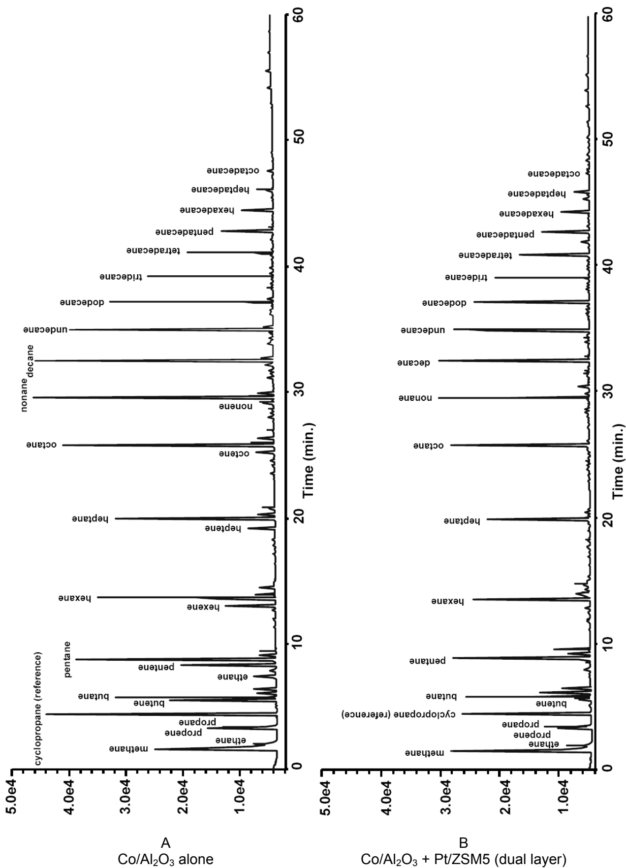
Fig 12.5: Example gas chromatograms from the gas phase (HP5890).
