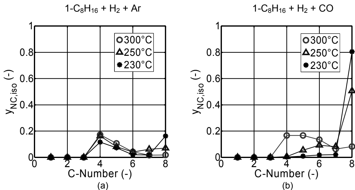
Fig. 6.5: Effect of CO and temperature on isomer content. Reactions of 1-C 8 H 16 with Pt/ZSM-5. Points: experimental, curves: trends. Definition of y_{NC,iso} see Equation 5.19. p = 0.5 MPa, WHSV = 0.22 h -1 . Other reaction conditions see Table 5.7.
