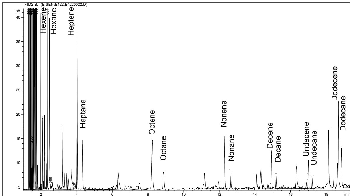
Fig. 12.2: Typical chromatogram of the organic compounds in the gas phase with cyclopropane as reference gas (HP6890N).
