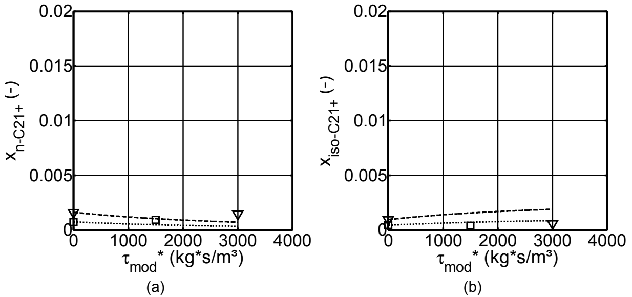
Fig. 12.25: Calculated and experimental molar fractions (curves, symbols) of the n-C 21+ (a) and iso-C 21+ (b) fractions in Pt/ZSM-5 catalyst layer below the K-promoted Fe catalyst layer (dual-layer configuration). Reaction conditions and kinetics: see Fig. 12.21.
