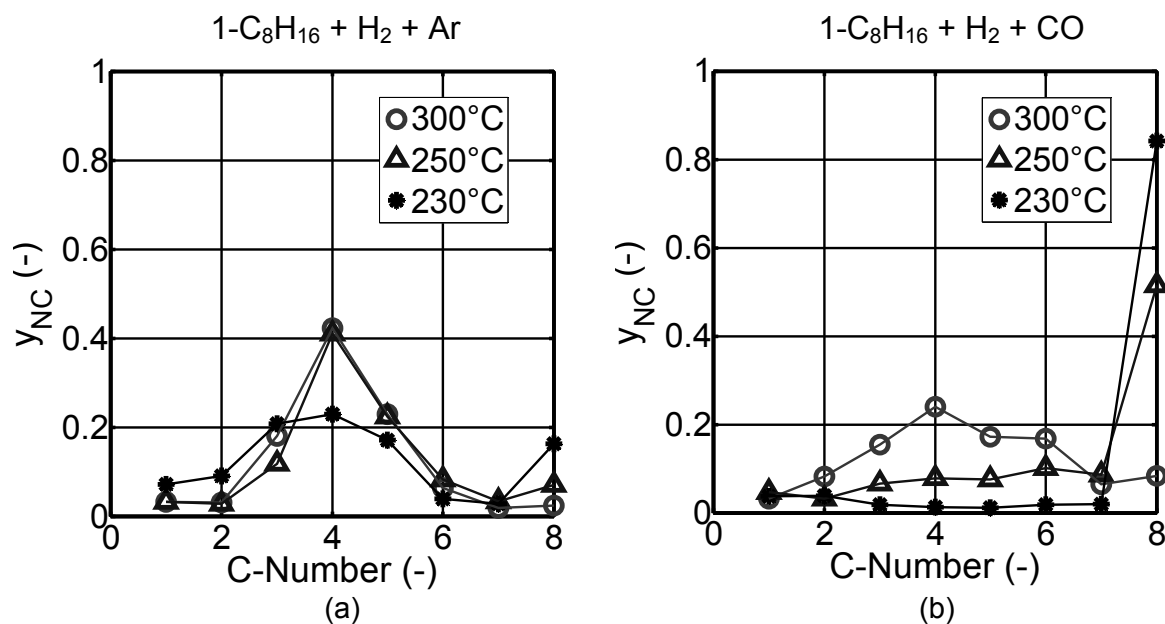
Fig. 6.4: Effect of CO and temperature on hydrocarbon molar fractions after hydrogenation, hydrocracking and hydroisomerisation reactions of 1-C 8 H 16 with Pt/ZSM-5. Points: experimental, curves: trends. p = 0.5 MPa, WHSV = 0.22 h -1 . Other reaction conditions see Table 5.7.
