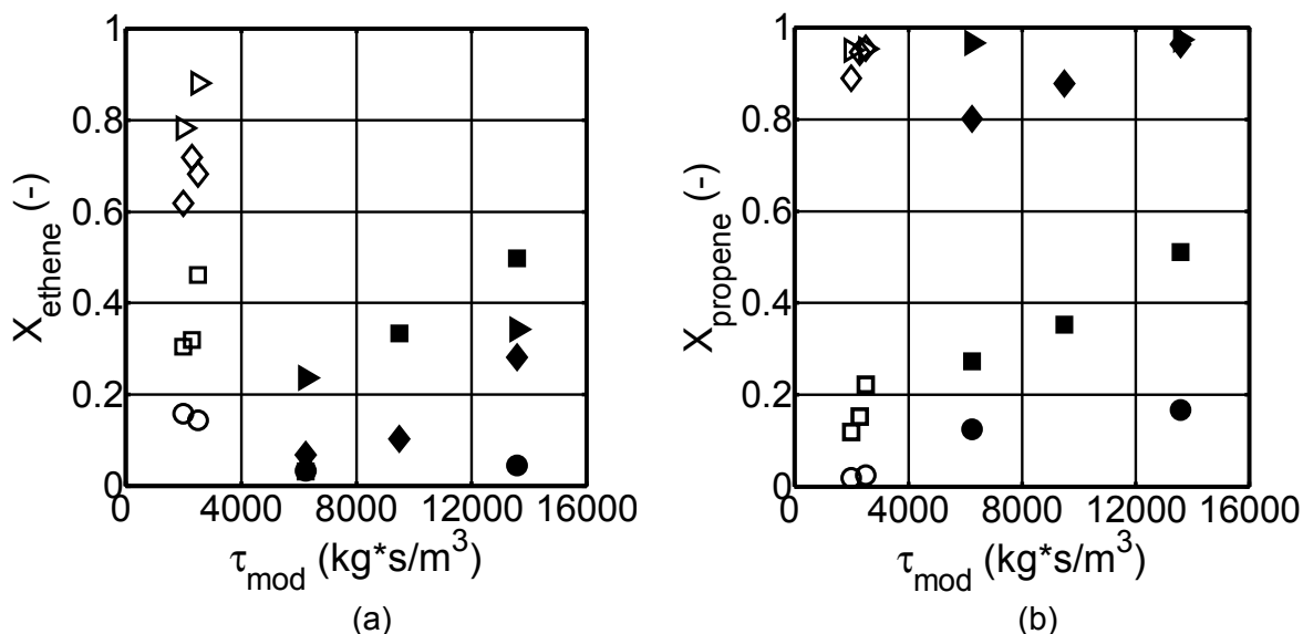
Fig. 6.8: Effect of the presence of synthesis gas and temperature on ethene (a) and propene (b) conversion versus modified residence time on Pt/ZSM-5. Feed: C_2H_4 + C_3H_6 + H_2 + CO + N_2 (open symbols), C_2H_4 + C_3H_6 + N_2 (full symbols). T = 215 °C (circles), 230 °C (squares), 250 °C (diamonds), 270 °C (triangle), p = 1 MPa. Ranges of other reaction conditions see Table 5.8.
