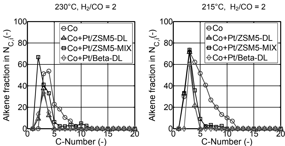
Fig. 6.27: Effect of temperature, bifunctional catalyst and catalyst-bed configuration on alkene content in carbon-number fractions in the gas phase. Catalysts: Co/Al 2 O 3 , Pt/ZSM-5, Pt/Beta. Reaction conditions: see Fig. 6.25.
