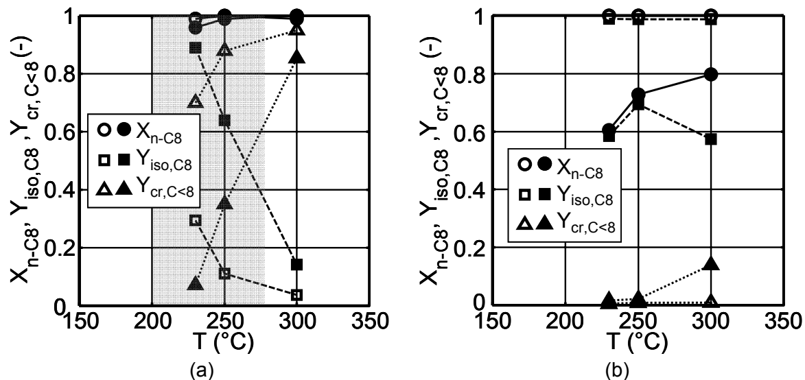
Fig. 9.2: Reactions of 1- \text{C}_8\text{H}_{16} without CO (open symbols) and with CO (full symbols). Feed: 1- \text{C}_8\text{H}_{16} + \text{H}_2 + Ar or CO. Catalyst: (a) Pt/ZSM-5, (b) Pt/Beta. Points: experimental, curves: trends. Grey range: low temperature FTS. p = 0.5 \text{ MPa} , \text{WHSV} = 0.22 \text{ h}^{-1} . Other reaction conditions see Table 5.7.
