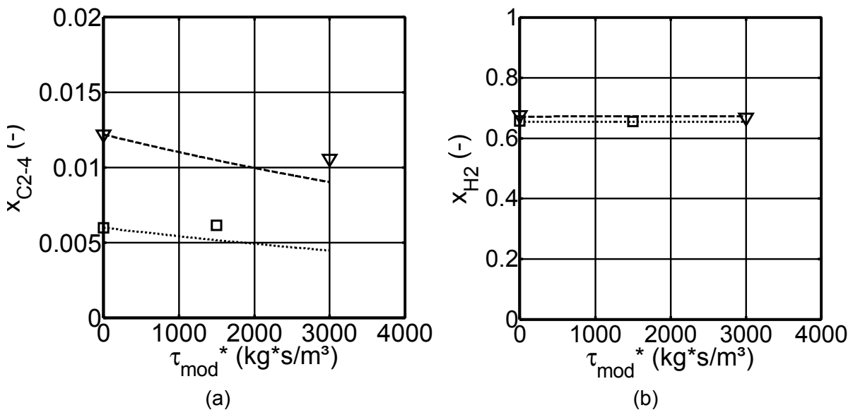
Fig. 12.26: Calculated and experimental molar fractions (curves, symbols) of the C 2-4 fraction (a) and H 2 (b) in Pt/ZSM-5 catalyst layer below the K-promoted Fe catalyst layer (dual-layer configuration). Reaction conditions and kinetics: see Fig. 12.21.
