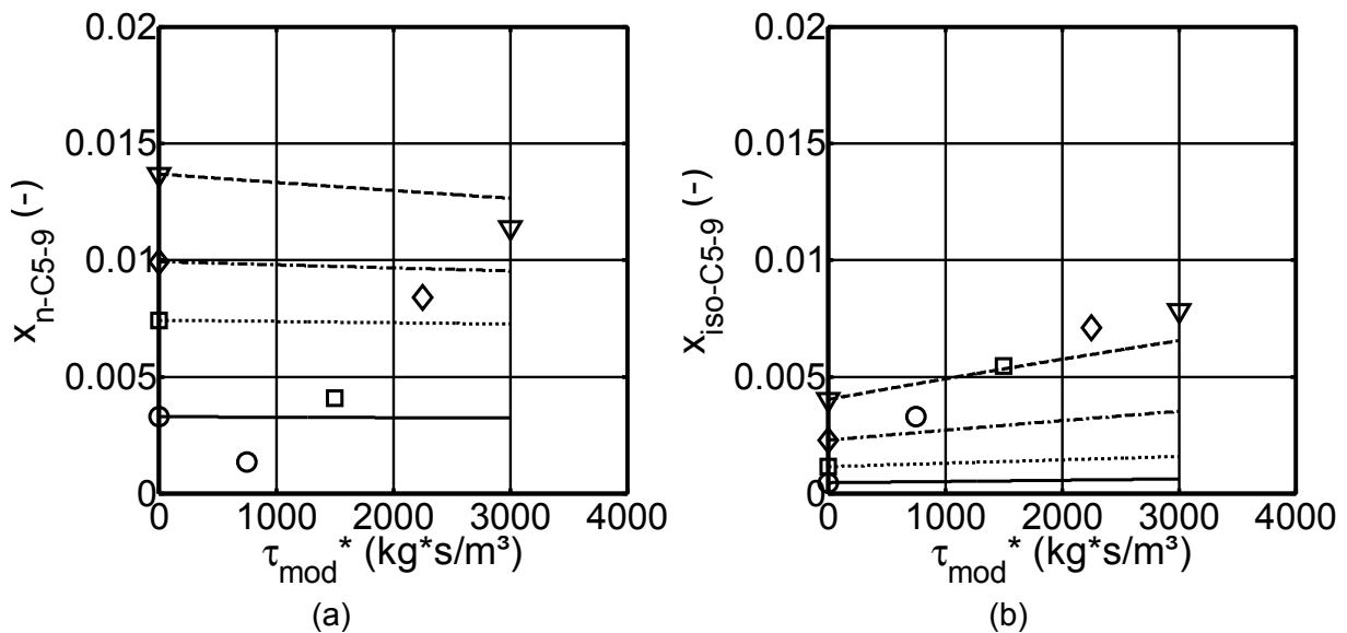
Fig. 7.4: Calculated and experimental molar fractions (curves, symbols) of n-C 5-9 (a) and iso-C 5-9 (b) in Pt/ZSM-5 catalyst layer below the Co/Al 2 O 3 catalyst layer (dual-layer configuration). \tau_{\text{mod}} = 4000 (triangles), 3000 (rhombus), 2000 (squares) and 1000 (circles) \text{kg}\cdot\text{s}/\text{m}^3 . T = 230 °C, p = 1 MPa, (p_{\text{H}_2}/p_{\text{CO}})_{\text{in}} = 2 . Kinetics: Tab. 7.3, Eq. 7.2-7.4.
