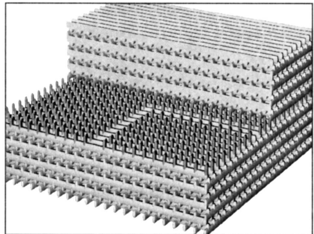
Fig. 1. Scheme of a 3D–2D–3D photonic crystal heterostructure. The foreground corresponds to the first set of experiments (i) presented in Fig. 2, and the background corresponds to the second set of experiments (ii) shown in Fig. 3.
