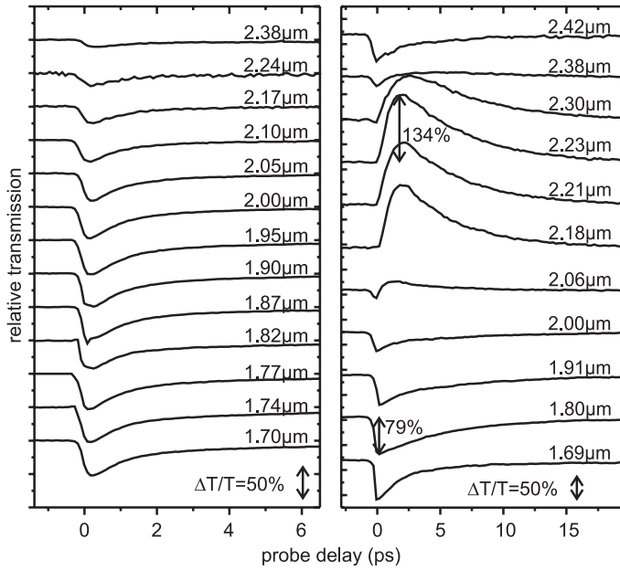
Fig. 3 Pump–probe traces for several probe wavelengths (as indicated), vertically displaced for clarity. LHS column: As-grown sample (a-Si), \lambda_{\text{pump}} = 1.84 \mu\text{m} , I_{\text{pump}} = 66 \text{ GW/cm}^2 ; RHS column: Tempered sample (polycrystalline Si), \lambda_{\text{pump}} = 1.73 \mu\text{m} , I_{\text{pump}} = 90 \text{ GW/cm}^2 . All curves in one column are shown on the same scale of transmission relative to the unexcited sample (see arrows). Note the different time scales on the LHS and RHS, respectively.
