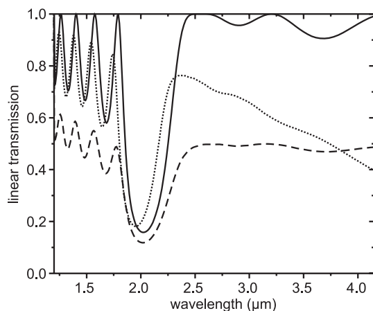
Fig. 4 Calculated transmission for three different parameter sets. The solid curve shows the linear spectrum (i.e., n_e = 0 ). The other two curves correspond to an optically excited electron density of n_e = 1.5 \times 10^{20} \text{ cm}^{-3} and \tau = 0.5 \text{ fs} (dashed curve) and \tau = 10 \text{ fs} (dotted curve), respectively.
