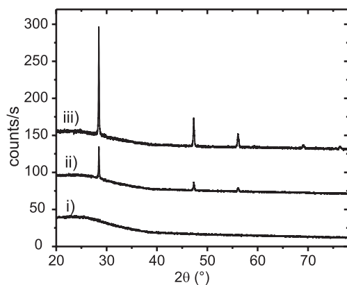
Fig. 2 X-ray diffraction measurements of a 1 \mu\text{m} thick silicon film on glass substrate, vertically displaced by 60 counts/s. i): untempered; ii): tempered for 7 hours at 600 °C; iii): tempered for 22 hours at 600 °C.
