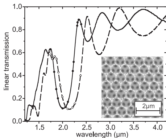
Fig. 1 Linear transmission spectra of the Silicon inverse opal in [111] direction, as-grown (dashed) and tempered (solid). The dots correspond to the probe wavelengths investigated in Fig. 3. The inset shows an SEM image of the sample surface.
