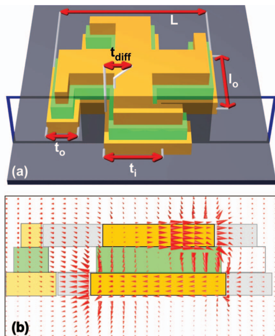
Fig. 1. (a) Scheme of the double-layer magnetic metamaterial. The geometrical parameters are indicated and given by L=274 nm, t_i=90 nm, l_o=135 nm, t_o=50 nm, and t_{diff}=15 nm (b) Snapshot of the \vec{E} -field at 0.86 \mu\text{m} wavelength for lcp incident light. The cutting plane is indicated in (a).
