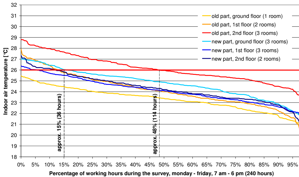
Figure 4: Indoor (air) temperatures in the rooms where the survey was carried out. The red line corresponds to the temperature limit of the German workplace regulations.
