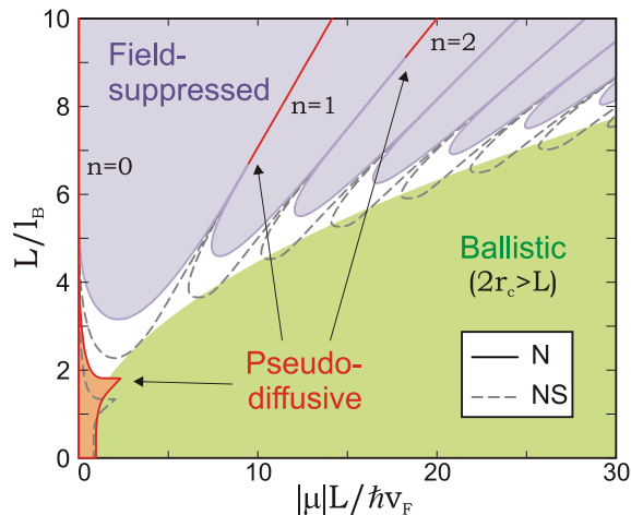
FIG. 2: (Color online) Phase diagram representing the crossovers from localized, pseudo-diffusive and ballistic transport regimes in the field-doping parameter plane. Solid (dashed) lines represent the boundaries for a N (NS) junction. LLs are labeled by n .
