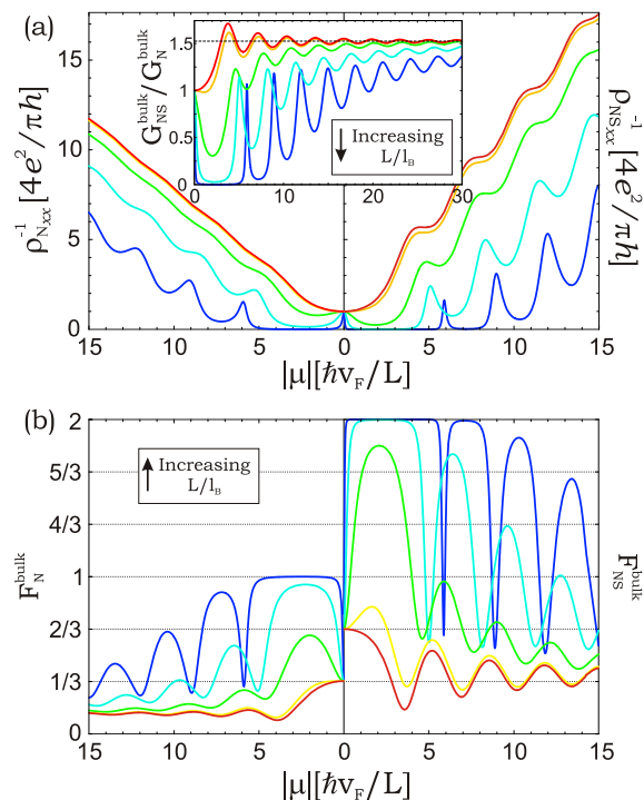
FIG. 1: (Color online) Inverse longitudinal resistivity in units of 4e^2/\pi h (a) and bulk Fano factor (b) for the N (left) and NS (right) junctions as a function of the (absolute value of the) Fermi energy (in units of \hbar v_F/L ). Different curves correspond to different values of L/l_B (where l_B \equiv \sqrt{\hbar/eB} ), which ranges from zero for red curve to four for the dark blue one in steps of one. The same for the ratio G_{NS}^{\text{bulk}}/G_N^{\text{bulk}} in the inset.
