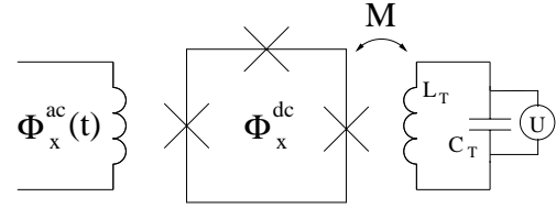
FIGURE 1. In the setup of Ref. [1] an externally driven three-junction flux qubit is coupled inductively to an LC oscillator.
