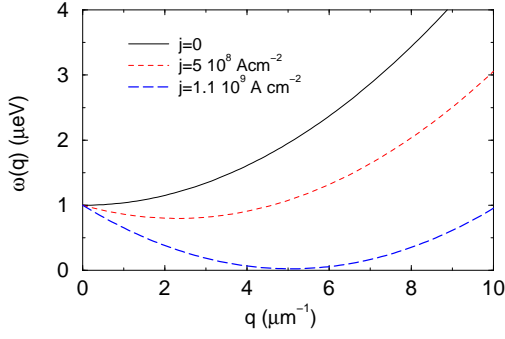
FIG. 2: Current modified spin-wave spectrum
