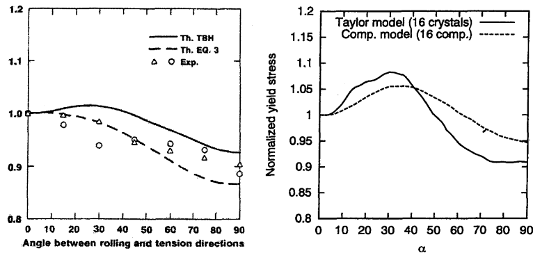
Fig. 2. Normalized yield stress versus tensile direction. Left: numerical and experimental results taken from Lege et al. [1]. Right: prediction of the texture component model and the Taylor model, respectively.
