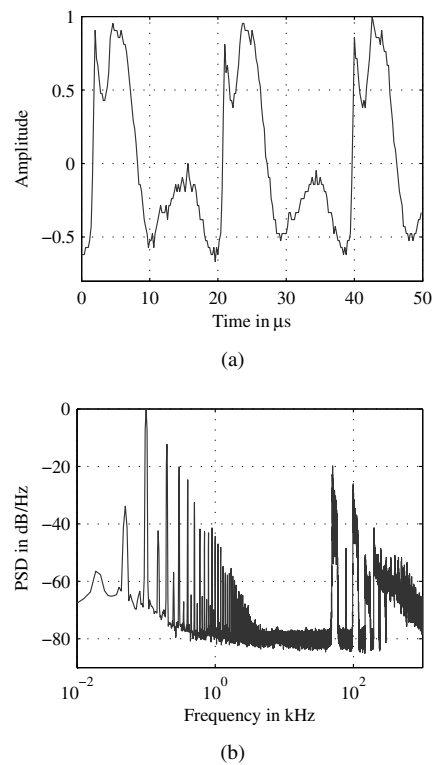
Fig. 4. Anode oscillations of compact fluorescent lamp Osram Dulux EL 23 with electronic ballast: (a) Time Waveform (b) Welch Power Spectral Density Estimate
