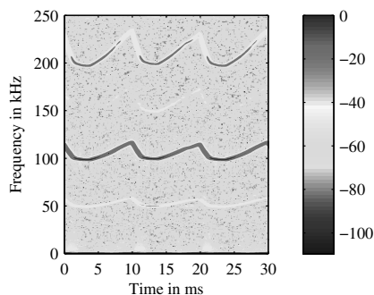
Fig. 3. Spectrogram of compact fluorescent lamp Osram Dulux EL 23 using Short Time Fourier Transform
