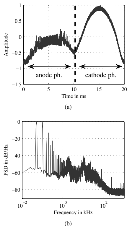
Fig. 1. Anode oscillations of fluorescent lamp Philips Master TL-D Super 80 18W/840 driven by an Tridonic Atco EC 18 C501 K reactive ballast: (a) Time Waveform (b) Welch Power Spectral Density Estimate
