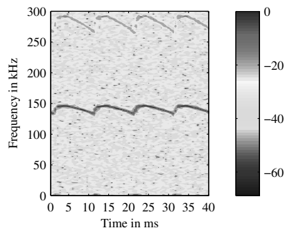
Fig. 6. Spectrogram of 7 W Light Emitting Diode Philips Master LED E27 A55 MV bulb lamp using Short Time Fourier Transform
