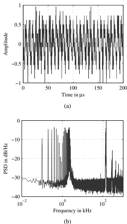
Fig. 5. 7 W Light Emitting Diode Philips Master LED E27 A55 MV bulb lamp: (a) Time Waveform (b) Welch Power Spectral Density Estimate
