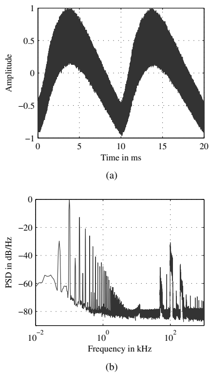
Fig. 2. Compact fluorescent lamp Osram Dulux EL 23 with electronic ballast: (a) Time Waveform (b) Welch Power Spectral Density Estimate
