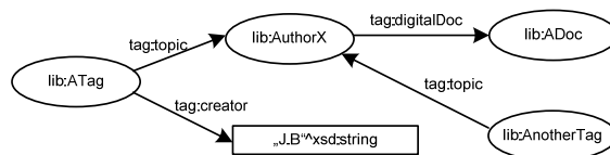
Figure 4: Example of a RDF graph
