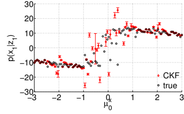
(c) CKF distributions can be overconfident and incoherent.
