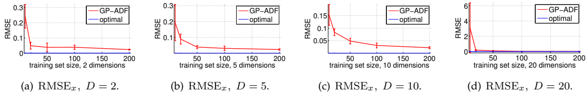
Figure 4.4: RMSE_x as a function of the dimensionality and the size of the training set. The x -axes show the size of the training set employed, the y -axes show the RMSE of the GP-ADF (red line) and the RMSE of the optimal filter (blue line). The error bars show the 95% confidence intervals. The different panels show the graphs for D = 2, 5, 10, 20 dimensions, respectively. Note the different scales of the y -axes.
