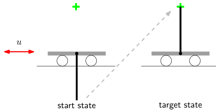
Figure 3.16: Cart-pole setup. The cart-pole system consists of a cart running on an infinite track and a freely swinging pendulum attached to the cart. Starting from the state where the pendulum hangs down, the task was to swing the pendulum up and to balance it in the inverted position at the cross by just pushing the cart to left and right. Note that the cart had to stop exactly below the cross in order to fulfill the task optimally.
