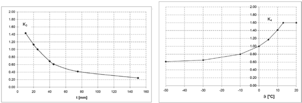
Fig. 10: Influence of the material thickness K_3 and the component temperature K_4 on K_c
