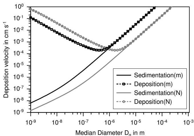
Figure 3.3.: Deposition of number (N) and mass density (m) for distributions with \sigma_g = 2 m and r_a = 50 \text{ s m}^{-1} as a function of the geometric median diameter D_g .
