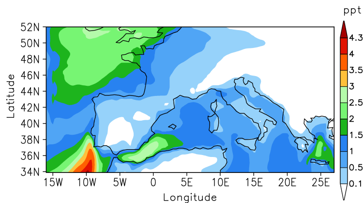
Figure 6.9.: Simulated DMSO mixing ratio, averaged over three days.
