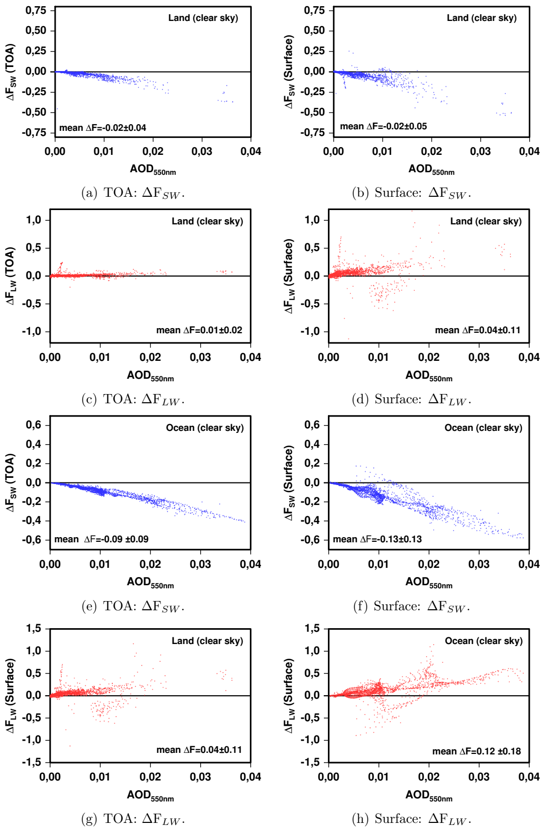
Figure 6.44.: Change (run F-run R) of the solar and thermal radiation budgets at cloud free conditions as a function of simulated AOD, averaged over three days.
