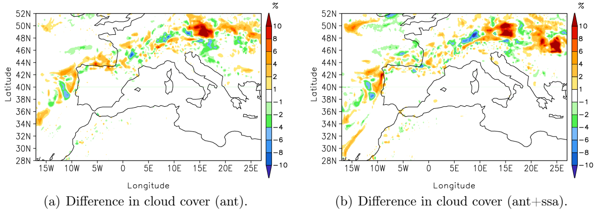
Figure 6.55.: Simulated change in the total cloud cover due to anthropogenic aerosol and composite aerosol, respectively, averaged over 24th-26th July.
