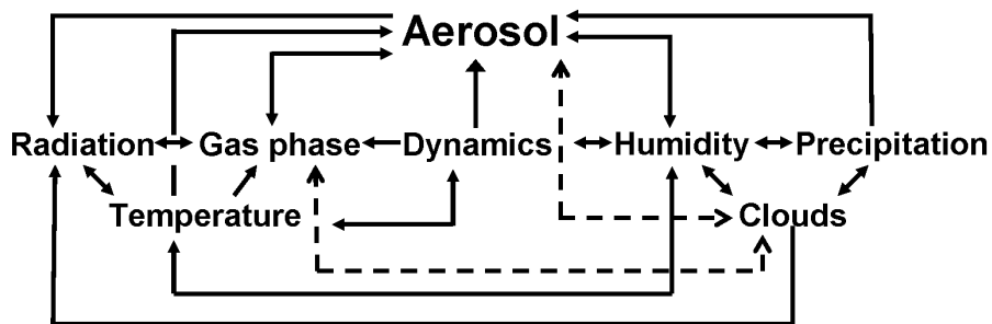
Figure 3.2.: The feedback loop accounted for in COSMO-ART.
