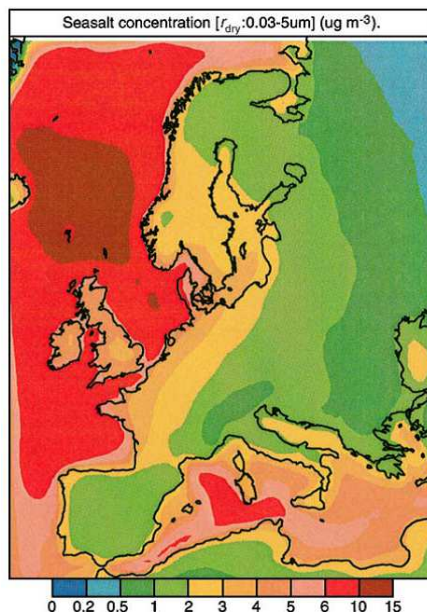
Figure 2.4.: Average sea salt mass concentration in \mu\text{g m}^{-3} in the surface layer for January 1999-December 2001 for sea salt with a dry radius of up to 5 \mu\text{m} from Foltescu et al. (2005).
