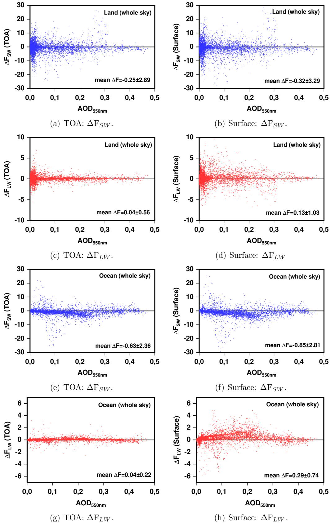
Figure 6.43.: Change (run F-run R) of the solar and thermal radiation budgets under all conditions as a function of simulated AOD, averaged over three days.
