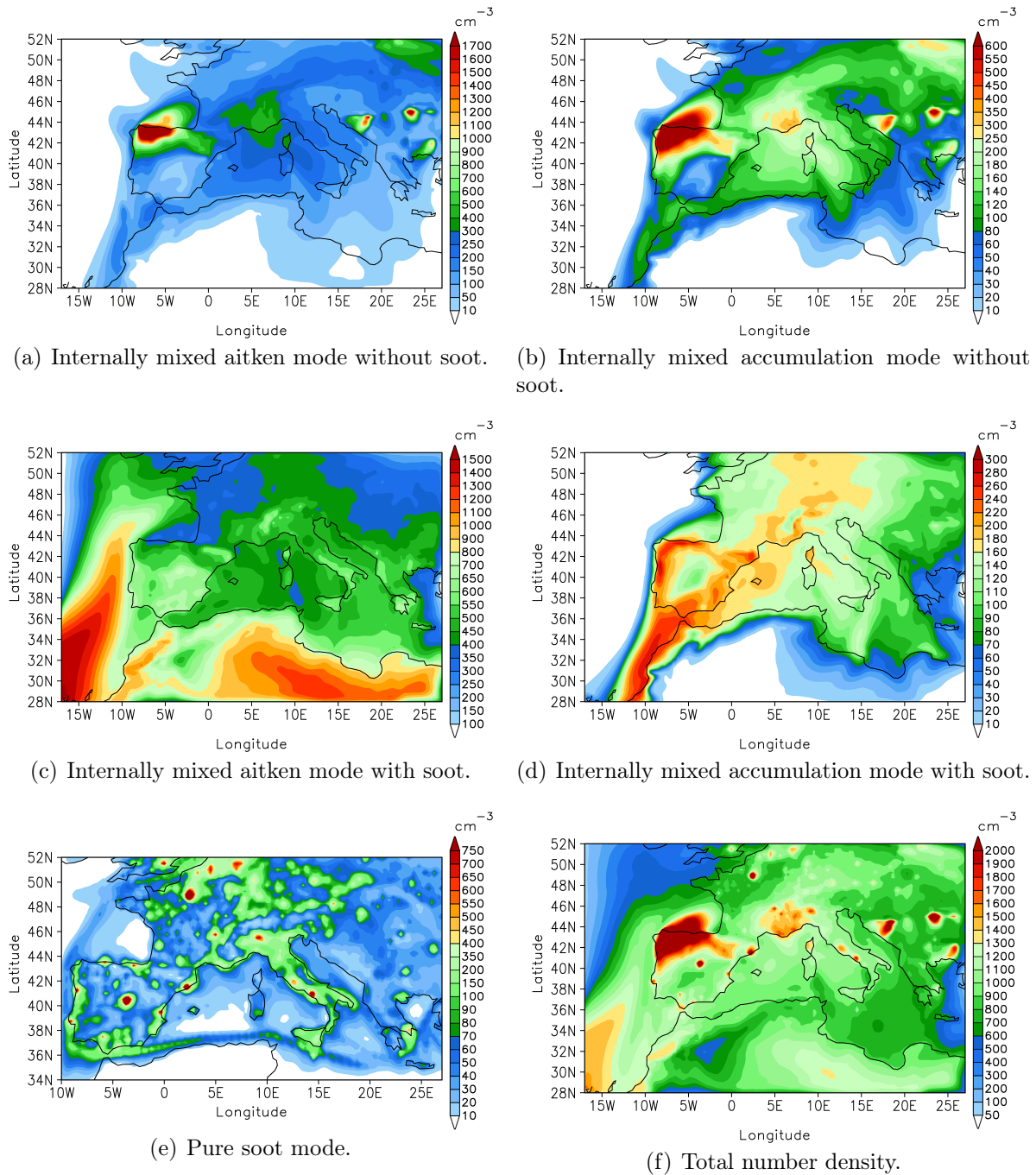
Figure 6.50.: Simulated anthropogenic number densities near the surface for the lowest approx. 40 m.
