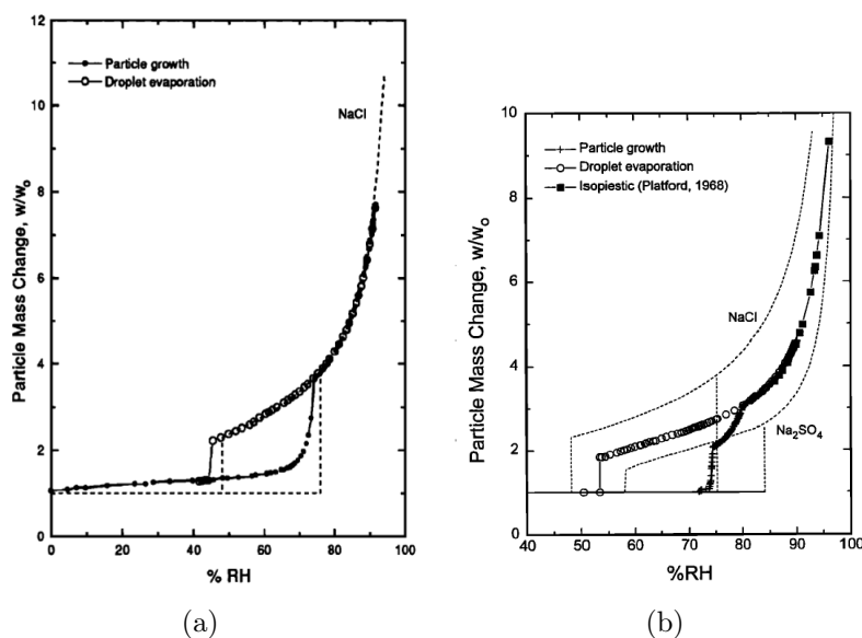
Figure 2.5.: (a): Water uptake of sea salt aerosol (circles) compared to pure NaCl particle (dotted line) as a function of RH. Reproduced from Tang et al. (1997). (b): Water uptake of mixed NaCl-Na 2 SO 4 particle (circles) compared to the single salt behaviour of NaCl and Na 2 SO 4 (dotted line). Reproduced from Tang (1997).
