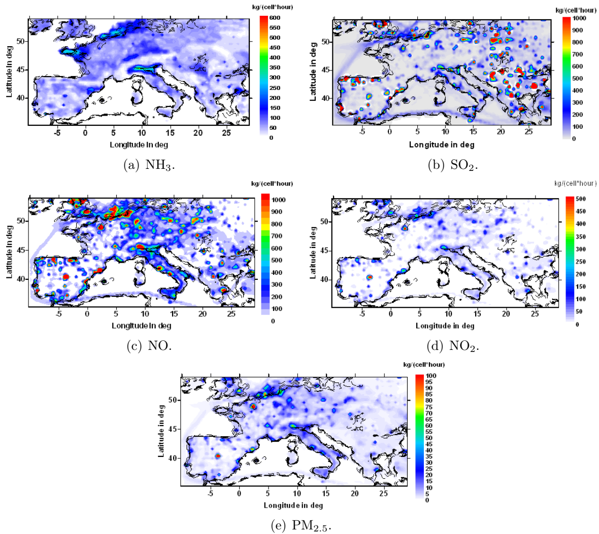
Figure 6.7.: Vertical sum of the emissions at 7 UTC.
