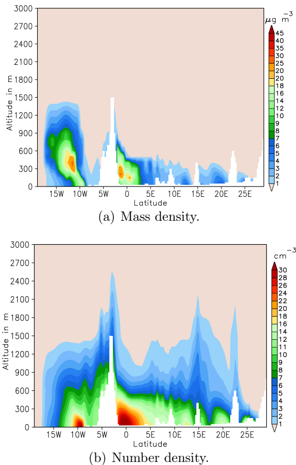
Figure 6.31.: Vertical cross sections at 37^\circ\text{N} of 3-day averages of the mass and number density, respectively.
