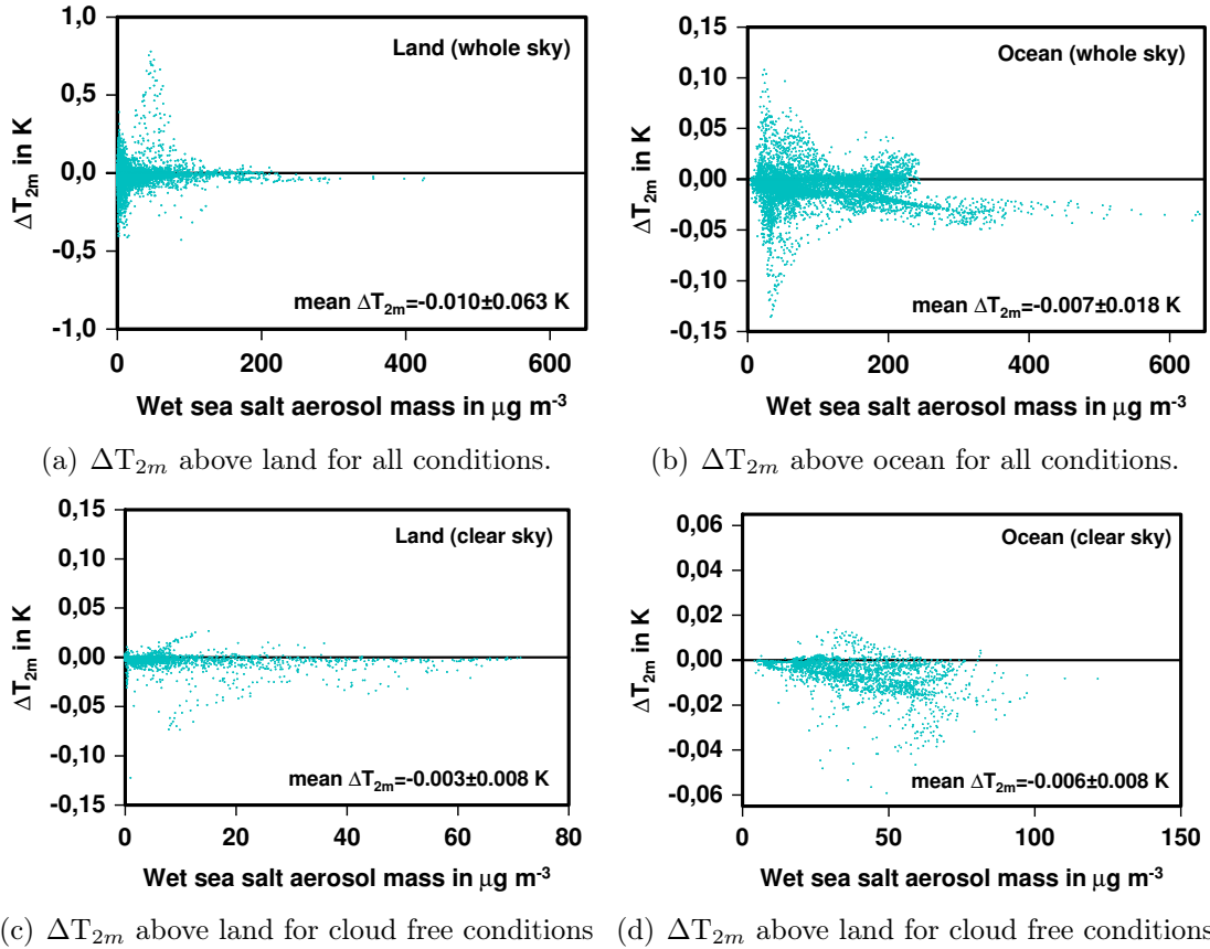
Figure 6.46.: \Delta T at 2m as a function of average aerosol mass (run F-run R), averaged over three days.
