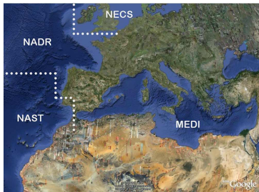
Figure 4.1.: The considered DMS sea water provinces.
