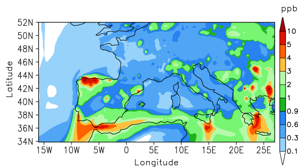
Figure 6.12.: Simulated SO 2 from DMS oxidation and anthropogenic emissions, near the surface averaged over three days.
