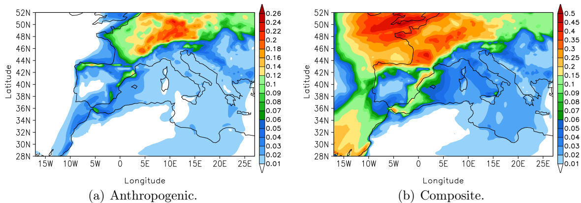
Figure 6.52.: Simulated mean anthropogenic \text{AOD}_{550} and mean sea salt and anthropogenic composite \text{AOD}_{550} . Please note the different scales.
