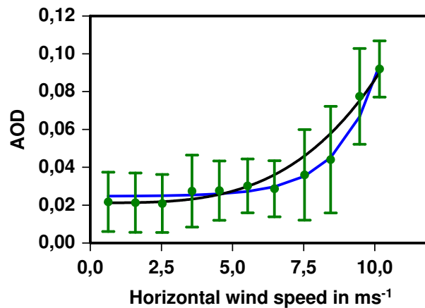
Figure 6.36.: Power law fit based on average AOD_{550} values ( R=0.998 ) in black and exponential fit ( R=0.938 ) in blue.
