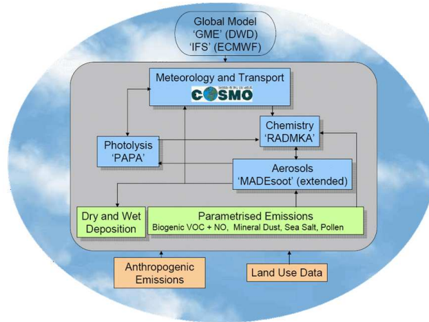
Figure 3.1.: The model system COSMO-ART.
