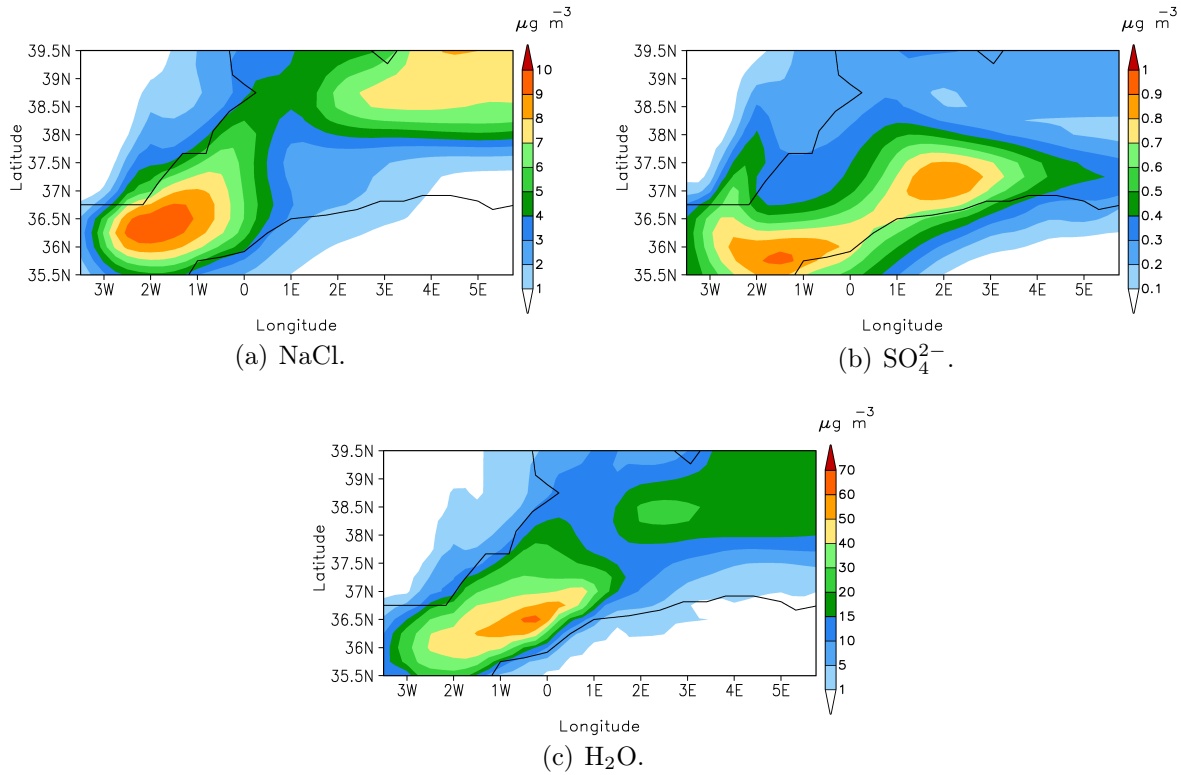
Figure 5.1.: Pre-simulated mass densities of the respective chemical components of the film mode for the lowest approx. 40 m.
