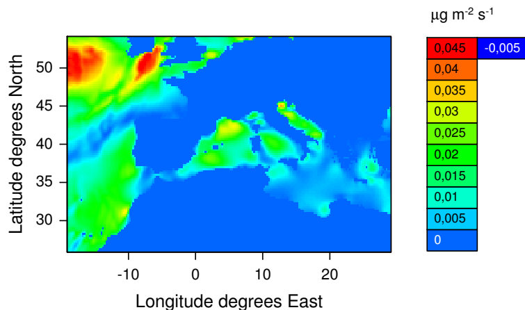
Figure 6.6.: Simulated DMS emission flux on 25th July, 8 UTC.
