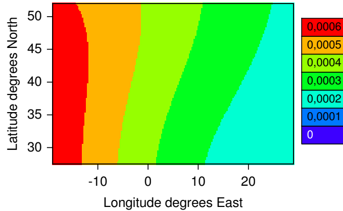
Figure 3.4.: Maritime aerosol optical depth in GRAALS.
