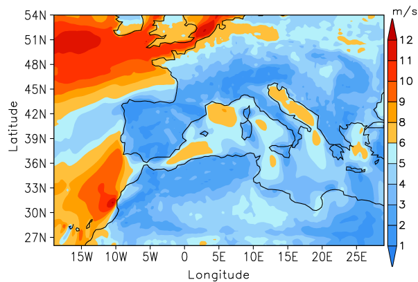
Figure 6.34.: U_{10} averaged over 24th-26th July.
