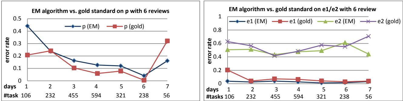
Figure 3: Estimations made by the EM algorithm vs. gold standard
