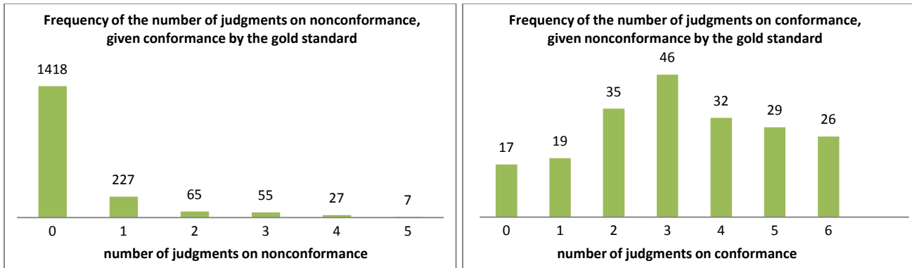
Figure 6: Frequency of number of judgments on nonconformance (conformance), given conformance (non-conformance)
