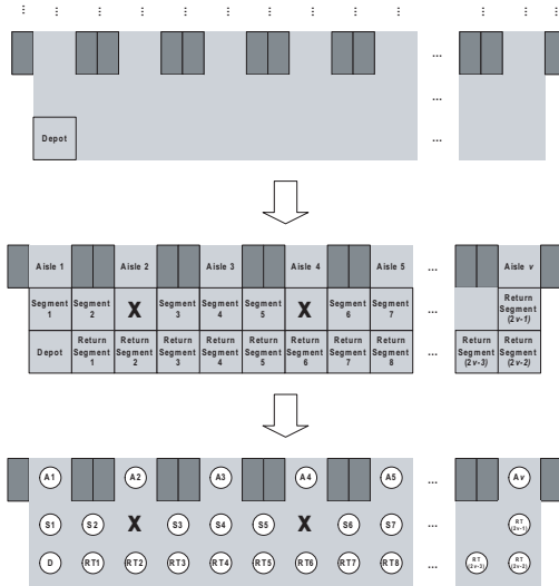
Figure 4.3: Queuing model of the lower cross aisle
