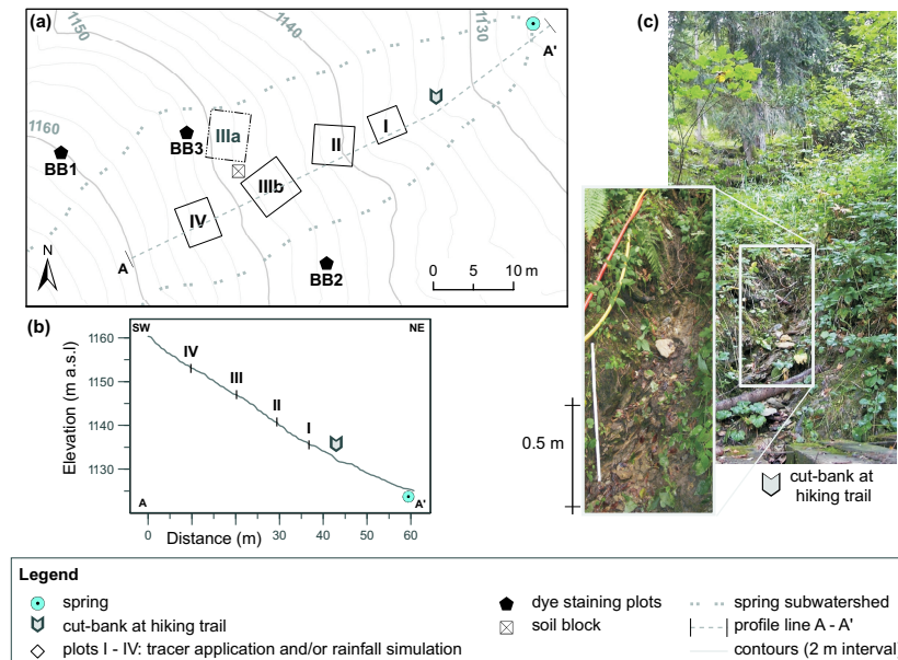
Fig. 1. (a) Map of experimental area and setup of hillslope tracer experiments. (b) Topographic cross section along A-A' in inset (a). (c) Photographs of cut-bank where a hiking trail crosses the slope and exfiltration occurs after rainfall events. Fluorescence tracers were measured in the outflow at this location and at the spring.
