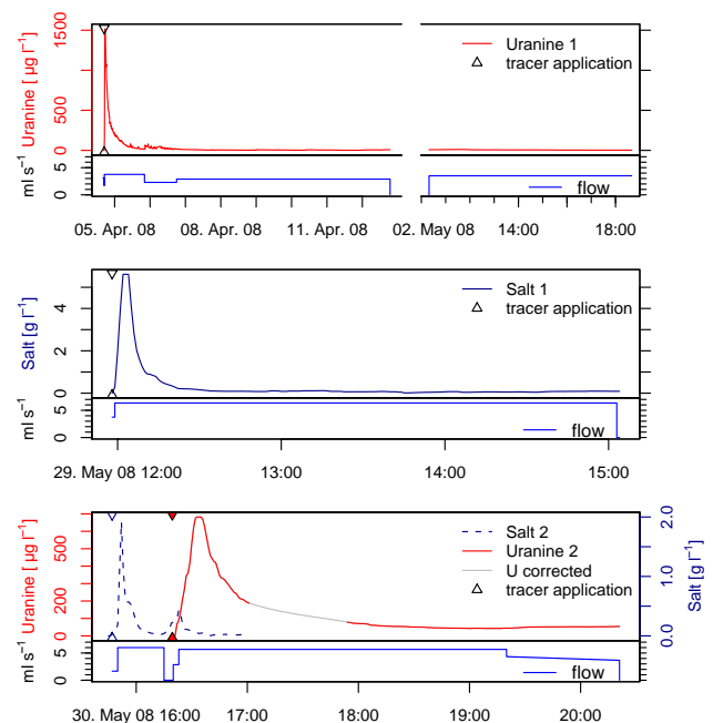
Fig. 2. Soil block experiments: tracer breakthrough curves (uranine and NaCl) and water flows of three subsequent runs (times are Central European Time). The soilblock was flushed with tracer free water before each run, and inflow was interrupted for 19 days during the first run. A gap in the second uranine BTC (lower panel) was corrected using spline interpolation for a second estimate of tracer recovery (Table 3).
