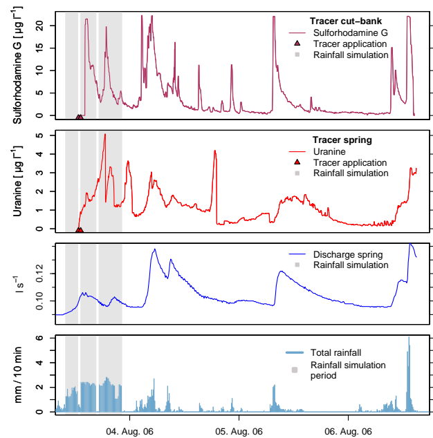
Fig. 3. First hillslope experiment under natural rainfall conditions: Tracer breakthrough curves (sulforhodamine G in outflow at cut-bank, uranine in spring discharge), spring discharge and total rainfall (from top to bottom). Grey shading marks the rainfall simulation period.
