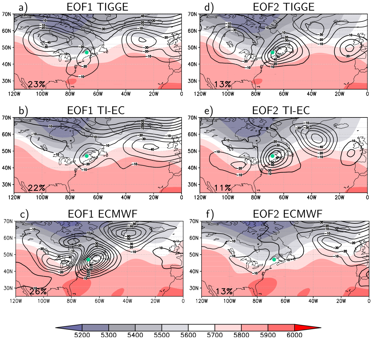
Figure 4.3: Distribution of EOF 1 (left) and EOF 2 (right)(contours, in gpm) and the ensemble mean of the geopotential height at 500 hPa (shading, in gpm) for the TIGGE (top), TI-EC (middle) and ECMWF (bottom) data set for Hurricane Ike forecast, initialised 12 UTC 10 September 2008. Investigation time given in Table 4.1. Percent of variability captured by the EOF is given in lower left corner. At this time, Hurricane Ike (green dot) is located at 45°N, 80°W in ECMWF control forecast (taken from Keller et al., 2011).
