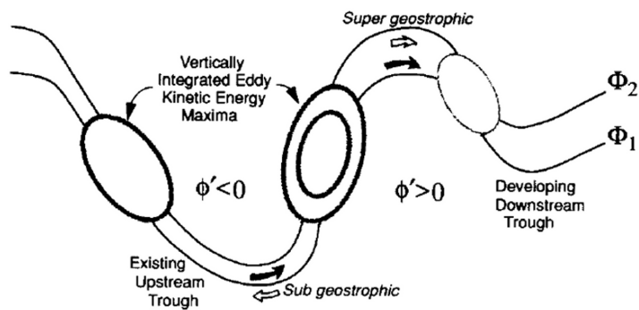
Figure 3.2: Different components of a baroclinic wave. The upper-level geopotential height field is indicated by contours, centres of enhanced vertically averaged K_e are marked as ellipses. Number of ellipses defines strength of the centre. Black arrows depict air flow relative to the wave, the ageostrophic wind is indicated by the open arrows. Eddy geopotential height is positive in the ridge and negative in the trough. Figure 2 from Orlandi and Sheldon (1995).
