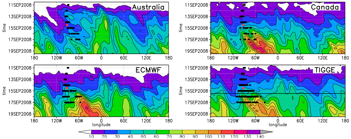
Figure 4.1: Hovmöller diagram for the standard deviation of the 500 hPa geopotential height (in gpm) in the Australian, the Canadian, the ECMWF and the TIGGE EPS for the sample case (Ike10). Surface position of Ike in all ensemble members is marked by the black dots, best track position at ET time by the red dot. Black line in TIGGE panel marks the investigation time (taken from Keller et al., 2011).
