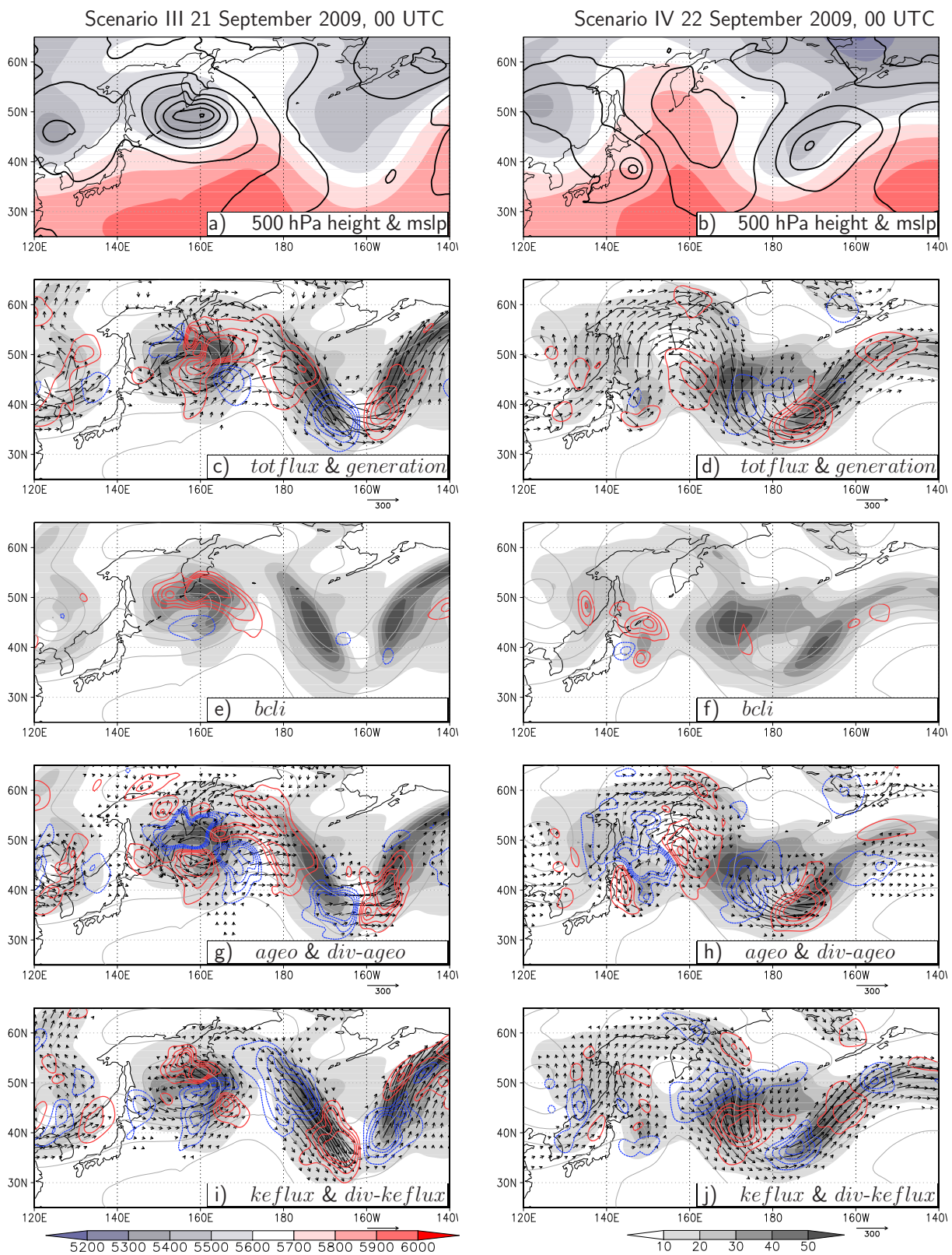
Figure 5.38: As Figure 5.35, but around the completion (III) and the onset (IV) of reintensification.
