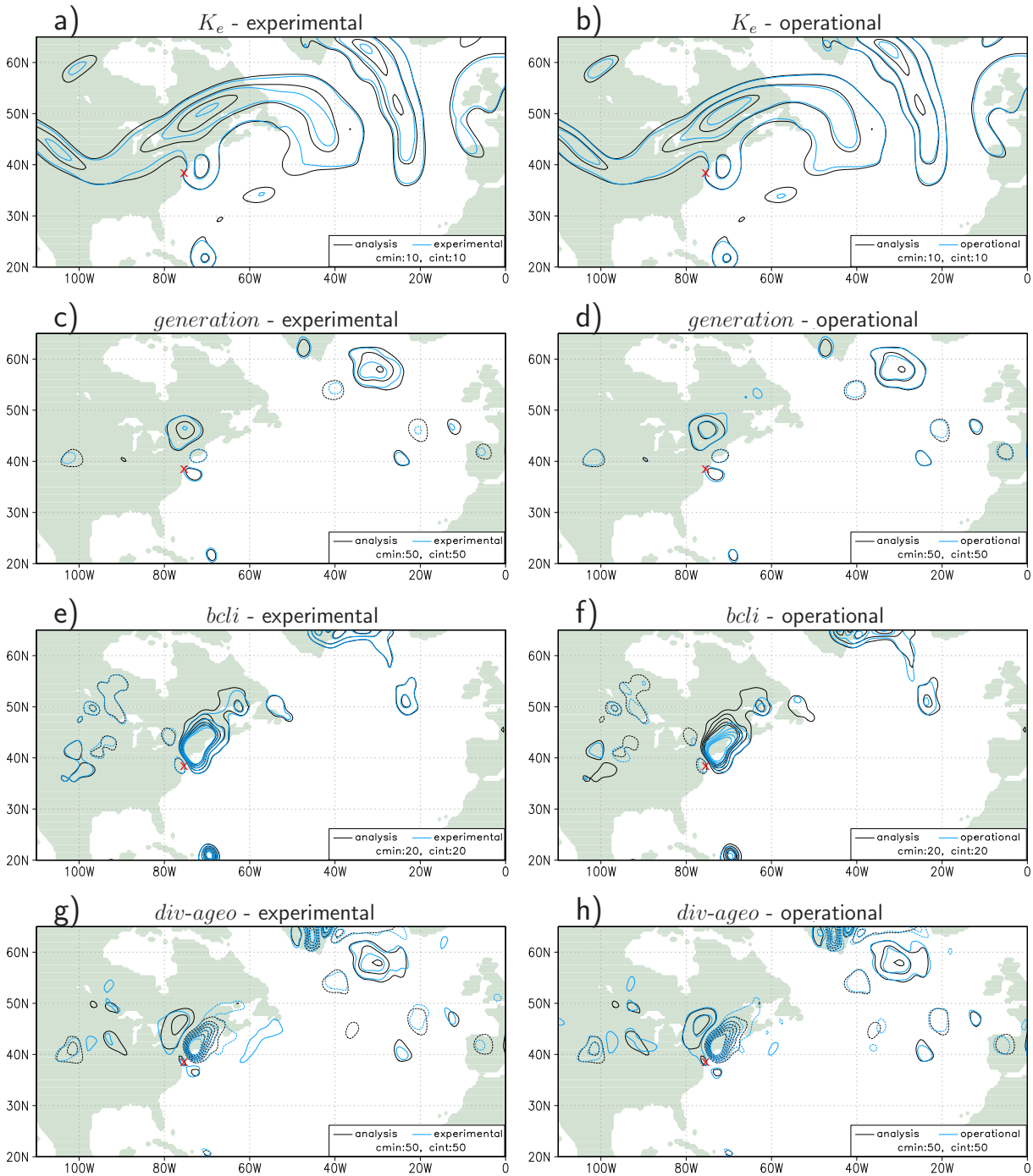
Figure 5.1: Vertically integrated eddy kinetic energy budget terms for 7 September 2008, 00 UTC in analysis output resolution (black contours, both columns), experimental EPS output resolution (blue contours, left column) and operational EPS output resolution (blue contours, right column). Surface pressure centre of Hurricane Hanna is marked by red cross. Contour intervals listed in legend, cint means contour interval, cmin stands for lowest contour plotted. a,b) eddy kinetic energy ( K_e ), c,d) total generation ( generation ), e,f) baroclinic conversion ( bcli ), g,h) ageostrophic geopotential flux convergence ( div-ageo ), i,j) convergence of K_e flux with total wind ( div-keflux ), k,l) barotropic conversion ( brtr ). K_e in 10^5 J/m^2 , budget terms in W/m^2 . Continued on next page.
