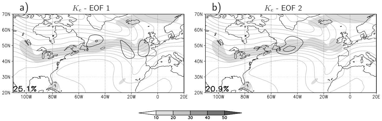
Figure 5.8: EOFs (in 3 \cdot 10^5 J/m^2 intervals, black contours) for vertically integrated ensemble mean of eddy kinetic energy (in 10^5 J/m^2 , shaded) for Hurricane Hanna at investigation time (00 UTC, 9 September 2008), ensemble mean of 500 hPa geopotential height as grey contours. a) EOF 1, b) EOF 2.
