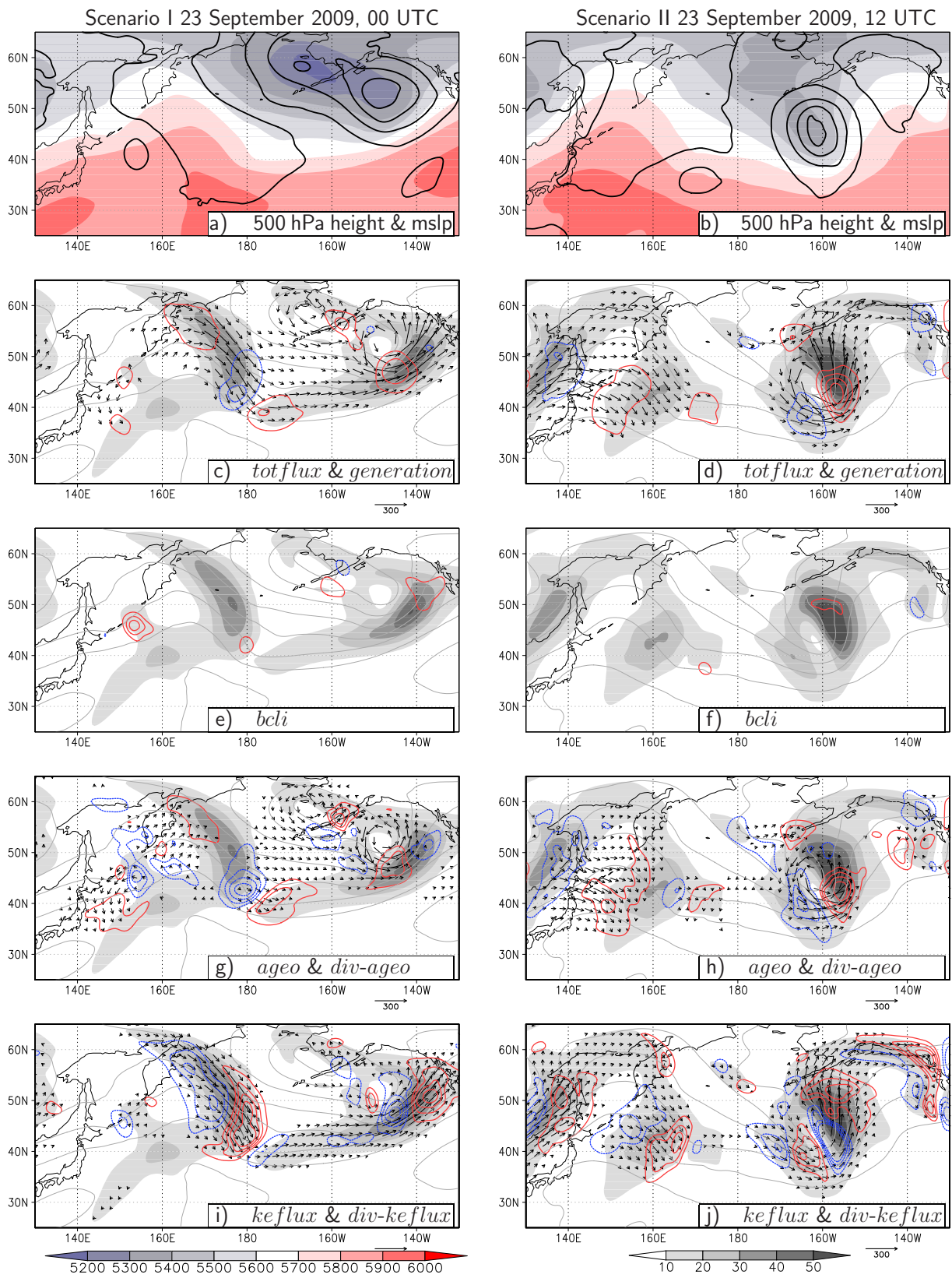
Figure 5.39: As Figure 5.35, but after completion of ET.
