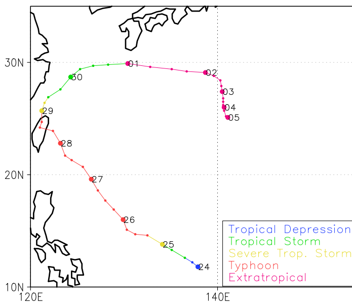
Figure 2.8: As Figure 2.7 but for Typhoon Jangmi in September-October 2008.
