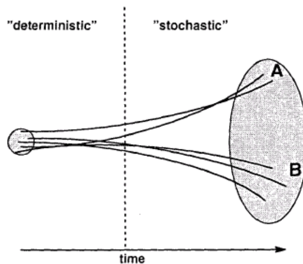
Figure 2.4: Example for an operational ensemble forecast. A representative set of perturbed initial conditions with some uncertainty distribution (circle) is advanced forward in time, indicated by the trajectories. Towards the end of the forecast the ensemble members span a range of possible solutions, represented by the ellipse. The more members point to one solution, the higher is the probability for this solution to occur. At the beginning, while the trajectories lie close to each other, the development can be considered as deterministic, thereafter it is stochastic. From Tracton and Kalnay (1993).
