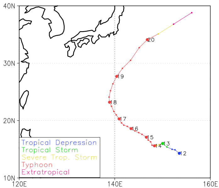
Figure 2.10: As Figure 2.7 but for Typhoon Choi-Wan in September 2009.
