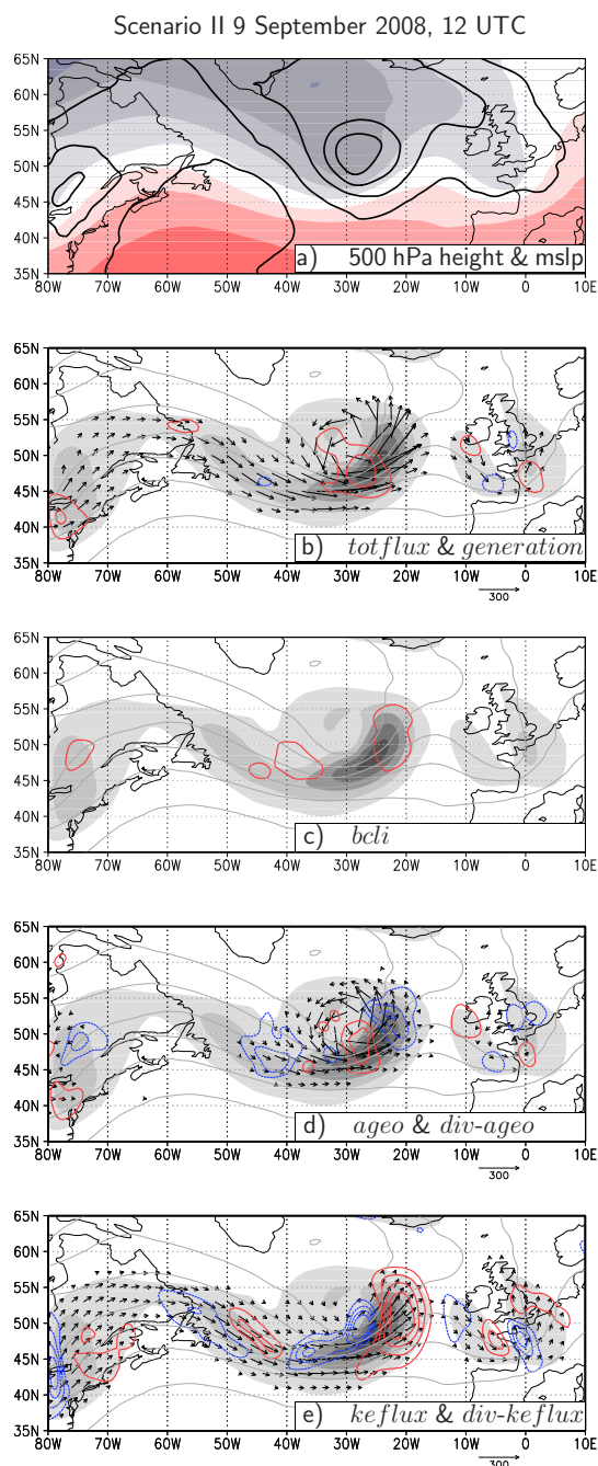
Figure 5.29: Scenario II during reintensification of Hanna. Plots as in Figure 5.27.
