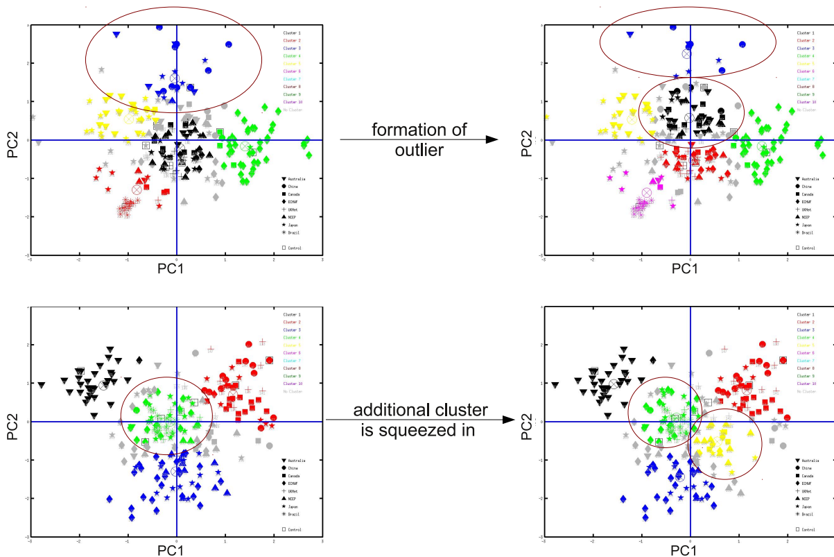
Figure 3.1: Example for undesirable cluster solutions. Top: increase of cluster number from 5 to 6 causes the additional cluster to form an outlier. Bottom: increase of cluster number from 4 to 5 leads the additional cluster to be squeezed-in between the preexisting clusters. If such a partitioning occurred, the former number of clusters (top: 4, bottom: 5) is retained.
