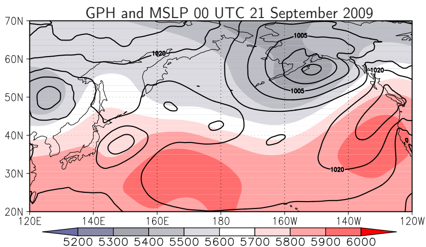
Figure 5.15: ECMWF-Ensemble mean of geopotential height at 500 hPa (in gpm ) and mean sea level pressure (in 5 hPa increments) at investigation time for EOF analysis of Typhoon Choi-Wan (00 UTC, 21 September 2009).
