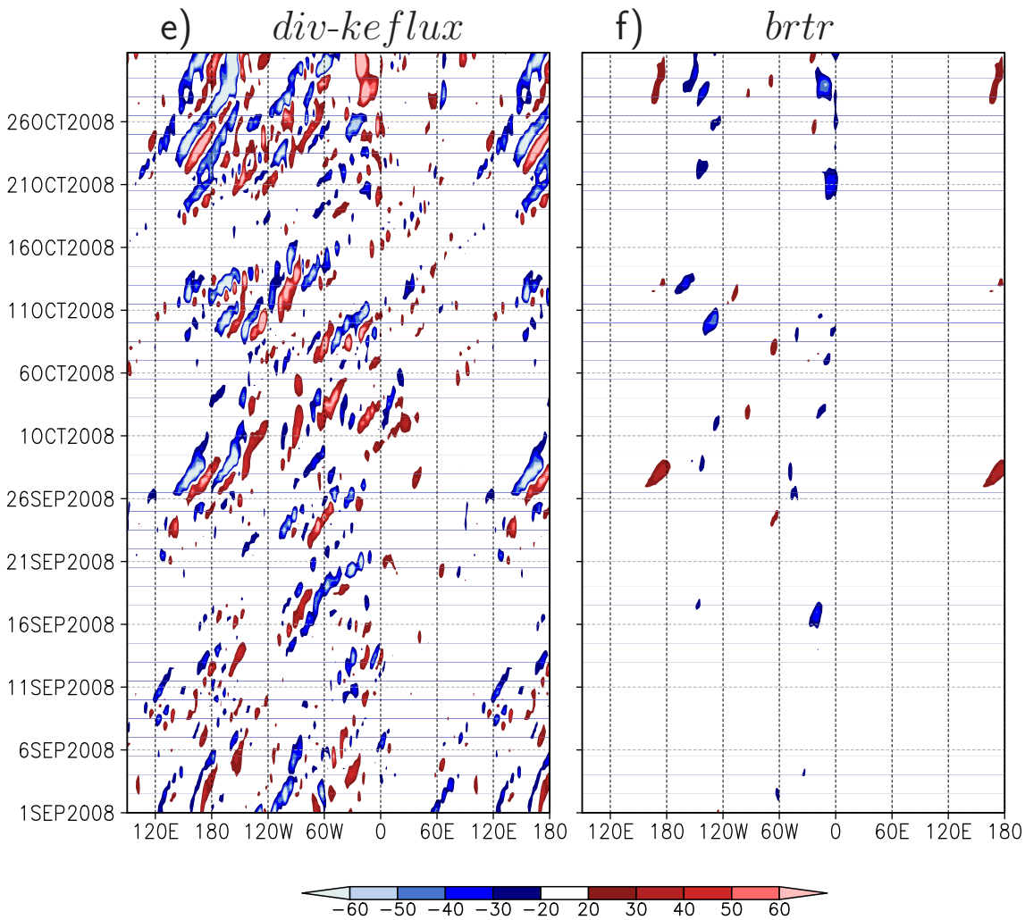
Figure 3.6: continued. e) convergence of K_e flux with the total wind ( div-keflux ) in W/m^2 , f) barotropic conversion of K_e ( brtr ) in W/m^2
