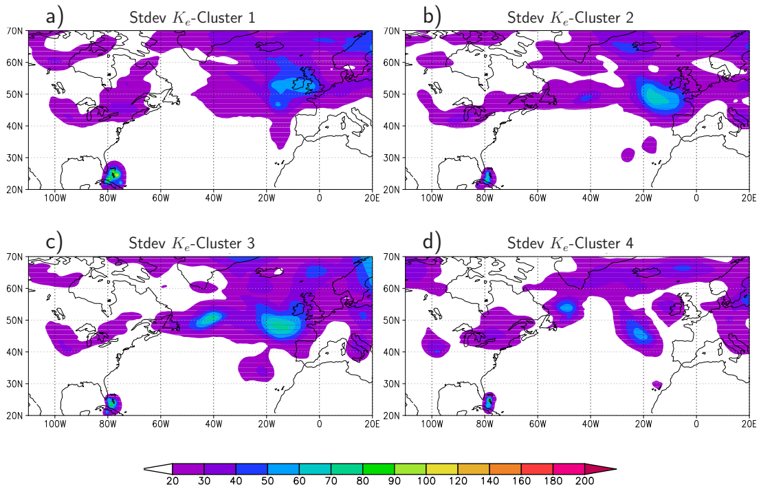
Figure 5.12: Standard deviation (in gpm ) for 500 hPa geopotential height of the K_e -clusters for Hurricane Hanna at investigation time (00 UTC, 09 September 2008). a) K_e -cluster 1, b) K_e -cluster 2, c) K_e -cluster 3, d) K_e -cluster 4.
