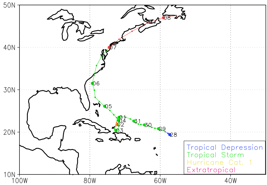
Figure 2.5: Track for Hurricane Hanna in August-September 2008. Dots mark the position of Hurricane Hanna every 6 hours. Large dots describe position at 00 UTC of the indicated day (number). Intensity in colours, as given in legend. Based on best track data from the HURDAT-archive from the National Hurricane Centre ( www.nhc.noaa.gov/pastall.shtml#hurdat ). ET positions from "Historical Hurricane Tracks" from the National Oceanic Atmospheric Administration (NOAA, http://www.csc.noaa.gov/hurricanes/# ).
