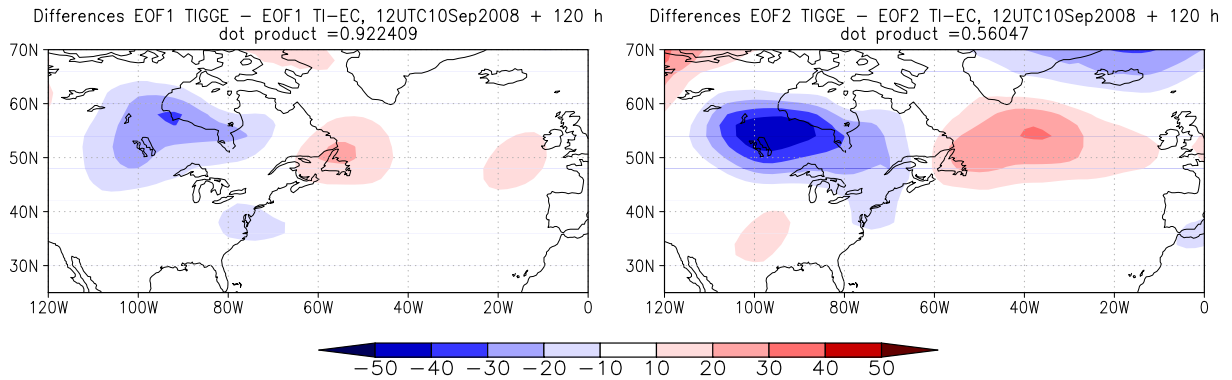
Figure 4.5: Differences between EOF 1 (left) and EOF 2 (right) in the TIGGE and TI-EC data set for the sample case (taken from Keller et al., 2011).
