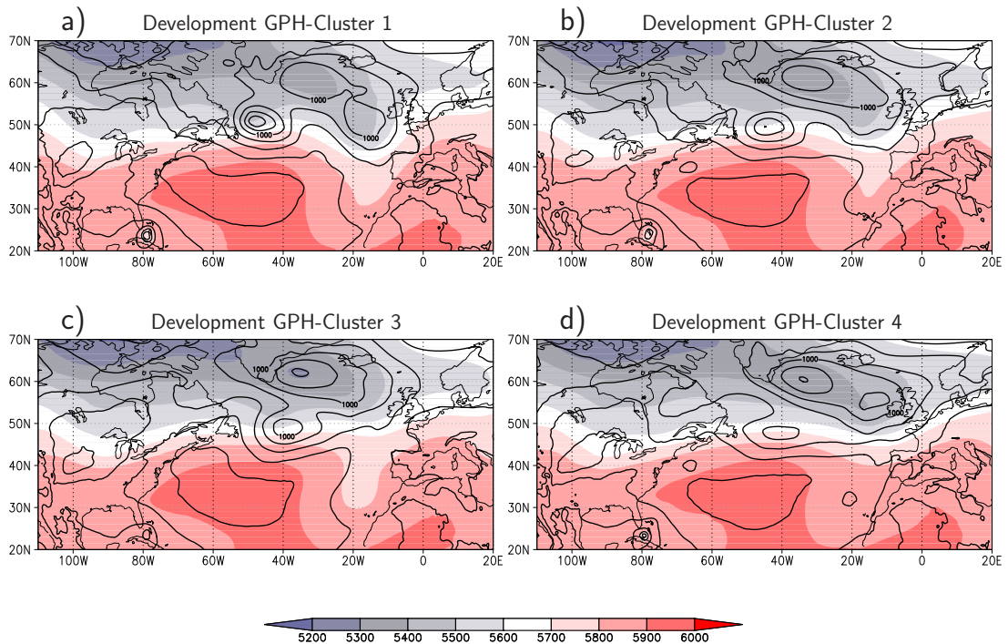
Figure 5.11: Cluster mean for 500 hPa geopotential height (in gpm ) and mean sea level pressure (in 5hPa increments) of the GPH-clusters for Hurricane Hanna at investigation time (00 UTC, 09 September 2008). a) GPH-cluster 1, b) GPH-cluster 2, c) GPH-cluster 3, d) GPH-cluster 4.
