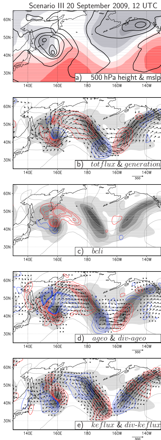
Figure 5.36: Scenario III during the merger between Choi-Wan and the extratropical cyclone. Plots as in Figure 5.35.
