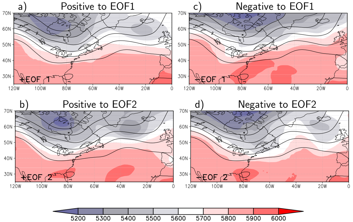
Figure 4.4: Geopotential height at 500 hPa (shaded, in gpm) for several TIGGE members and for the ensemble mean (contour). The members contribute a) positive to EOF 1, b) positive to EOF 2, c) negative to EOF 1, d) negative to EOF 2. Contribution to the other EOF, respectively, is rather neutral.
