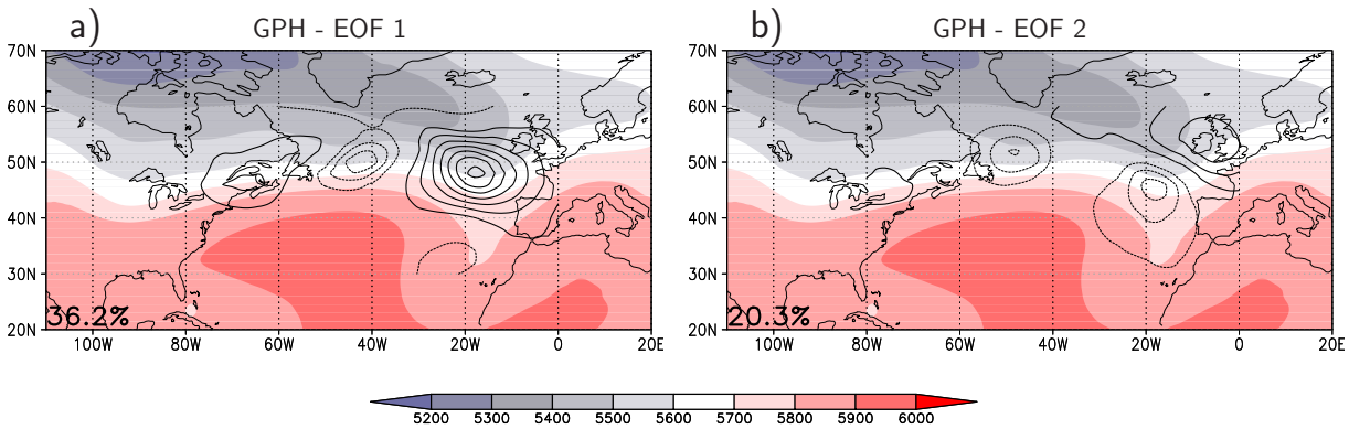
Figure 5.6: EOFs (in 10 gpm intervals, contours) for 500 hPa geopotential height (in gpm , shaded) for Hurricane Hanna at investigation time (00 UTC, 09 September 2008). a) EOF 1, b) EOF 2, captured amount of total variability at bottom left.
