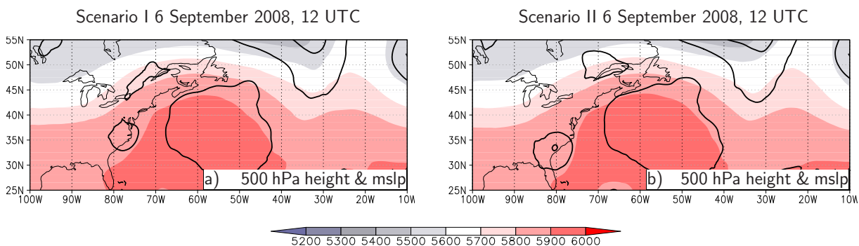
Figure 5.26: Scenario I (left) and II (right) 36 h after initialisation (6 September 2008, 12 UTC). Geopotential height (shaded, in gpm) and mslp (contours). Remnants of Hanna are embedded in the closed mslp contour near the US East Coast.
