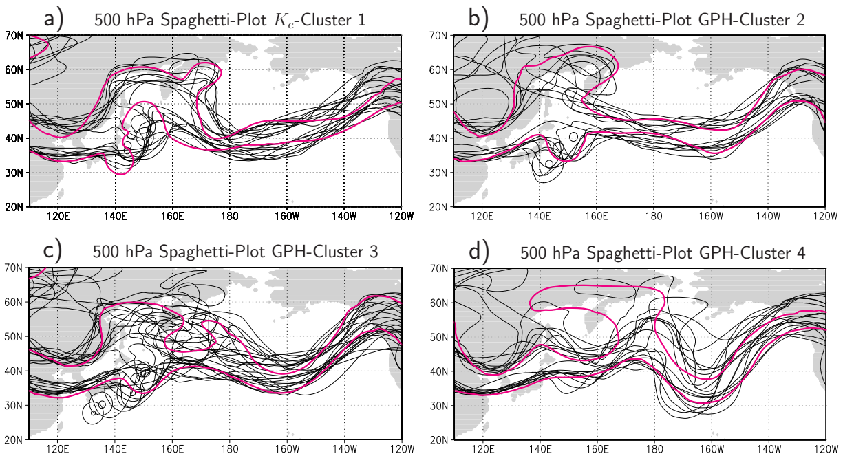
Figure 5.32: Spaghetti-Plot for 5600 and 5800 gpm height isolines at investigation time for all ensemble members, assigned to K_e -Cluster 1 (a), GPH-Cluster 2 (b), GPH-Cluster 3 (c) and GPH-Cluster 4 (d) for Choi-Wan.
