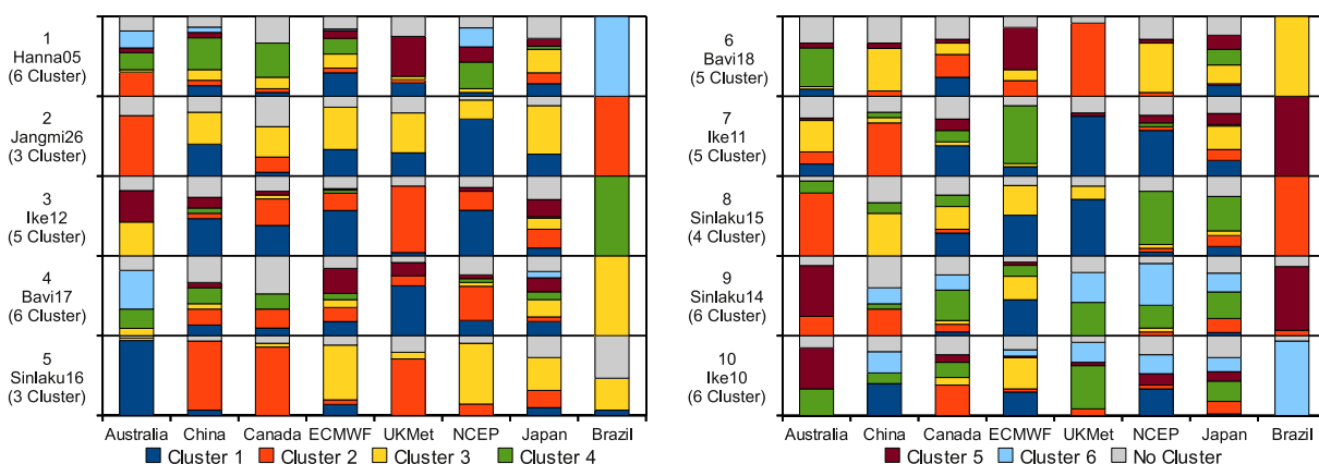
Figure 4.7: As Figure 4.6 but for all ten cases. The bottom right panel (Ike10) is reproduced from 4.6 for completeness (taken from Keller et al., 2011).
