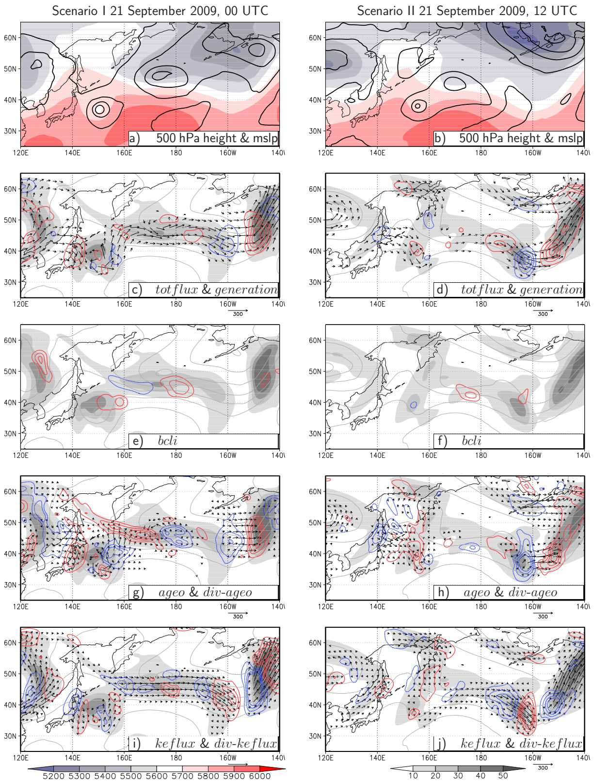
Figure 5.37: As Figure 5.34, but around the onset reintensification.
