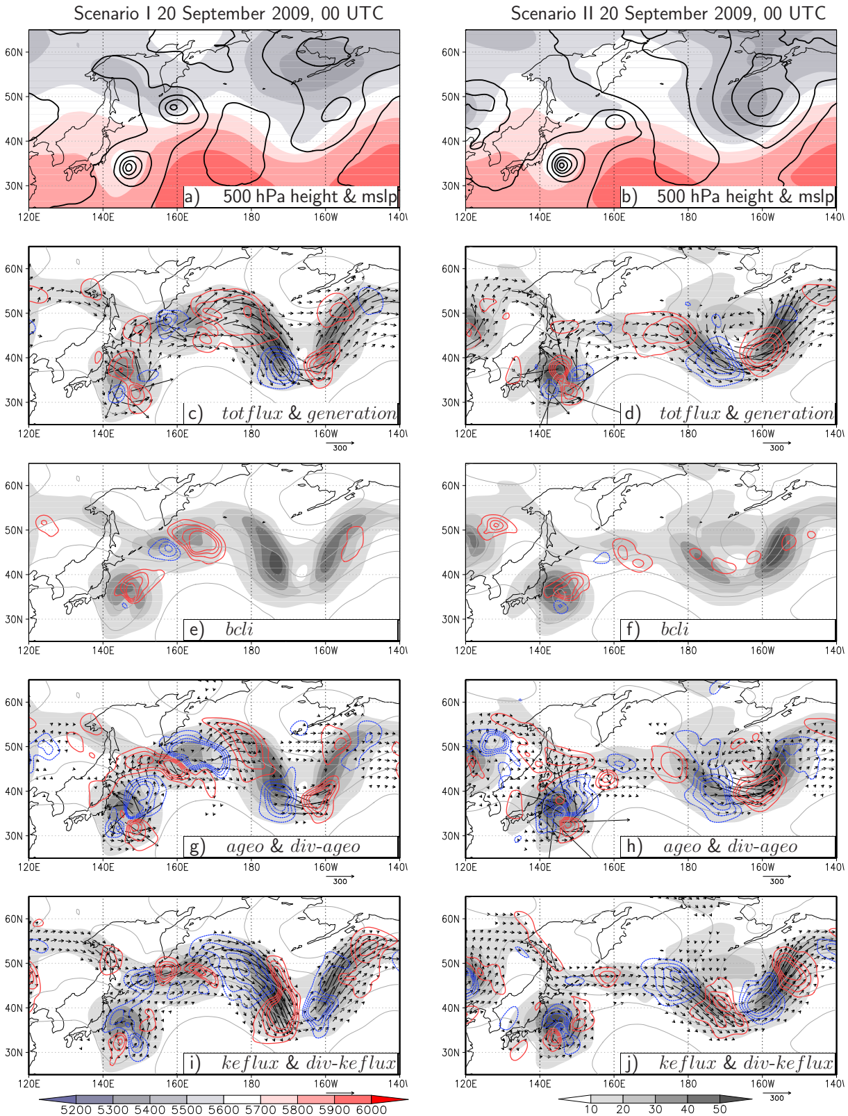
Figure 5.34: Scenario I (left) and II (right) at the onset of interaction between Choi-Wan and the mid-latitude flow. a, b) 500 hPa geopotential height (shaded, in gpm) and mslp (contours, in 5 hPa increments); c, d) K_e (shaded, for all in 10^5 J/m^2 ), tot flux (arrows, for all in 10^6 W/m , larger than 40 \cdot 10^6 W/m ) and generation (contours, for all in W/m^2 ); e, f) K_e (shaded) and bcli (contours); g, h) K_e (shaded), ageo (arrows, larger than 20 \cdot 10^6 W/m ) and div-ageo (contours); i, j) K_e (shaded), keflux (arrows, larger than 20 \cdot 10^6 W/m ) and div-keflux (contours). Contour interval 50 W/m^2 , starting with 50 W/m^2 for all plots at each time, blue: divergence/loss of K_e , red: convergence/gain of K_e . See Table 3.1 for abbreviations.
