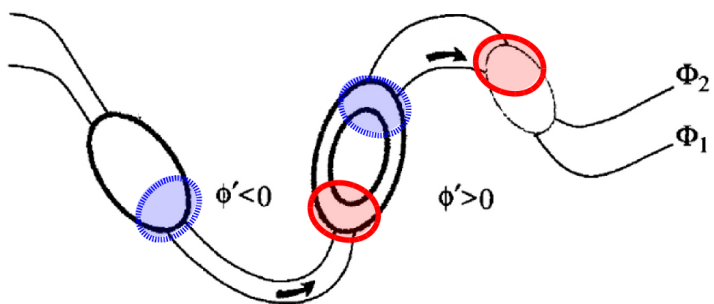
Figure 3.3: Schematic illustration for the ageostrophic geopotential flux and its divergence and convergence. Flow structure and K_e centres as in Figure 3.2. Convergence of div-ageo in red, divergence in blue.
