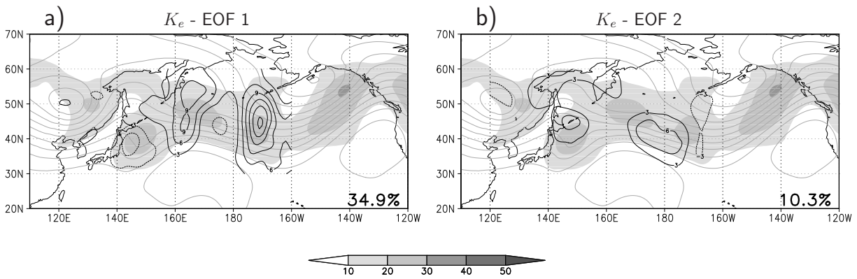
Figure 5.18: EOFs (in 3 \cdot 10^5 J/m^2 intervals, black contours) for vertically integrated ensemble mean of eddy kinetic energy (in 10^5 J/m^2 , shaded) for Typhoon Choi-Wan at investigation time (00 UTC, 21 September 2009), ensemble mean for 500 hPa geopotential heights as grey contours. a) EOF 1, b) EOF 2, amount of total variability captured is given at bottom right.
