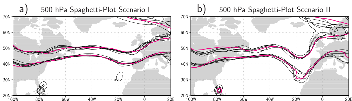
Figure 5.24: Spaghetti-Plot for 5600 and 5800 gpm height isolines at investigation time (9 September 2008, 00 UTC) for all ensemble members, assigned to GPH-Cluster 1 (a) and GPH-Cluster 4 (b) for Hanna.
