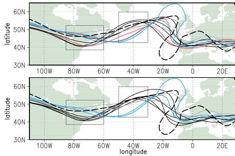
Figure 4.8: Different development scenarios for Ike10, 48 h after investigation time (12 UTC 17 September 08, verifying analysis dashed). Spaghetti plots of the 570 gpm isoline cluster means. Top: TIGGE (3 black, 2 red) and ECMWF (blue), bottom: TI-EC (black) and ECMWF (as above). Colours to highlight scenarios mentioned in text. Boxes discussed in text (taken from Keller et al., 2011).
