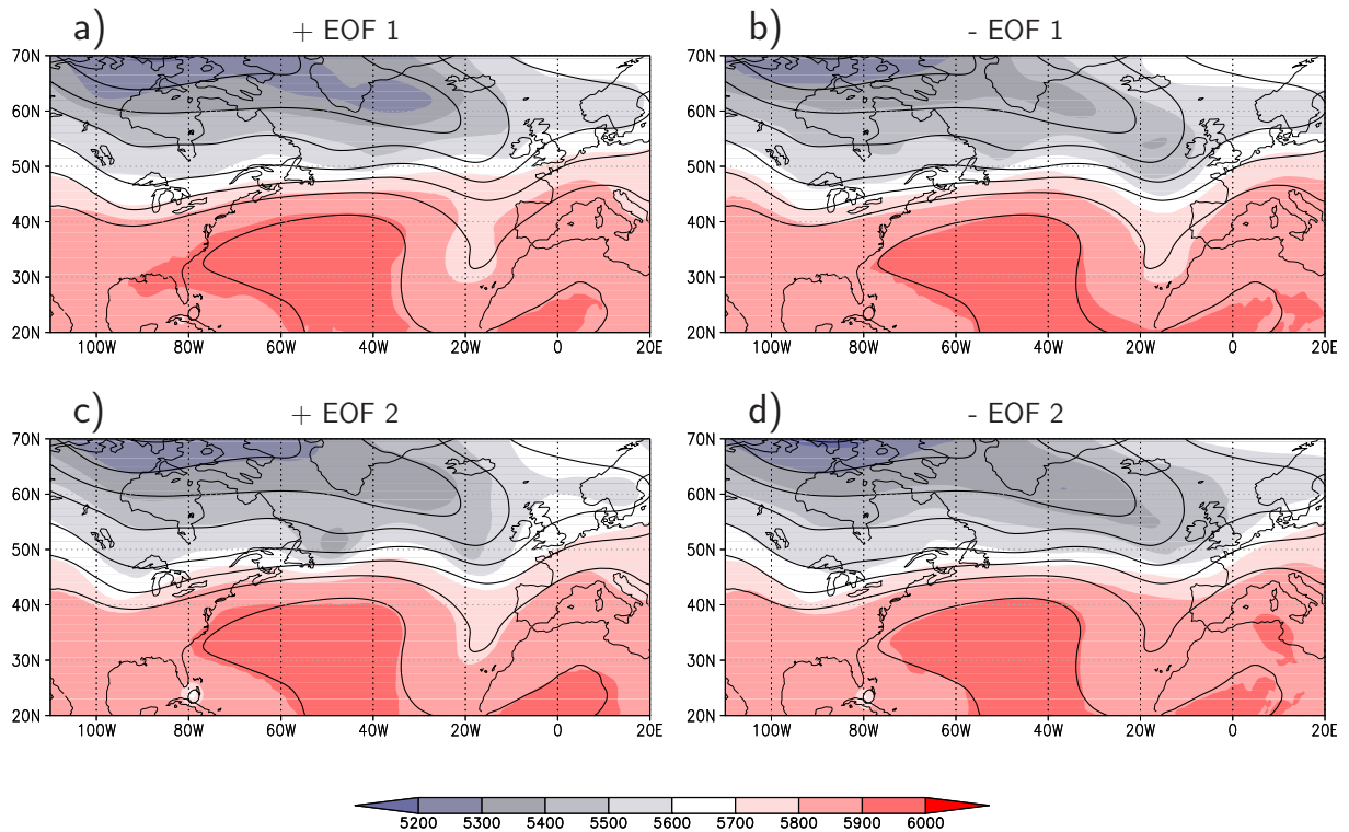
Figure 5.7: 500 hPa geopotential height (shaded, in gpm ) and ensemble mean for 500 hPa geopotential height (contours, in gpm ) for ensemble members with distinct contributions to the EOF patterns for Hurricane Hanna at investigation time (00 UTC, 09 September 2008). a) Member with positive contribution to EOF 1 and neutral to EOF 2, b) Member with negative contribution to EOF 1 and neutral to EOF 2, c) Member with positive contribution to EOF 2 and neutral to EOF 1, d) Member with negative contribution to EOF 2 and neutral to EOF 1.
