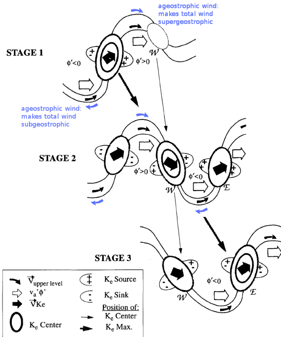
Figure 3.5: Schematic illustration of downstream baroclinic development (with slight modifications reproduced from Orlandi and Sheldon, 1995). In the three stage process the upstream maximum (ellipse) decays, while the downstream centres \mathcal{W} and \mathcal{E} gain K_e (+/- signs) due to convergence of the ageostrophic geopotential flux (open arrow). The ageostrophic geopotential flux always points downstream due to sub- or super-geostrophic total winds (blue arrows) and positive or negative geopotential anomalies in the troughs and ridges, respectively. The K_e maximum propagate with group velocity (long thick arrow), a single K_e centre, on the other hand, propagates with phase velocity (long thin arrow)
