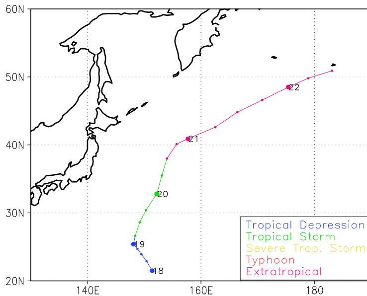
Figure 2.9: As Figure 2.7 but for Tropical Storm Bavi in October 2008.
