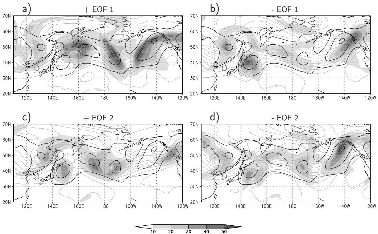
Figure 5.19: Vertically integrated K_e (shaded, in 10^5 J/m^2 ) and ensemble mean for K_e (contours, in 10^5 J/m^2 , starting with 10 \cdot 10^5 J/m^2 , interval 10 \cdot 10^5 J/m^2 ) with distinct contributions to the EOF patterns for Typhoon Choi-Wan at investigation time (00 UTC, 21 September 2009). a) Member with positive contribution to EOF 1 and neutral to EOF 2, b) Member with negative contribution to EOF 1 and neutral to EOF 2, c) Member with positive contribution to EOF 2 and neutral to EOF 1, d) Member with negative contribution to EOF 2 and neutral to EOF 1.
