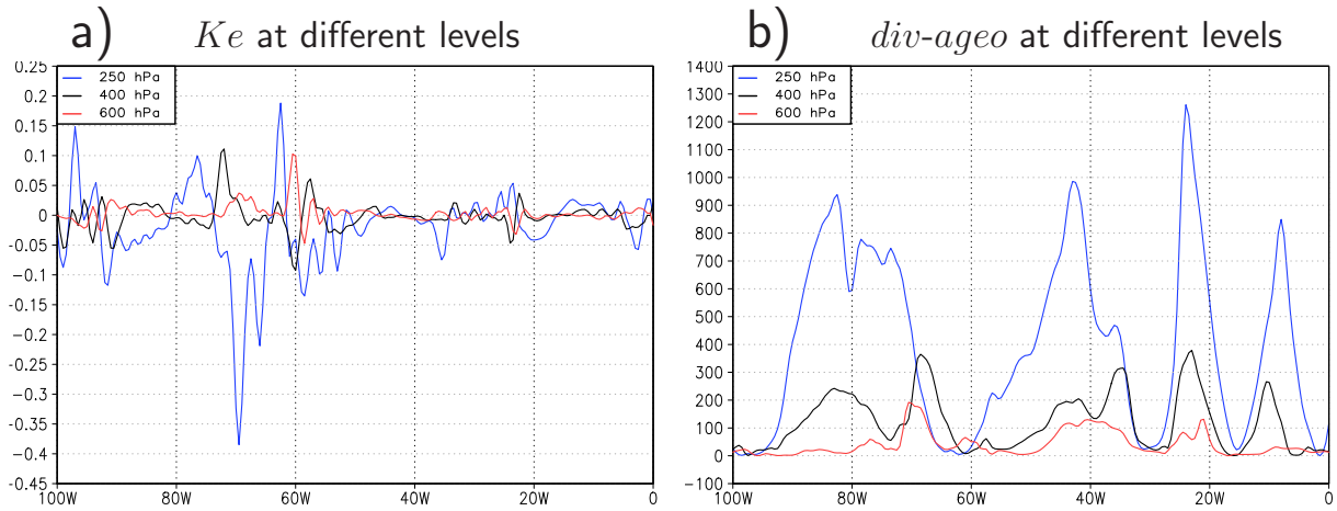
Figure 5.2: Magnitudes for a) K_e and b) div-ageo for lat=45^\circ N at 7 September 2008, 00 UTC at 250 hPa (blue), 400 hPa (black) and 600 hPa (red) from the analysis data set.
