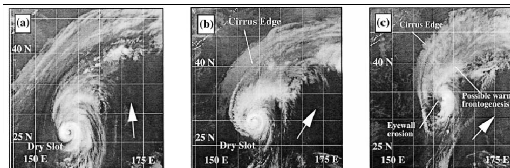
Figure 2.2: Satellite images for the ET of Super-Typhoon Ginger in 1997 indicating the structural changes during ET, as described in the conceptual model. a) 03 UTC 28 Sep, b) 00 UTC 29 September and c) 12 UTC 29 September 1997. Regions of interest are marked. White arrow indicates translation of the storm. Part of Figure 4 from Klein et al. (2000).
