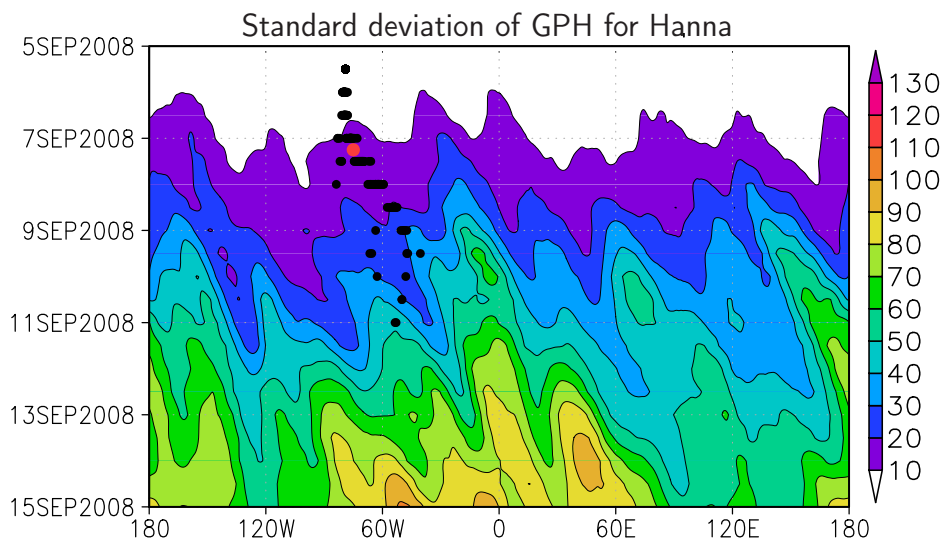
Figure 5.4: Hovmöller diagram for standard deviation of 500 hPa geopotential height (shaded, in gpm ) in the ensemble forecast for Hanna, initialised 00 UTC, 5 September 2008. Black dots mark surface position of Hanna in the individual ensemble members, red dot marks its best track position as it was declared as extratropical system by the RMSC
