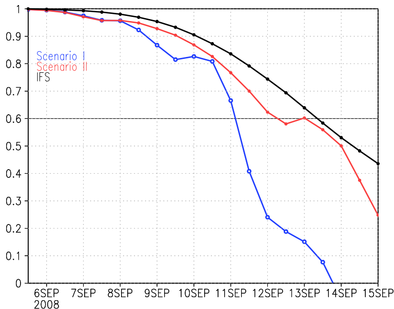
Figure 5.25: Anomaly Correlation Coefficient for the two members of the experimental ECMWF EPS forecast, the ECMWF analysis and the ERA-Interim climatology for the 500 hPa geopotential field between 30-70°N and 250-380°W for scenario I (blue) and scenario II (red). General forecast accuracy of the operational deterministic ECMWF forecast is highlighted in black. Forecast was initialised on 00 UTC, 5 September 2008. Thanks to Christian Grams for providing the ACC-Grads-Script.
