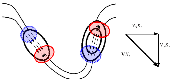
Figure 3.4: Schematic illustration for the flux of K_e with the total wind (arrows) and its divergence and convergence. Flow structure and K_e centres as in Figure 3.2. Convergence of div-keflux in red, divergence in blue. The flux component can be separated into a zonal (x) and meridional (y) component, highlighting the propagation of the K_e centre.
