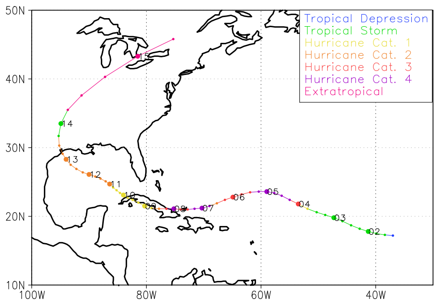
Figure 2.6: As Figure 2.5 but for Hurricane Ike in September 2008.
