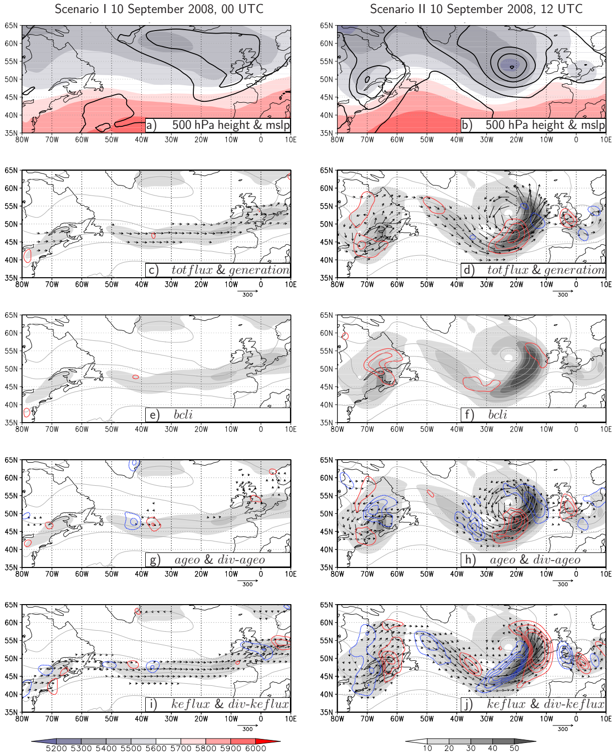
Figure 5.30: As Figure 5.27, but after completion of reintensification in scenario II.
