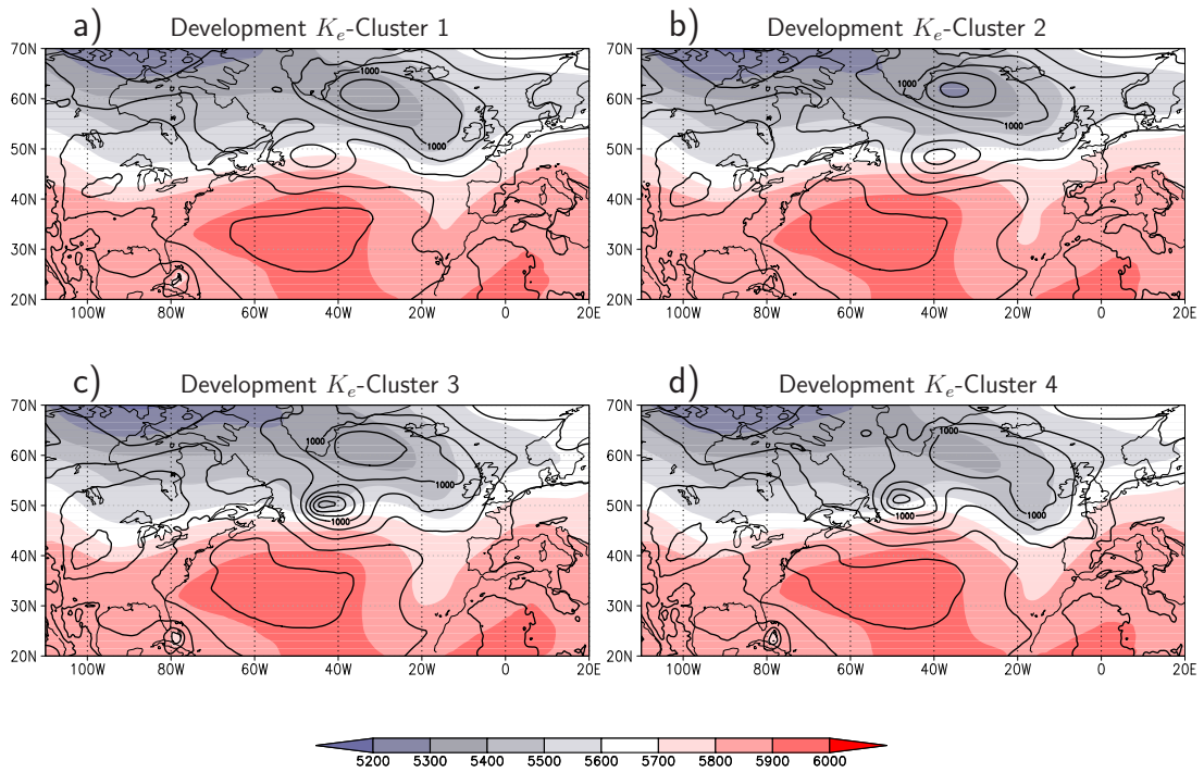
Figure 5.13: Cluster mean for 500 hPa geopotential height (in gpm ) and mean sea level pressure (in 5hPa increments) of the K_e -clusters for Hurricane Hanna at investigation time (00 UTC, 09 September 2008). a) K_e -cluster 1, b) K_e -cluster 2, c) K_e -cluster 3, d) K_e -cluster 4.
