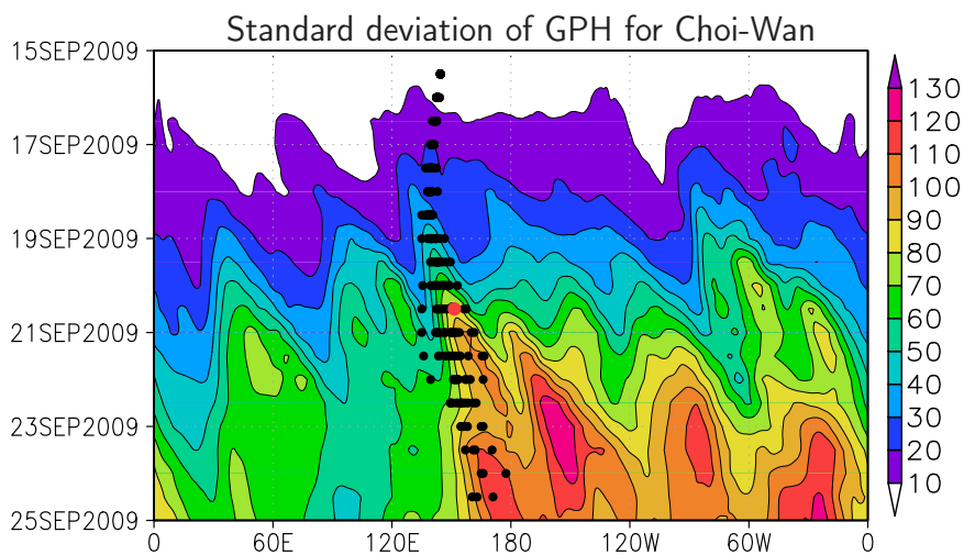
Figure 5.14: Hovmöller diagram for standard deviation of 500 hPa geopotential height (shaded, in gpm ) in the ensemble forecast for Choi-Wan, initialised 00 UTC, 15 September 2009. Black dots mark surface position of Choi-Wan in the individual ensemble members, red dot marks its best track position as it was declared as extratropical system by the RMSC.
