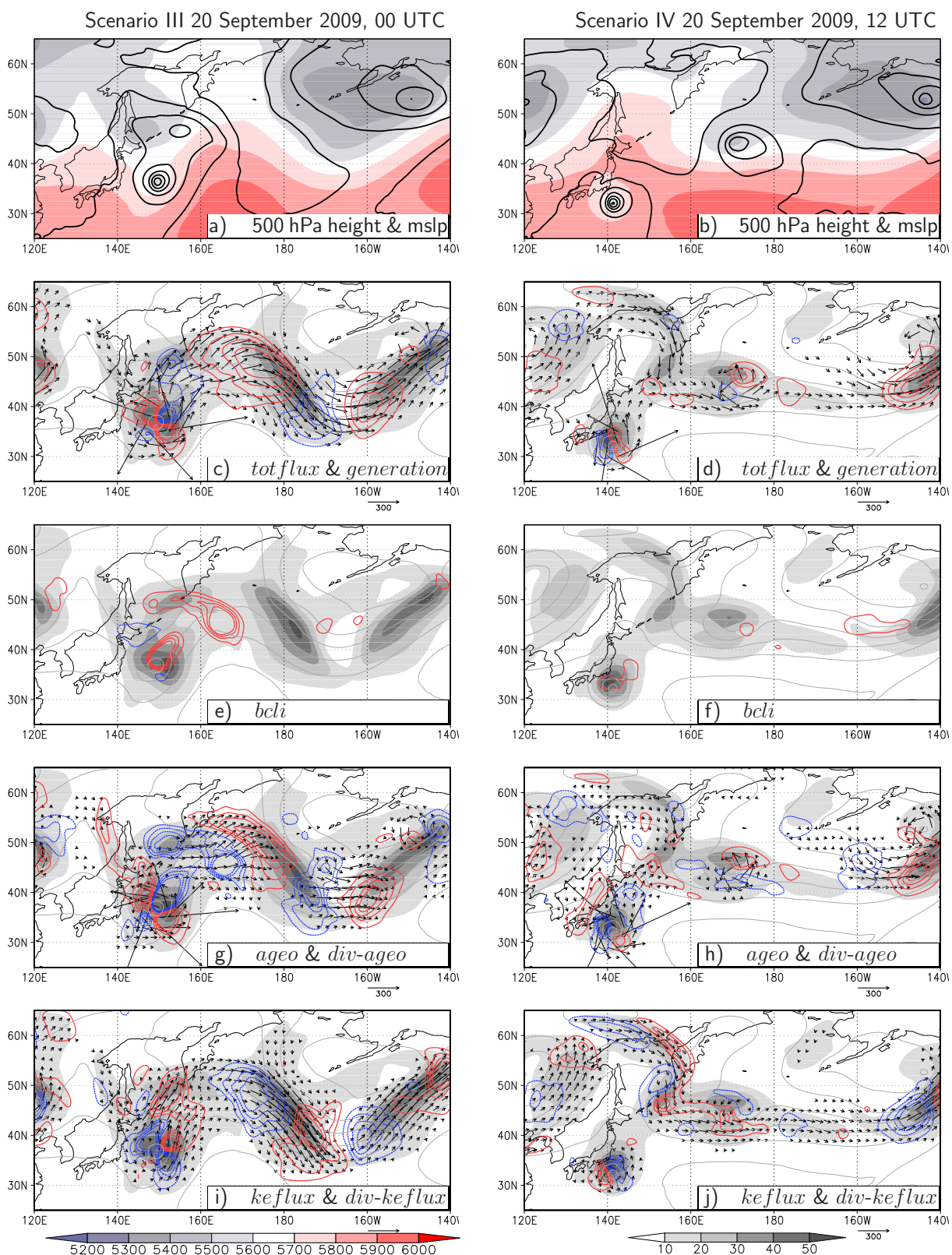
Figure 5.35: Scenario III (left) and IV (right) at the onset of interaction between Choi-Wan and the mid-latitude flow. a, b) 500 hPa geopotential height (shaded, in gpm) and mslp (contours, in 5 hPa increments); c, d) K_e (shaded, for all in 10^5 J/m^2 ), totflux (arrows, for all in 10^6 W/m , larger than 40 \cdot 10^6 W/m ) and generation (contours, for all in W/m^2 ); e, f) K_e (shaded) and bcli (contours); g, h) K_e (shaded), ageo (arrows, larger than 20 \cdot 10^6 W/m ) and div-ageo (contours); i, j) K_e (shaded), keflux (arrows, larger than 20 \cdot 10^6 W/m ) and div-keflux (contours). Contour interval 50 W/m^2 , starting with 50 W/m^2 for all plots at each time, blue: divergence/loss of K_e , red: convergence/gain of K_e . See Table 3.1 for abbreviations.
