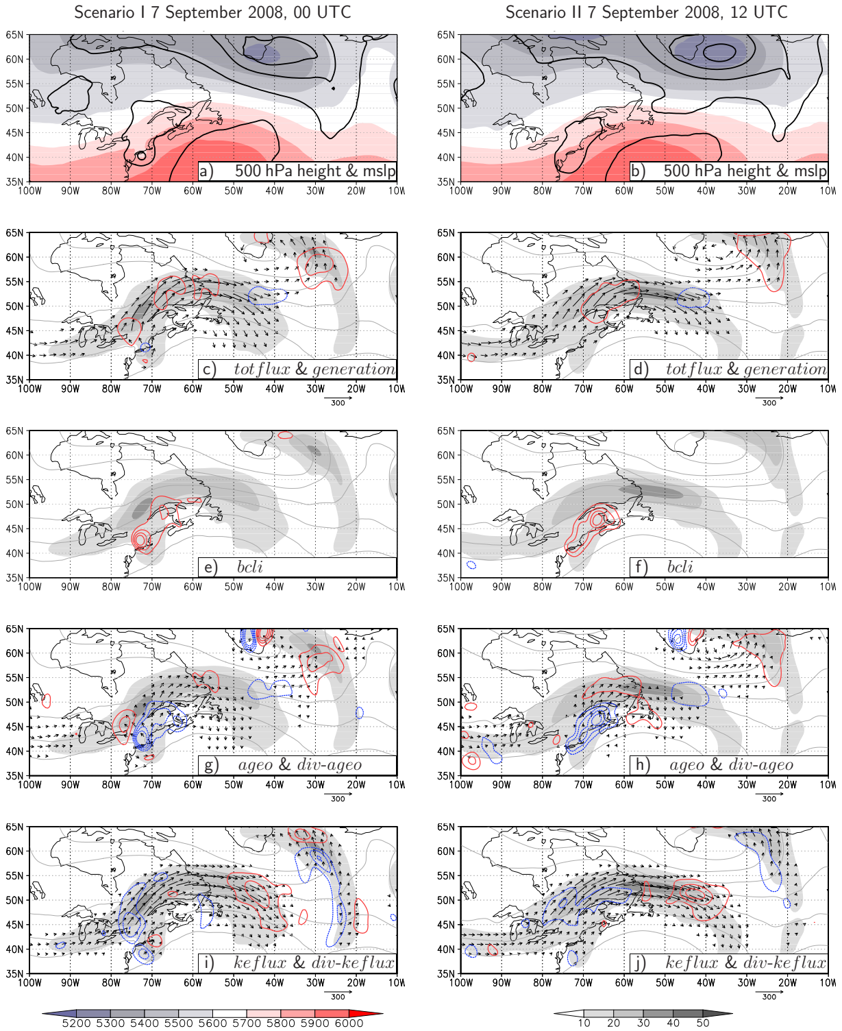
Figure 5.27: Scenario I (left) and II (right) at the onset of interaction between Hanna and the mid-latitude flow. a, b) 500 hPa geopotential height at 500 hPa (shaded, in gpm) and mslp (contours, in 5 hPa increments); c, d) K_e (shaded, for all in 10^5 J/m^2 ), totflux (arrows, for all in 10^6 W/m , larger than 40 \cdot 10^6 W/m ) and generation (contours, for all in W/m^2 ); e, f) K_e (shaded) and bcli (contours); g, h) K_e (shaded), ageo (arrows, larger than 20 \cdot 10^6 W/m ) and div-ageo (contours); i, j) K_e (shaded), keflux (arrows, larger than 20 \cdot 10^6 W/m ) and div-keflux (contours). Contour interval 50 W/m^2 , starting with 50 W/m^2 for all plots at each time, blue: divergence/loss of K_e , red: convergence/gain of K_e . See Table 3.1 for abbreviations.
