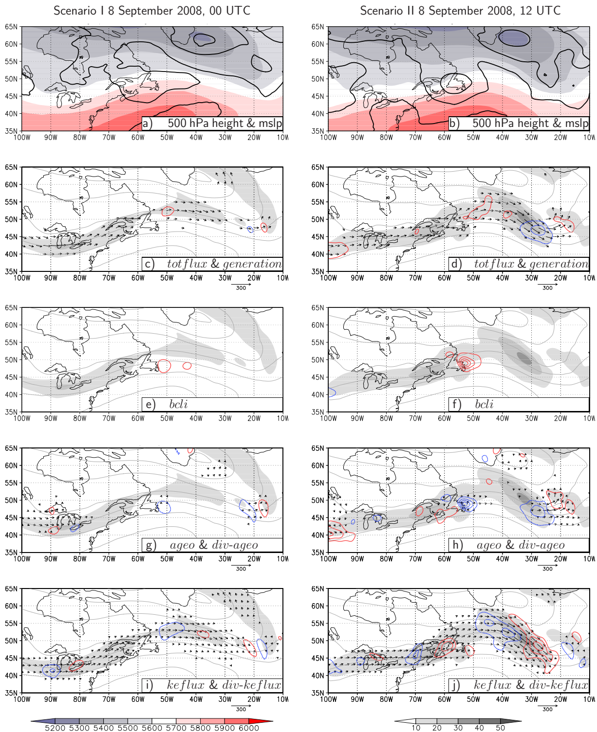
Figure 5.28: As Figure 5.27, but for the onset of reintensification in scenario II.
