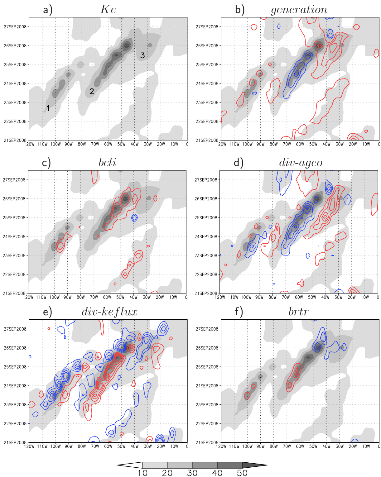
Figure 3.7: Sections of Hovmöller diagram for a specific K_e signal. K_e in shading, different source and sink terms in contours (red=gain, convergence, blue=loss, divergence): a) eddy kinetic energy K_e , b) total generation of K_e ( generation ), c) baroclinic conversion ( bcli ), d) convergence (positive) of the ageostrophic geopotential flux ( div-ageo ), e) convergence (positive) of K_e flux with total wind ( div-keflux ) and f) barotropic conversion ( brtr ). K_e in 10^5 \text{ J/m}^2 , budget terms in \text{W/m}^2 .
