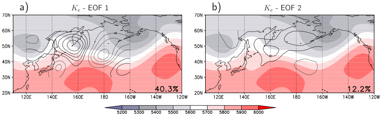
Figure 5.16: EOFs (in 10 gpm intervals, contours) for 500 hPa geopotential height (in gpm , shaded) for Typhoon Choi-Wan at investigation time (00 UTC, 21 September 2009). a) EOF 1, b) EOF 2, captured amount of total variability at bottom right.
