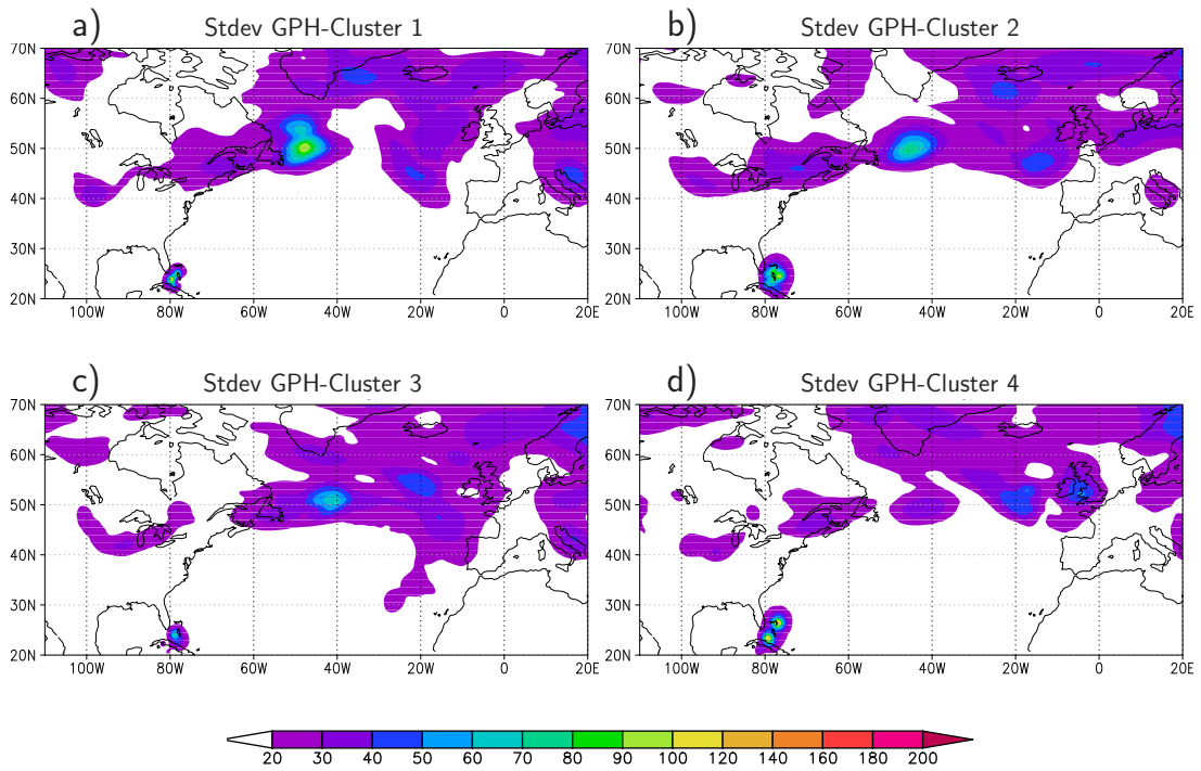
Figure 5.10: Standard deviation (in gpm ) for 500 hPa geopotential height of the GPH-clusters for Hurricane Hanna at investigation time (00 UTC, 09 September 2008). a) GPH-cluster 1, b) GPH-cluster 2, c) GPH-cluster 3, d) GPH-cluster 4.
