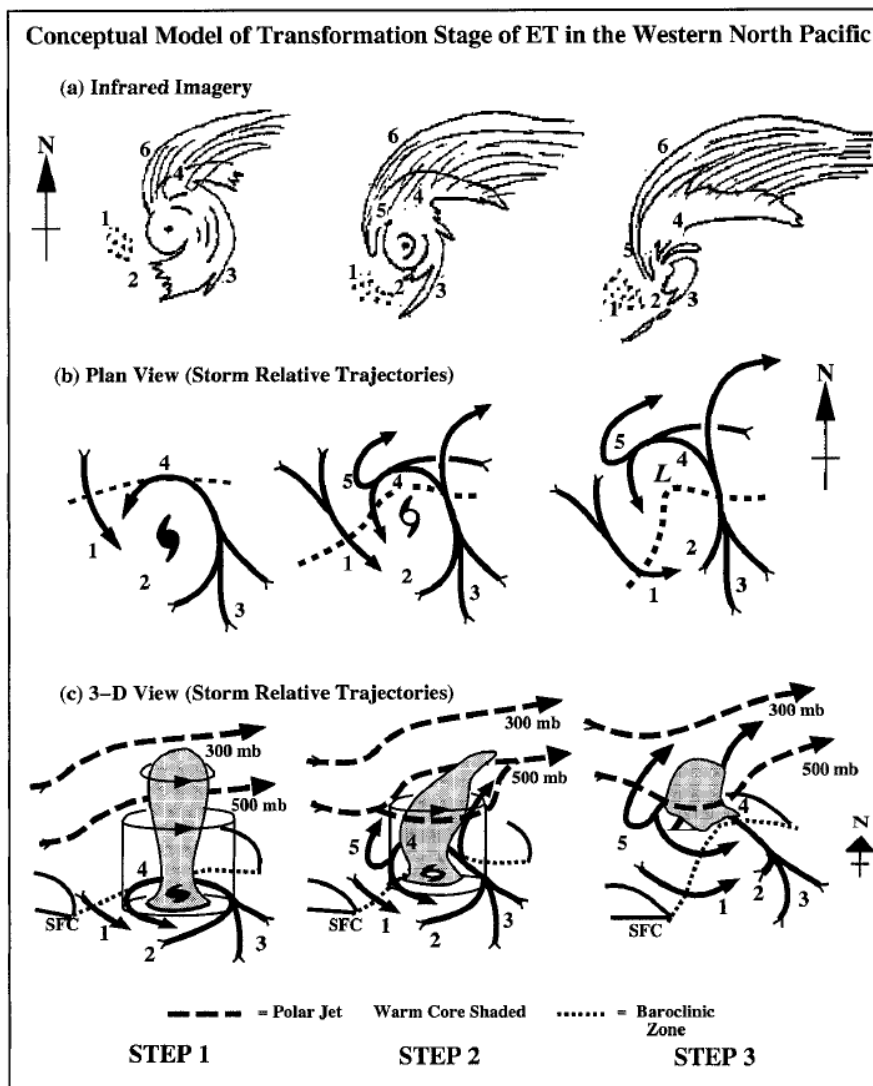
Figure 2.1: Conceptual model of Klein et al. (2000) for the three steps of the transformation stage during ET in the western North Pacific, based on examination of satellite images. a) schematic IR-imagery, b) schematic circulation pattern, c) schematic 3-d circulation. Numbers highlight different regions discussed in text. Figure 5 from Klein et al. (2000).
