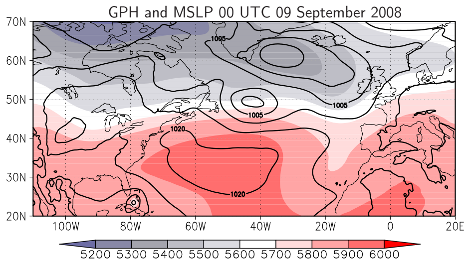
Figure 5.5: ECMWF ensemble mean of geopotential height at 500 hPa (in gpm ) and mean sea level pressure (in 5 hPa increments) at investigation time for the EOF analysis of Hurricane Hanna (00 UTC, 09 September 2008)
