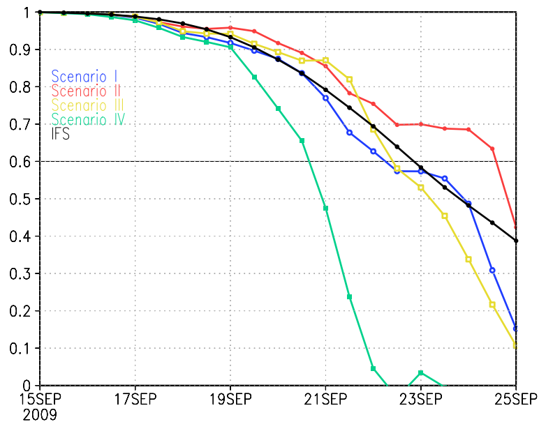
Figure 5.33: Anomaly Correlation Coefficient for the four members of the operational ECMWF EPS forecast for Typhoon Choi-Wan, the ECMWF analysis and the ERA-Interim climatology for the 500 hPa geopotential field between 20-60°N and 120-300°W for scenario I (blue), scenario II (red), scenario III (yellow) and scenario IV (green). General forecast accuracy of the operational deterministic ECMWF forecast is highlighted in black. Forecast was initialised on 00 UTC, 15 September 2009.
