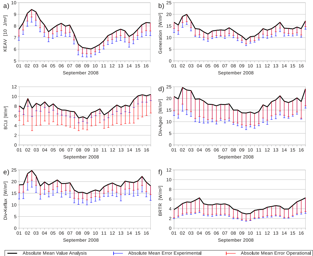
Figure 5.3: Absolute mean (black), MAE for the experimental (blue) and operational (red) data set for the budget terms, averaged over a region between 20°N to 65°N, 110°W to 20°E for each day in the first half of September 2008. As magnitude of quantities is lower, compared to the analysis values, only negative error bars are drawn. a) eddy kinetic energy ( K_e ), b) total generation ( generation ), c) baroclinic conversion ( bcli ), d) ageostrophic geopotential flux divergence (DLVP= div-ageo ), e) divergence of K_e flux with total wind (DLKE= div-keflux ), f) barotropic conversion ( brtr ). K_e in 10^5 J/m^2 , budget terms in W/m^2 .
