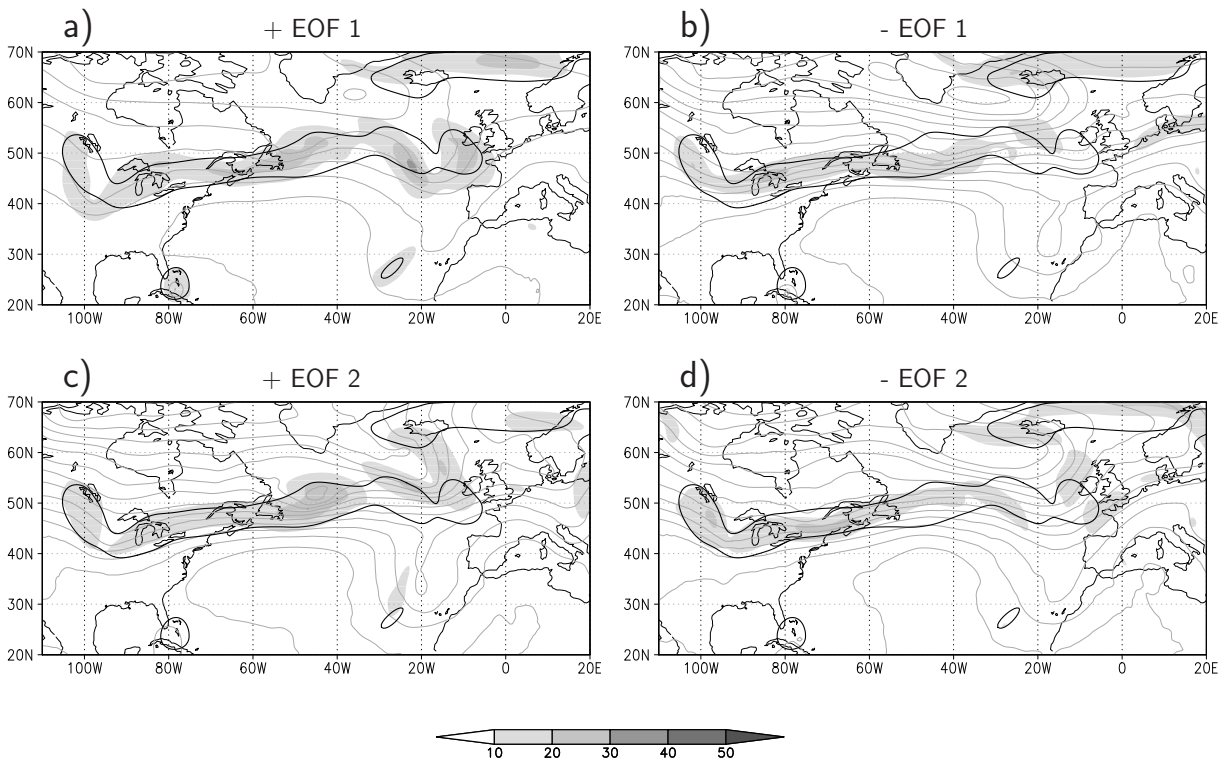
Figure 5.9: Vertically integrated K_e (shaded, in 10^5 J/m^2 ) and ensemble mean for K_e (black contours, in 10^5 J/m^2 ) for ensemble members with distinct contributions to the EOF patterns for Hurricane Hanna at investigation time (00 UTC, 09 September 2008), ensemble mean for 500 hPa geopotential height as grey contours. a) Member with positive contribution to EOF 1 and neutral to EOF 2, b) Member with negative contribution to EOF 1 and neutral to EOF 2, c) Member with positive contribution to EOF 2 and neutral to EOF 1, d) Member with negative contribution to EOF 2 and neutral to EOF 1.
