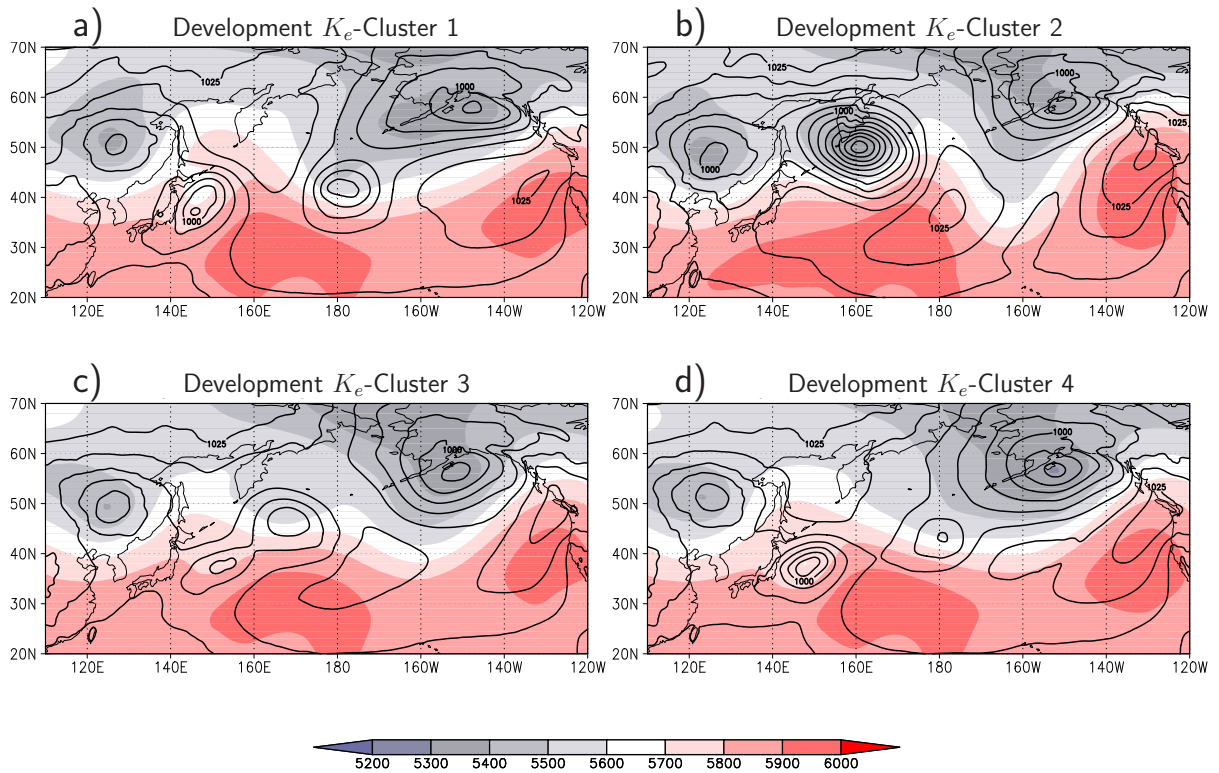
Figure 5.23: Cluster mean for 500 hPa geopotential height (in gpm ) and mean sea level pressure (in 5hPa increments) of the K_e -clusters for Typhoon Choi-Wan at investigation time (00 UTC, 21 September 2009). a) K_e -cluster 1, b) K_e -cluster 2, c) K_e -cluster 3, d) K_e -cluster 4.
