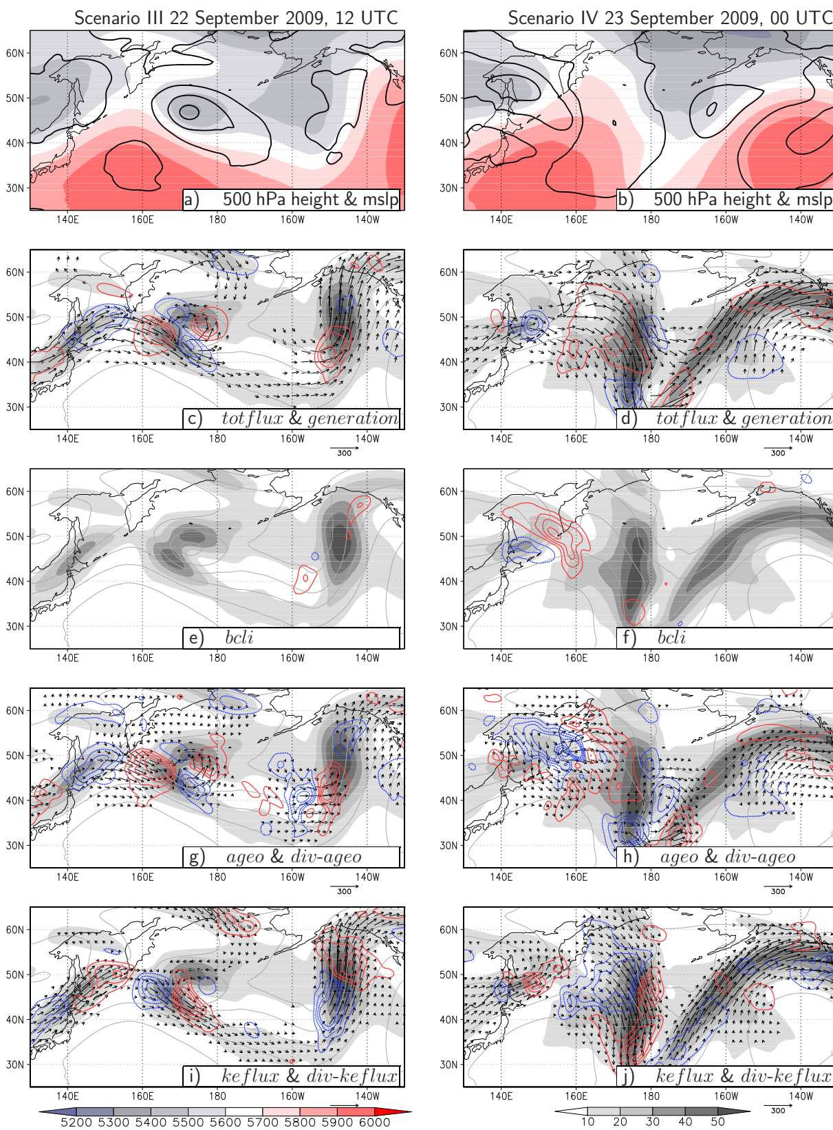
Figure 5.40: As Figure 5.35, but after completion of ET.
