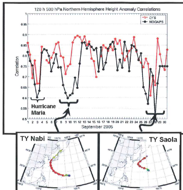
Figure 2.3: Anomaly correlation coefficient for 5 day forecast of 500 hPa geopotential height over the Northern Hemisphere during the ET of three tropical cyclones (Maria, Nabi and Saola) in 2005. The ET of the tropical cyclones caused a significant drop in predictability. Red: Global Forecast System from the National Centres for Environmental Prediction (NCEP-GFS). Black: Navy Operational Global Atmospheric Prediction System (NOGAPS). Figure 1 from Harr (2010).
