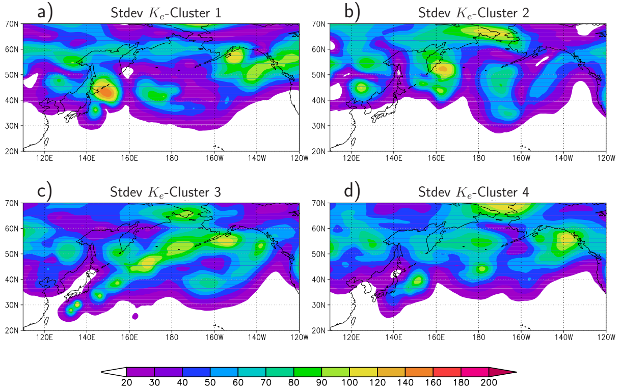
Figure 5.22: Standard deviation (in gpm ) for 500 hPa geopotential height of the K_e -clusters for Typhoon Choi-Wan at investigation time (00 UTC, 21 September 2009). a) K_e -cluster 1, b) K_e -cluster 2, c) K_e -cluster 3, d) K_e -cluster 4.
