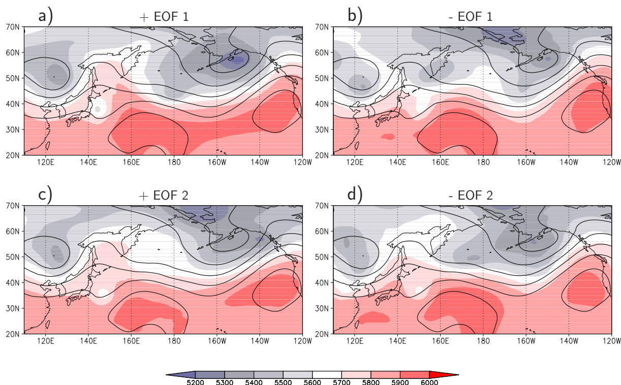
Figure 5.17: 500 hPa geopotential height (shaded, in gpm ) and ensemble mean for 500 hPa geopotential height (contours, in gpm ) for ensemble members with distinct contributions to the EOF patterns for Typhoon Choi-Wan at investigation time (00 UTC, 21 September 2009). a) Member with positive contribution to EOF 1 and neutral to EOF 2, b) Member with negative contribution to EOF 1 and neutral to EOF 2, c) Member with positive contribution to EOF 2 and neutral to EOF 1, d) Member with negative contribution to EOF 2 and neutral to EOF 1.
