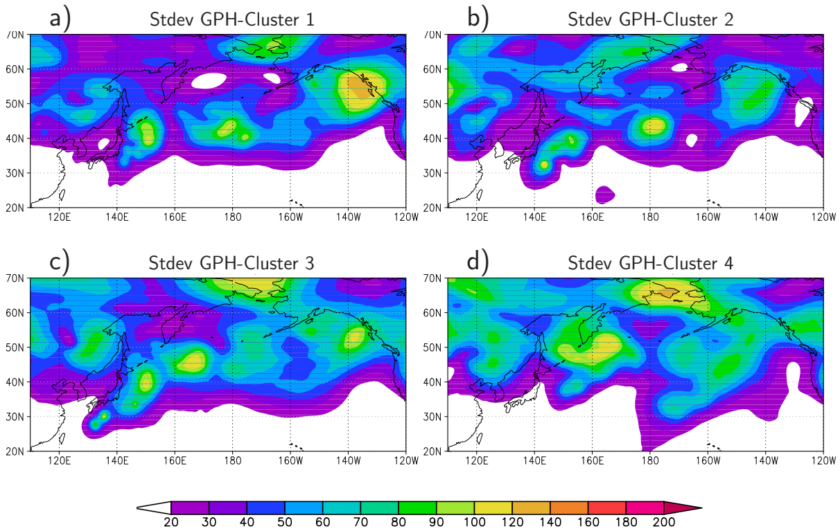
Figure 5.20: Standard deviation (in gpm ) for 500 hPa geopotential height of the GPH-clusters for Typhoon Choi-Wan at investigation time (00 UTC, 21 September 2009). a) GPH-cluster 1, b) GPH-cluster 2, c) GPH-cluster 3, d) GPH-cluster 4.
