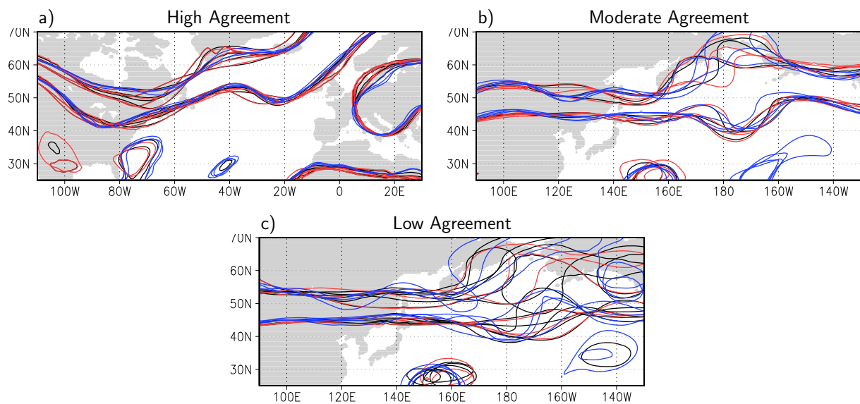
Figure 4.9: Spaghetti plots for 5500, 5700, 5900 gpm isolines of cluster means from the TIGGE (black), TI-EC (red) and ECMWF (blue) development scenarios. Shown are three cases, which characterise a) high, b) moderate and c) low agreement between the black (TIGGE) and red (TI-EC) lines.
