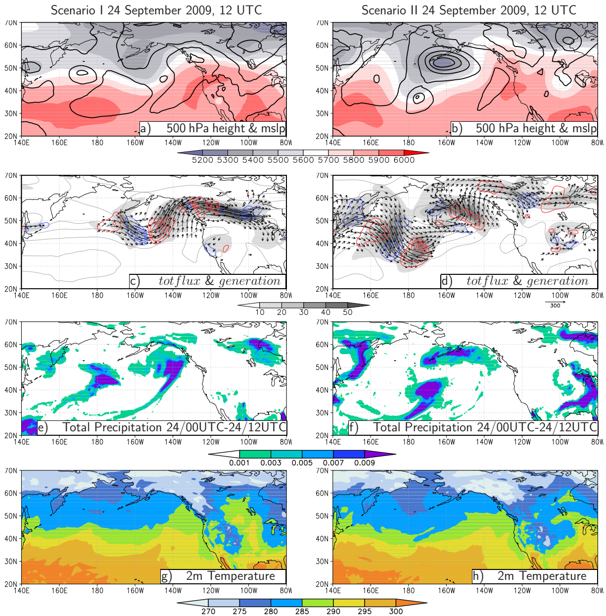
Figure 5.41: Distinct synoptic fields towards the end of the investigated forecast period for development scenarios for Typhoon Choi-Wan (valid at 24 September 2009, 12 UTC. a,b) 500 hPa geopotential height (shaded, in gpm) and mslp (contours, in 5 hPa increments) for scenario I and II, c,d) total eddy kinetic energy, generation and totflux , as Figure 5.34 for scenario I e,f) sum of large scale and convective precipitation (in m) between 24 September 2009, 00 UTC and 12 UTC scenario I and II, g,h) 2 m Temperature (in K) for scenario I and II
