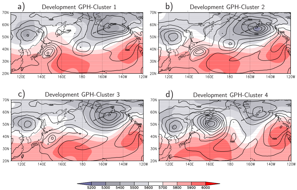
Figure 5.21: Cluster mean for 500 hPa geopotential height (in gpm ) and mean sea level pressure (in 5hPa increments) of the GPH-clusters for Typhoon Choi-Wan at investigation time (00 UTC, 21 September 2009). a) GPH-cluster 1, b) GPH-cluster 2, c) GPH-cluster 3, d) GPH-cluster 4.
