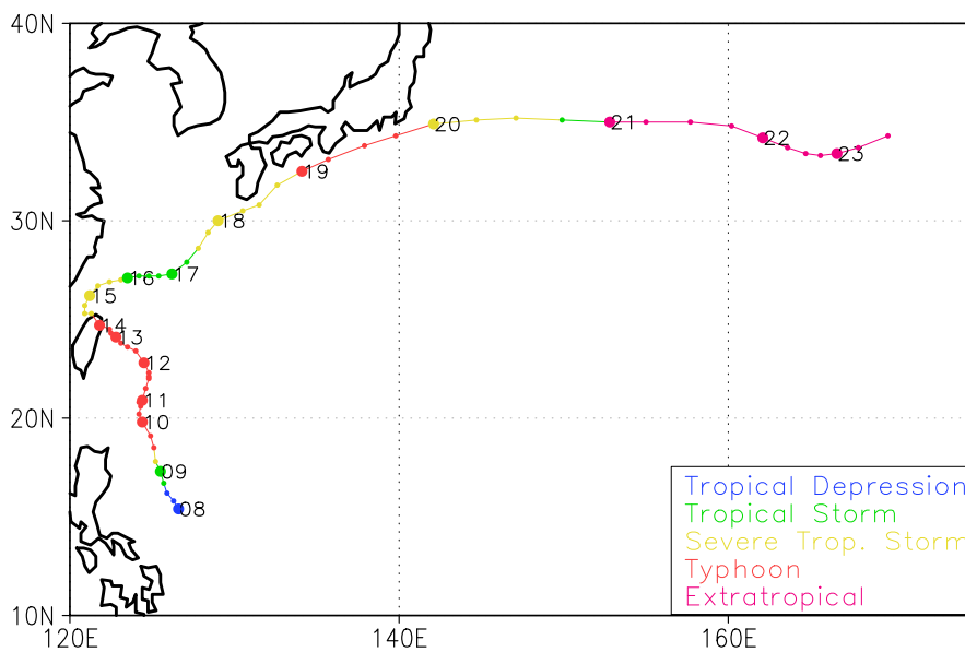
Figure 2.7: Track for Typhoon Sinlaku in September 2008. Dots mark the position of Typhoon Sinlaku every 6 hours. Large dots describe position at 00 UTC of the indicated day (number). Intensity in colours, as given in legend. Based on best track data from the Regional Specialised Meteorological Center (RSMC), Typhoon Center-Tokyo, Japan Meteorological Agency (JMA, http://www.jma.go.jp/jma/jma-eng/jma-center/rsmc-hp-pub-eg/besttrack.html ).
