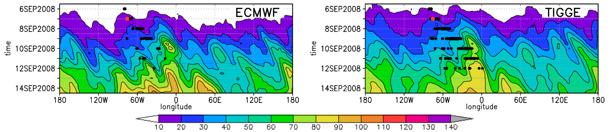
Figure 4.2: As Figure 4.1 but for forecast of Hurricane Hanna, where ECMWF and TIGGE show closely related patterns of standard deviation.
