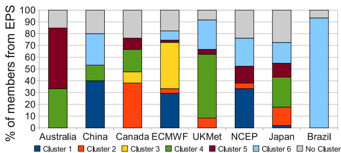
Figure 4.6: Contribution of members from the individual EPS to the different clusters (in colours) for Ike10. Ordinate: % of members from the given EPS contributing to the cluster in question (in colour). Members that could not be clearly assigned to one cluster are outlined in grey (taken from Keller et al., 2011).
