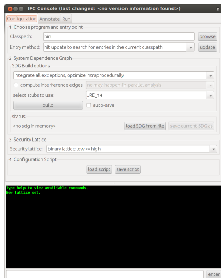
(a) configuration tab including console
