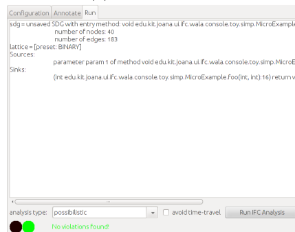
(c) analysis tab
