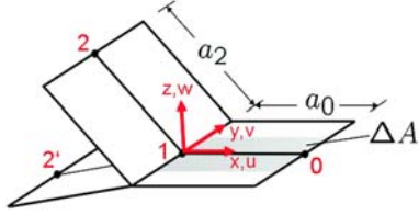
Figure 3: VCCT model with arbitrary rectangular shell elements and strain energy release rates
