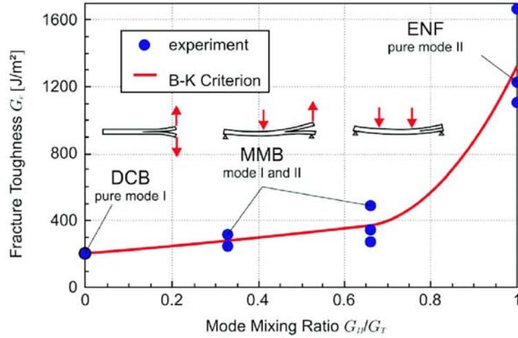
Figure 4: Original B-K-law [4] for mixed mode I-II. Graph taken from [18]
