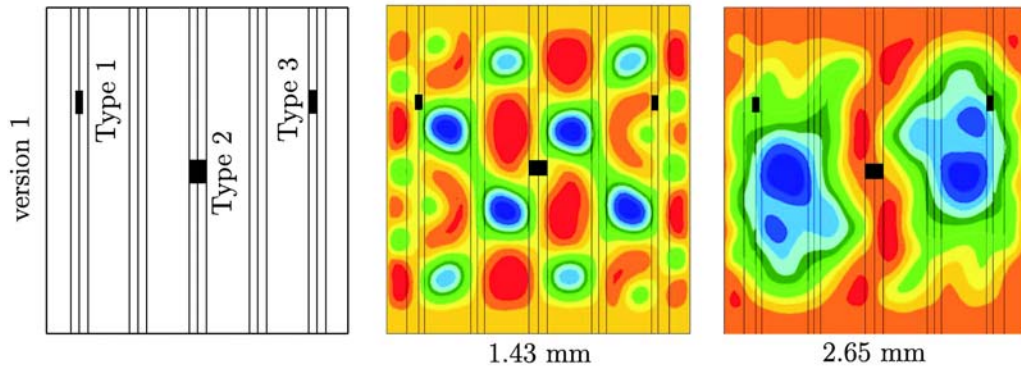
Figure 10: Pre-damaged configuration V1: Initial damage configuration and contour plots including the current state of debonding
