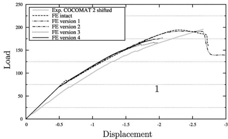
Figure 16: Comparison of the global behaviour at the final state: Intact and pre-damaged V1 - 4
