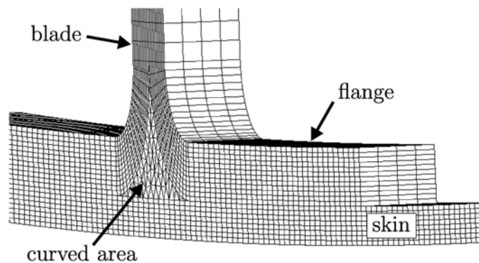
Figure 7: Section of the generated model for the structural zooming analysis
