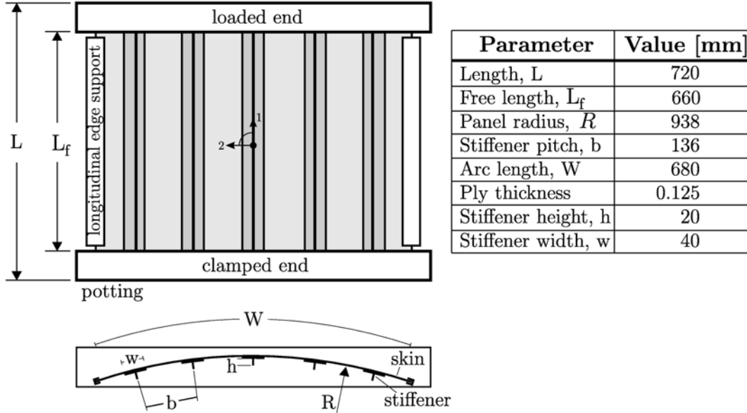
Figure 1: Experimental set-up and dimensions in [mm] for both intact and pre-damaged configuration
