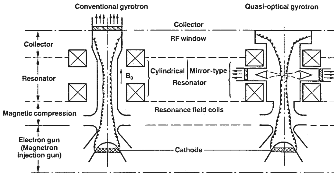
Fig. 2: Principle of a conventional gyrotron with cylindrical resonator and of a quasi-optical gyrotron with mirror resonator [75,76].
