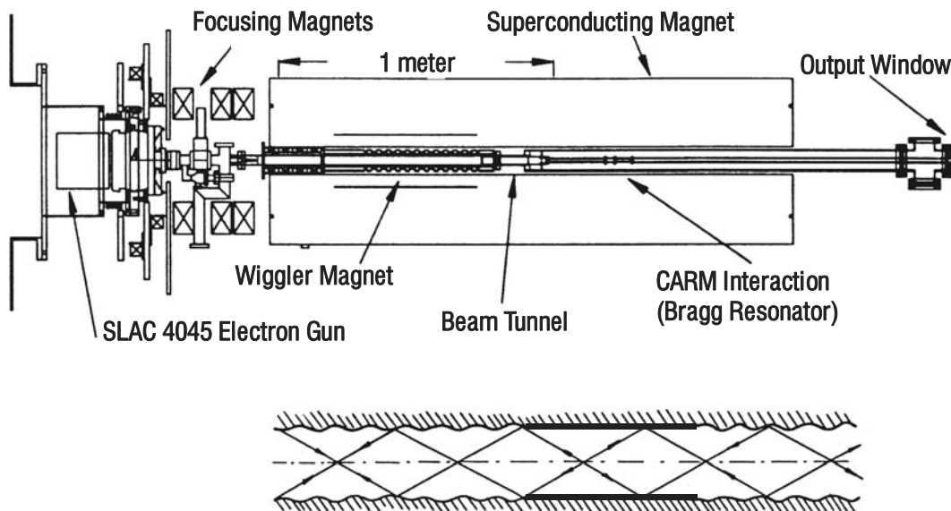
Fig. 7: Schematic of the long-pulse MIT CARM oscillator experiment [266] and scheme of a Bragg resonator [236].
