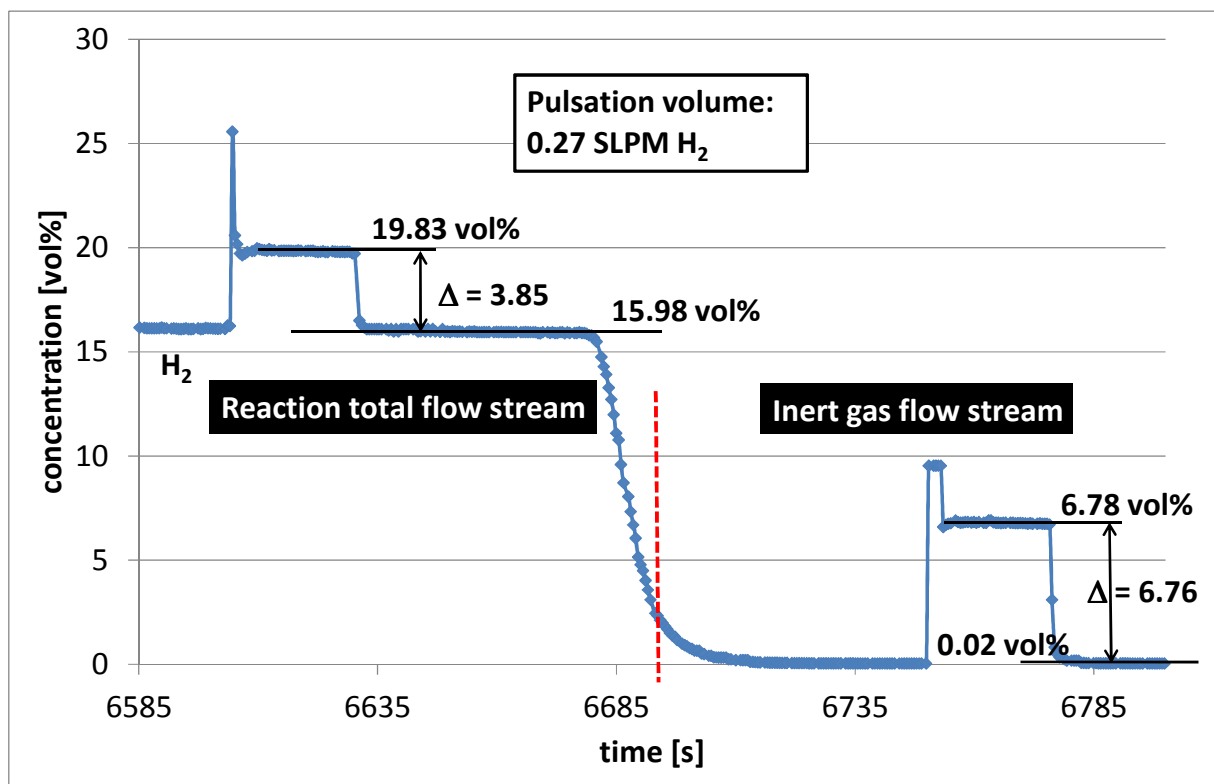
Figure 4-10: Method of internal standard for total flow determination. Shown is an exemplary pulse sequence of 0.27 SLPM H 2 into the reaction total gas stream (left) and the pure nitrogen flow (right).
