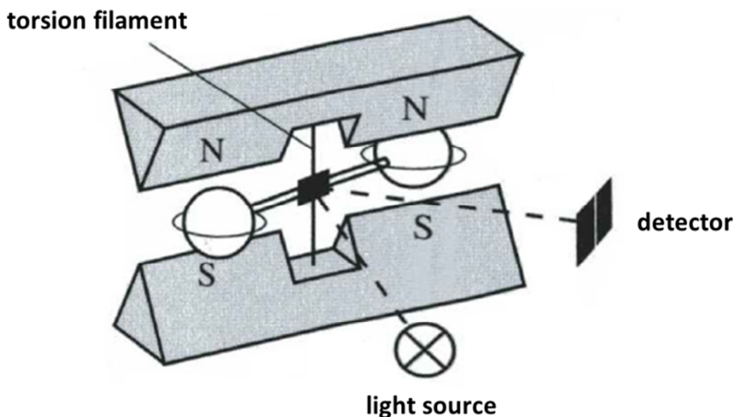
Figure 4-9: Schematic illustration of the magneto-mechanic detection principle, adapted from [107].
