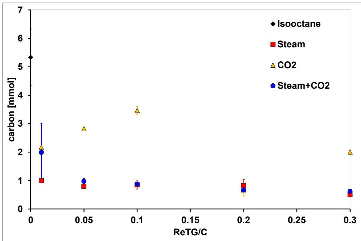
Figure 6-7: Calculated amount of carbon deposition from carbon burn-off experiments for each ReTG/C ratio and isooctane reference. Each value represents the overall carbon amount for C/O 0.72 – 1.79. Error margins are calculated from the total amount of C detected in the carbon burn-off experiments performed after each measurement and its rerun.
