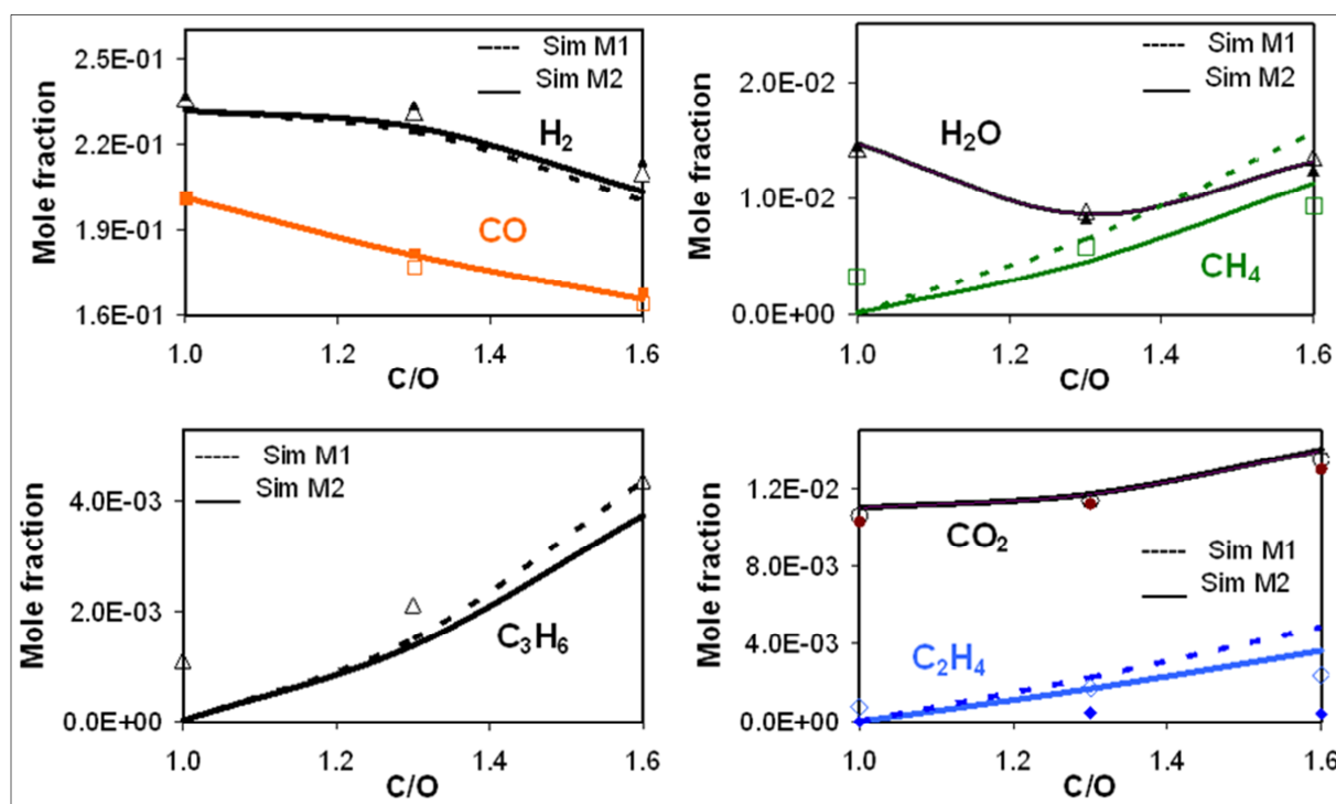
Figure 5-6: Species profiles for varying C/O ratios at 993 K; open symbols = experiment, dashed/solid lines = simulations with mechanisms M1/M2, filled symbols = inlet.
