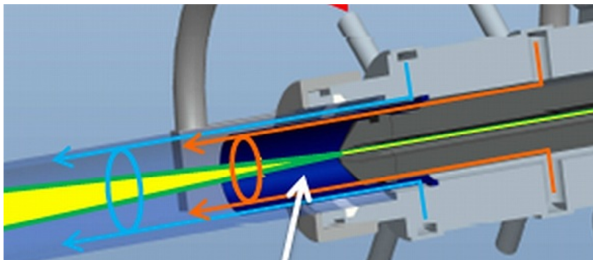
Figure 4-2: Enlarged section of the tube-in-tube configuration of Figure 4-1 (same labeling).
