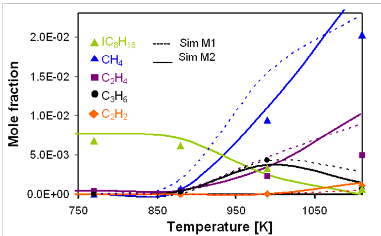
Figure 5-5: Product distribution as a function of temperature measured in the center of the reactor tube for C/O=1.6 ; symbols = experiment, dashed/solid lines = simulations with M1/2.
