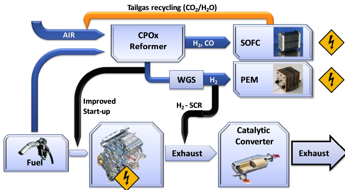
Figure 2-1: Concept drawing of an APU. The bottom path shows the conventional principle of a today's automobile with internal combustion engine (ICE), generator, and exhaust gas after-treatment. The electricity production is performed by the generator, driven by the ICE. The upper path describes the combination of CPOx reformer and fuel cell stack with additional options for start-up and emission control improvement. Reprinted from [36] with permission from ACS.
