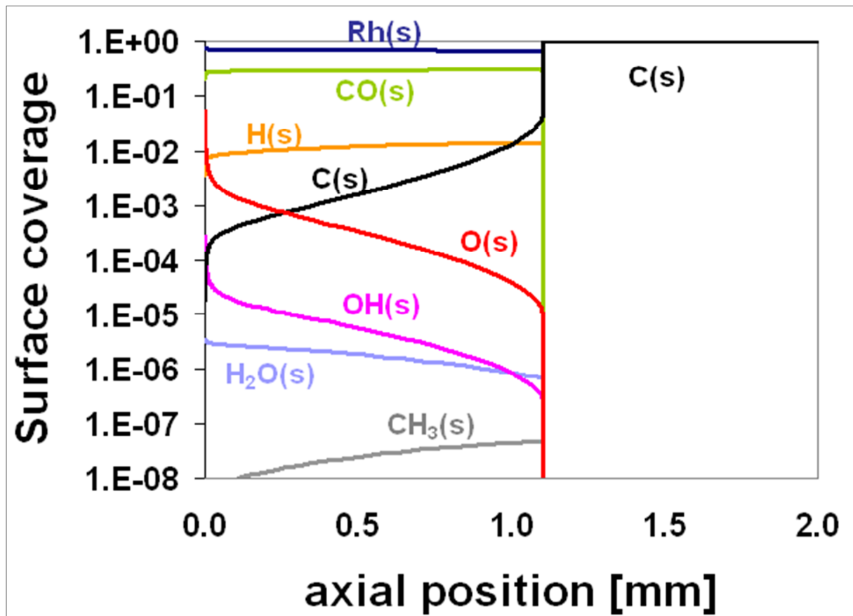
Figure 5-2: Numerically predicted surface coverage of adsorbed species as a function of axial position along the monolith channel: C/O = 1.1, 1080 K, 80 % N 2 dilution, 4 SLPM.
