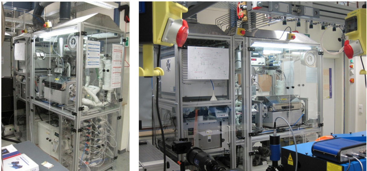
Figure 4-6: Pictures of the installed reactor set-up close to the laser system (blue device, bottom right in the right picture)
