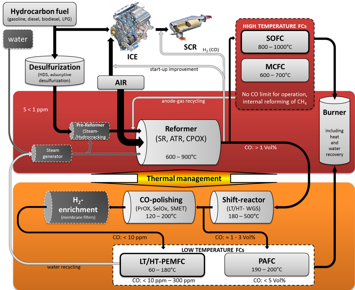
Figure 1-1: Detailed concept chart of an APU, including pre-treatment of the hydrocarbon fuel (desulfurization, pre-reforming), the conversion of fuel to hydrogen-rich gas mixtures (Reformer), direct use in high-temperature fuel cells (upper right), CO removal (HT/LT WGS, CO-polishing), hydrogen enrichment and use in low-temperature fuel cells (bottom middle). Blackened parts are not necessary in general; their usage depends on the process demands based on fuel source and hydrogen quality. Greyed lines indicate fuel processor integration in the APU / vehicle. For efficiency improvement and energy recuperation, a significant focus has to be put on thermal management, as different temperature regimes are present in a fuel processor (indicated in red (HT) and orange (LT)).
