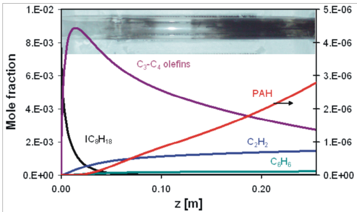
Figure 5-4: The distribution of carbon precursors along the reactor modeled with mechanism M2; C/O = 1.6 , 1108 K, 6 SLPM. C_3 - C_4 olefins contain 1,2-propadiene, propene, propyne, n-butene (1-buten, 2-butene), iso-butene, and 1,3-butadiene; PAH contains naphthalene, anthracene, and pyrene. Embedded photo shows the tubular quartz reactor after operation.
