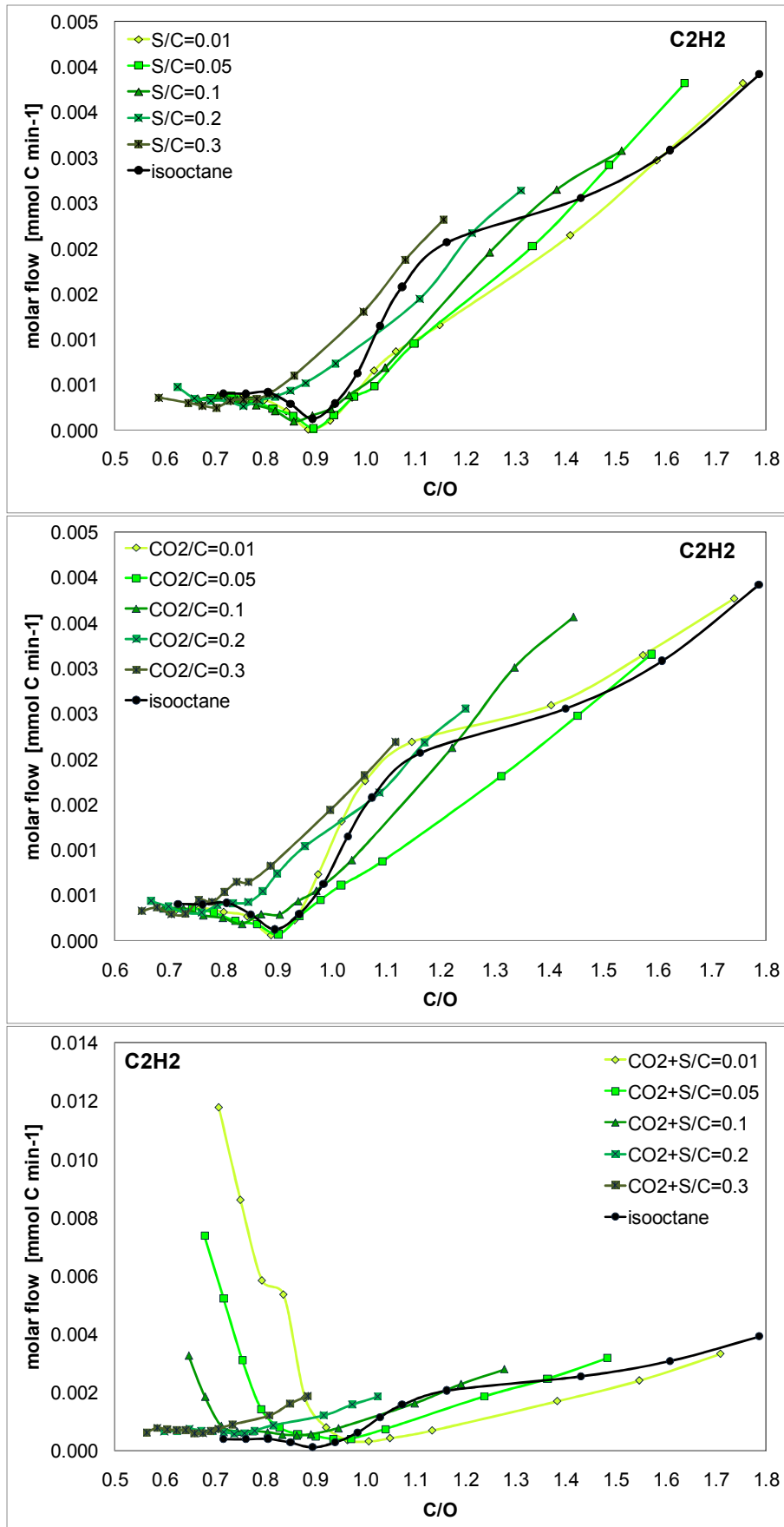
Figure 6-6: Molar flow rates of C 1 -C 3 byproducts for case 1-3 and the five ReTG/C ratios.
