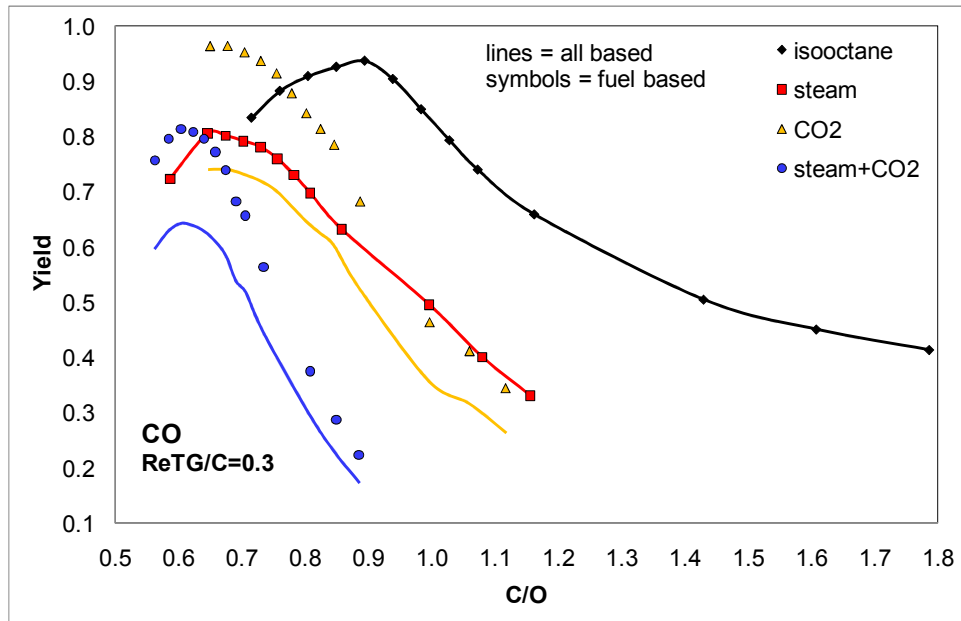
Figure 6-1: Yield of H 2 and CO for cases 1-3 and the five different ReTG/C ratios. Full lines = all-based C/H yield, symbol = fuel-based C/H yield.
