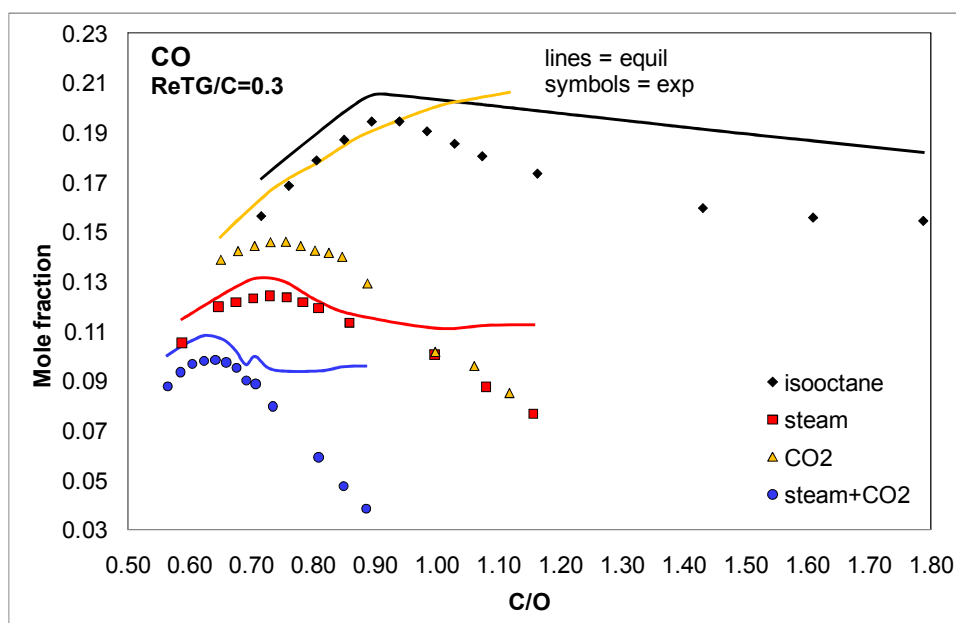
Figure 6-8: Mole fractions of H 2 and CO for case study 1-3 and the five different ReTG/C ratios. Full lines = calculated mole fractions at equilibrium for measured outlet temperatures, symbol = experiment.
