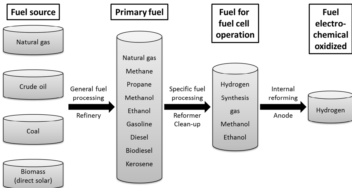
Figure C-1: Chart of fuel flow from source to hydrogen, taken from [99].
