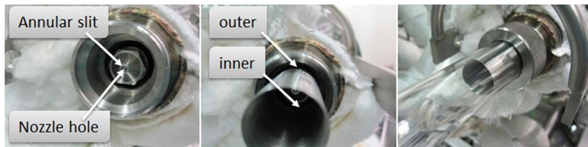
Figure 4-3: Picture of the two-substance stainless steel nozzle integrated in the tube-in-tube inlet configuration. Left: nozzle without inner tube installed. Middle: with installed inner tube. Right: complete configuration with quartz glass tube.
