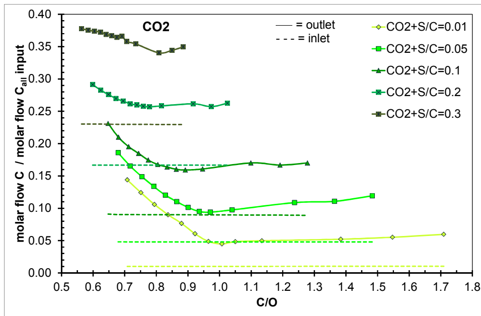
Figure 6-4: Input-referenced molar flow rates for \text{H}_2\text{O} and \text{CO}_2 input (dashed lines) and output (full lines) of the reactor. Upper first = case 1, second = case 2, last two = case 3.
