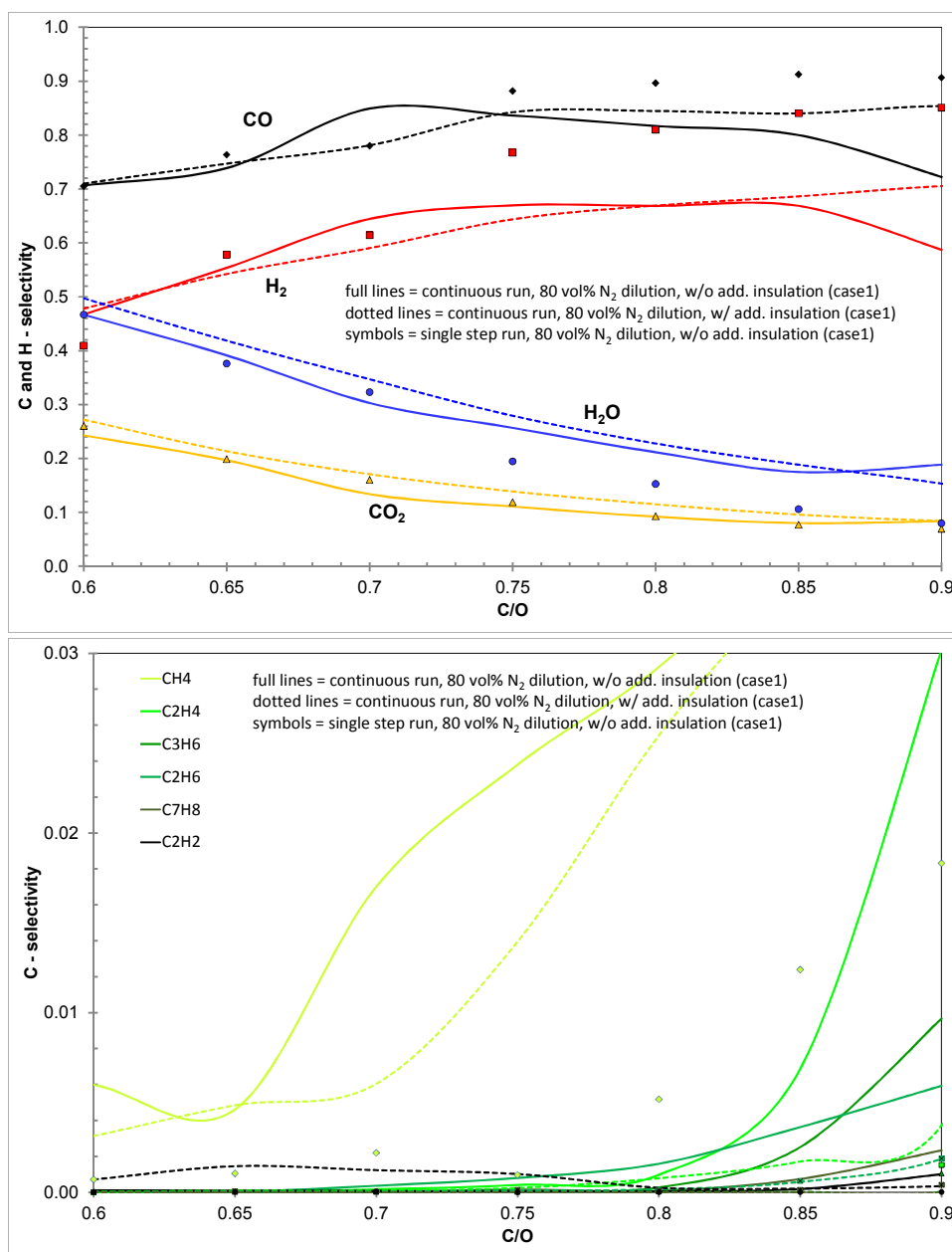
Figure 7-5: TOP: Main product distribution as function of the C/O ratio for Study 1 over a C/O ranging from 0.6 – 0.9. Trends are very similar for the single-step and continuous-run experiments (dotted lines with additional catalyst insulation). In case of an additional insulation of the catalyst, a more stable operation is noticeable regarding the production of syngas. Deviations from the single-step run experiments, especially for higher C/O ratios, could arise from the fact that, for the continuous runs, a carbon layer starts forming on the catalytic surface with increasing C/O, which slightly deactivates the catalytic activity. BOTTOM: Side product distribution as function of the C/O ratio for Study 1 over a C/O ranging from 0.6 – 0.9. Trends are very similar for the single-step and continuous-run experiments (dotted lines with additional catalyst insulation). In case of an additional insulation of the catalyst, side product formation is reduced. Since, for the single-step run experiments, even less C1 – C3 species were detected than for the continuous-run experiments, the actual condition state of the surface is imported for the interpretation of the measured results.
