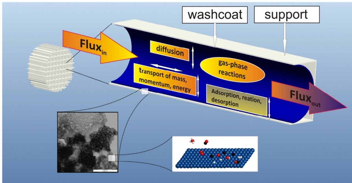
Figure 3-1: Modeling stages in a monolithic honeycomb catalyst channel.
