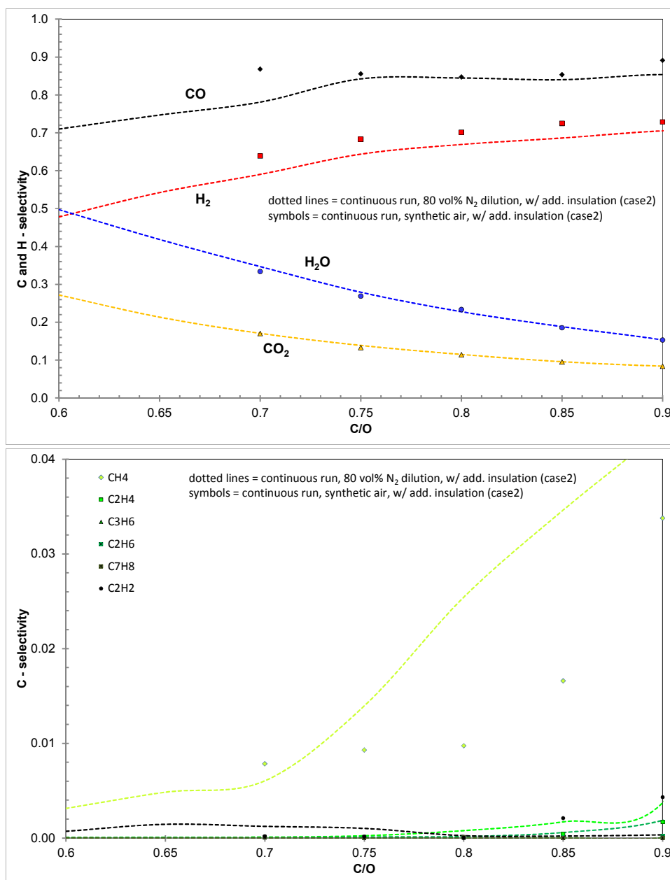
Figure 7-7: TOP: Comparison of the continuous run of Study 1 and Study 2 (both with additional insulation of the catalyst) with regard to main product distribution as function of the C/O ratio. Slightly higher selectivities in syngas production were detected in case of the synthetic air mixture. Total oxidation products stay at the same level as for the 80% nitrogen dilution case. BOTTOM: Comparison of the continuous run of study1 and Study 2 (both with additional insulation of the catalyst) with regard to side product distribution as function of the C/O ratio. Compared to Study 1 the higher oxygen content in Study 2 reduces the formation of smaller hydrocarbons. Significant reduction of CH 4 is observed.
