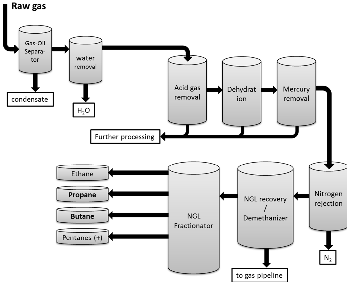
Figure C-2: Schematic gas processing of a natural raw gas, taken from [99].
