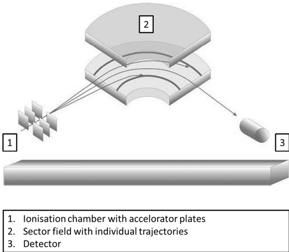
Figure 4-8: Schematic illustration of a sector field mass spectrometer, adapted from [108]
