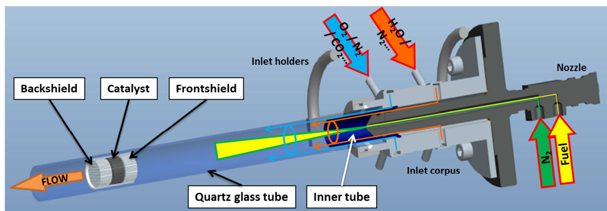
Figure 4-1: Schematic drawing of the inlet configuration: The nozzle (right) is placed in a stainless steel inlet corpus providing the liquid fuel (yellow) and the carrier gas (green). The nozzle tip ends in an inner stainless steel tube with a wall thickness of only 0.2 mm. An inner gas stream (red) keeps the nebulized fuel away from the inner tube wall and provides further non-reactive inlet stream components such as water vapor. The inner tube (dark blue) finally ends in the reactor quartz glass tube. Through a second small annular slit between inner and quartz glass tube, further gaseous components are provided containing the reactive oxygen (light blue). As a consequence of the small slit mentioned, high gas velocities are achieved, which additionally contribute to keeping the nebulized fuel away from the reactor wall.
