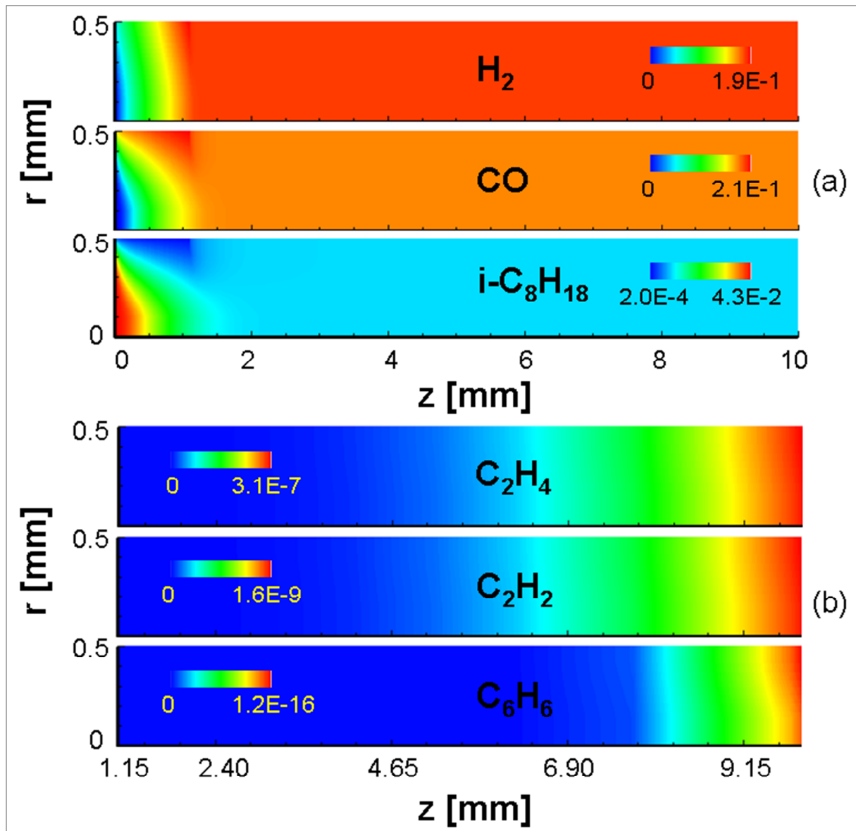
Figure 5-1: Numerically predicted mole fractions of isooctane, CO, H_2 (a) and ethylene, acetylene, and benzene (b) in the catalytic channel at C/O = 1.1 , 1080 K, 80 % N_2 dilution. The symmetry axis of the channel and the gas-wall interface are at r = 0 and 0.5 mm, respectively.
