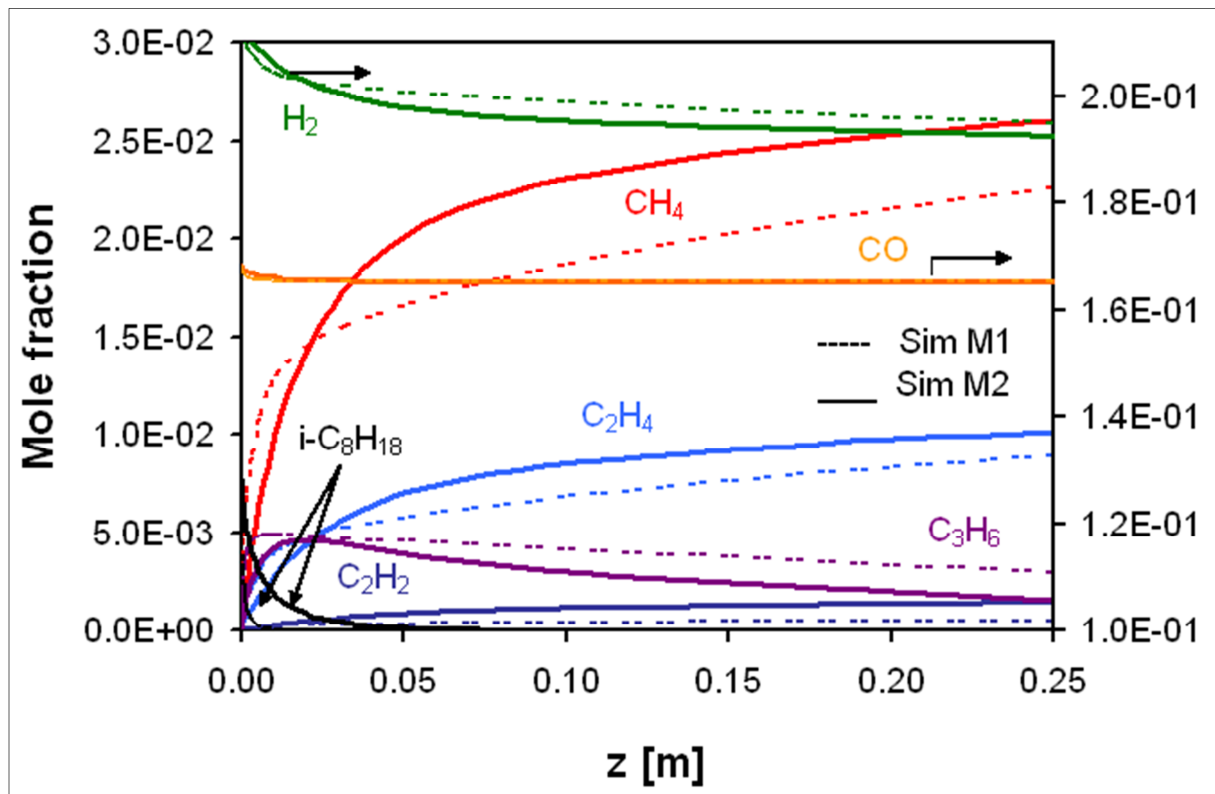
Figure 5-3: Numerically predicted fuel and product profiles with mechanisms M1 (dashed lines) and M2 (solid lines) as a function of axial position along the reactor; \text{C}/\text{O} = 1.6 , 1108 K, 6 SLPM.
