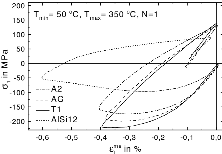
Abb. 8.107. \sigma_n - \epsilon_t^{me} -Hysteresen, TMF-Beanspruchung, T_{\max} = 350\text{ °C} , N = 1
