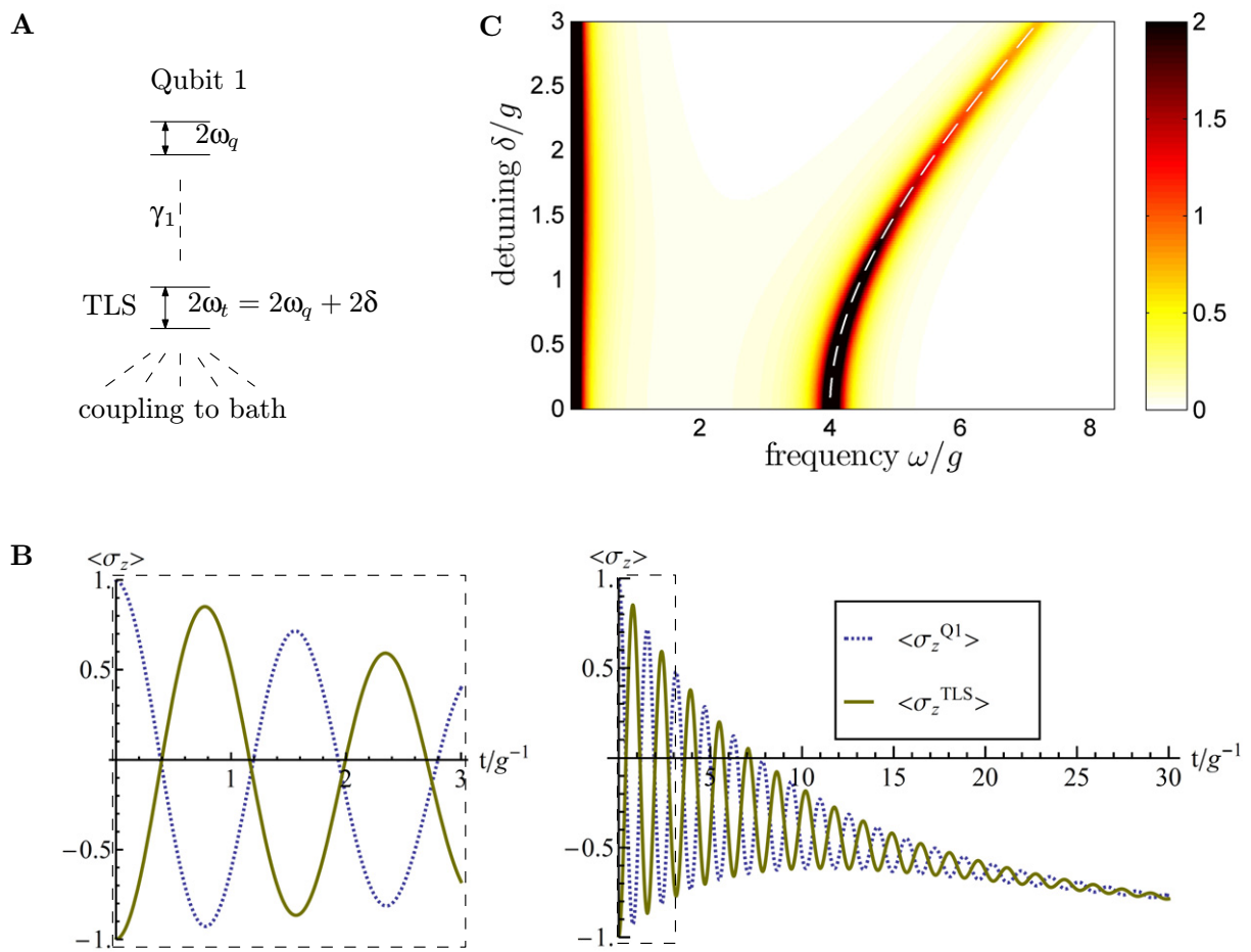
Figure 2. (A) Illustration of the simplified model system of one qubit with level splitting \omega_q coupled with coupling strength g_1 to an environmental TLS detuned by \delta . The TLS in turn is coupled to a bath. This system follows from figure 1(A) by setting g_2 = 0 . (B) Expectation values for the case of a single qubit coupled to a TLS as a function of time for \Gamma_1 = \Gamma_\varphi = 0.1g_1 ; g_2 = 0 ; \delta = 0 . (C) Real part of the one-sided Fourier transform of \langle \sigma_z^{Q1} \rangle(t) as a function of detuning \delta with \Gamma_1 = \Gamma_\varphi = 0.1g_1 ; g_2 = 0 . This is a numerical solution of either the Bloch–Redfield equations, where \Gamma_1 and \Gamma_\varphi are the definitions given by equations (6) and (7), or a numerical solution of the Lindblad equations with phenomenological rates. Analytically we find the angular frequency of the oscillation: \omega_{\text{osc}} = 2\sqrt{\delta^2 + 4g_1^2} , which is drawn as a dashed line. For details of the calculation, see section 3.1.
