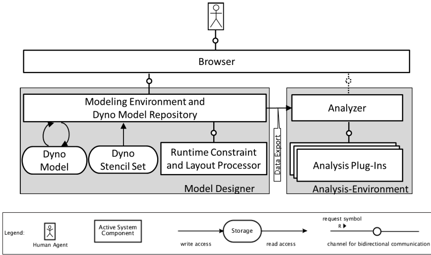
Figure 41: Editor architecture
