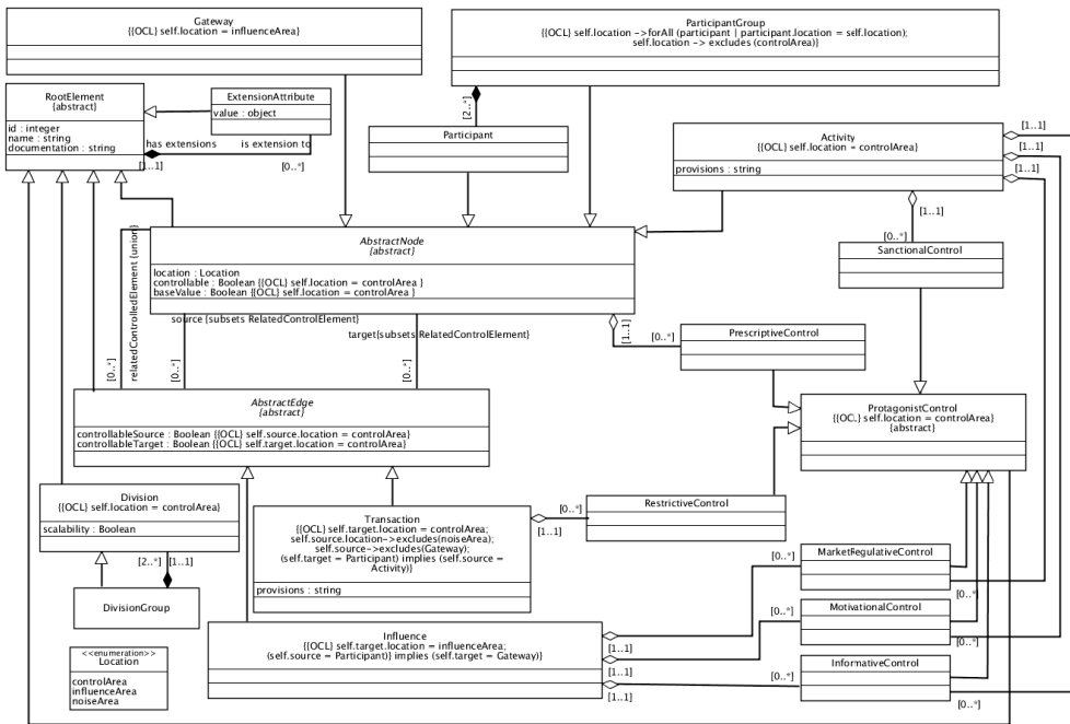
Figure 22: Complete Dyno meta-model
