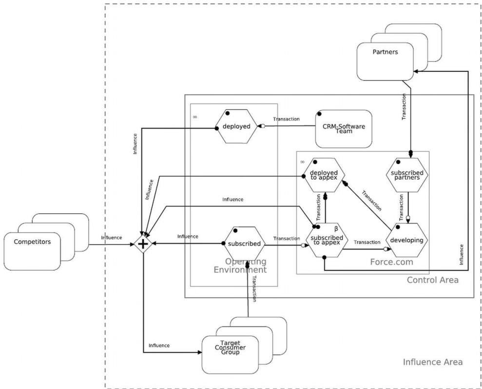
Figure 32: Salesforce, growth phase 3, screenshot from Dyno-Editor
