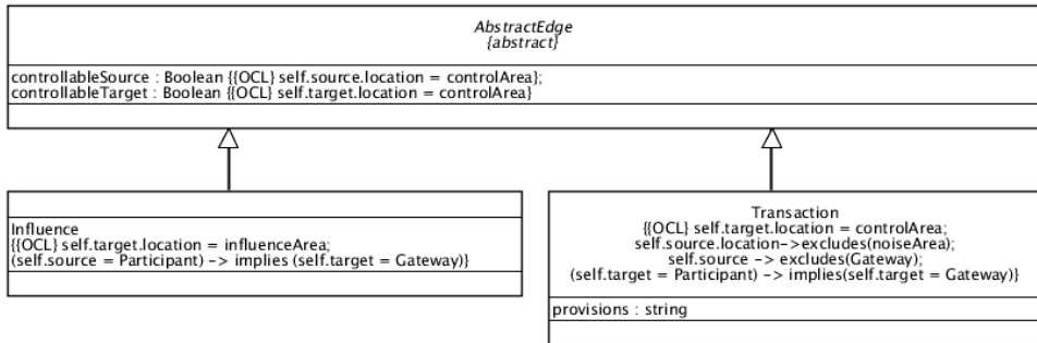
Figure 27: Definition of edges
