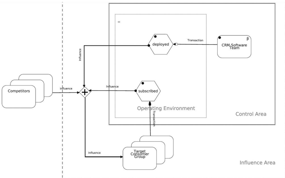
Figure 29: Salesforce, Launch phase, screenshot from Dyno-Editor
