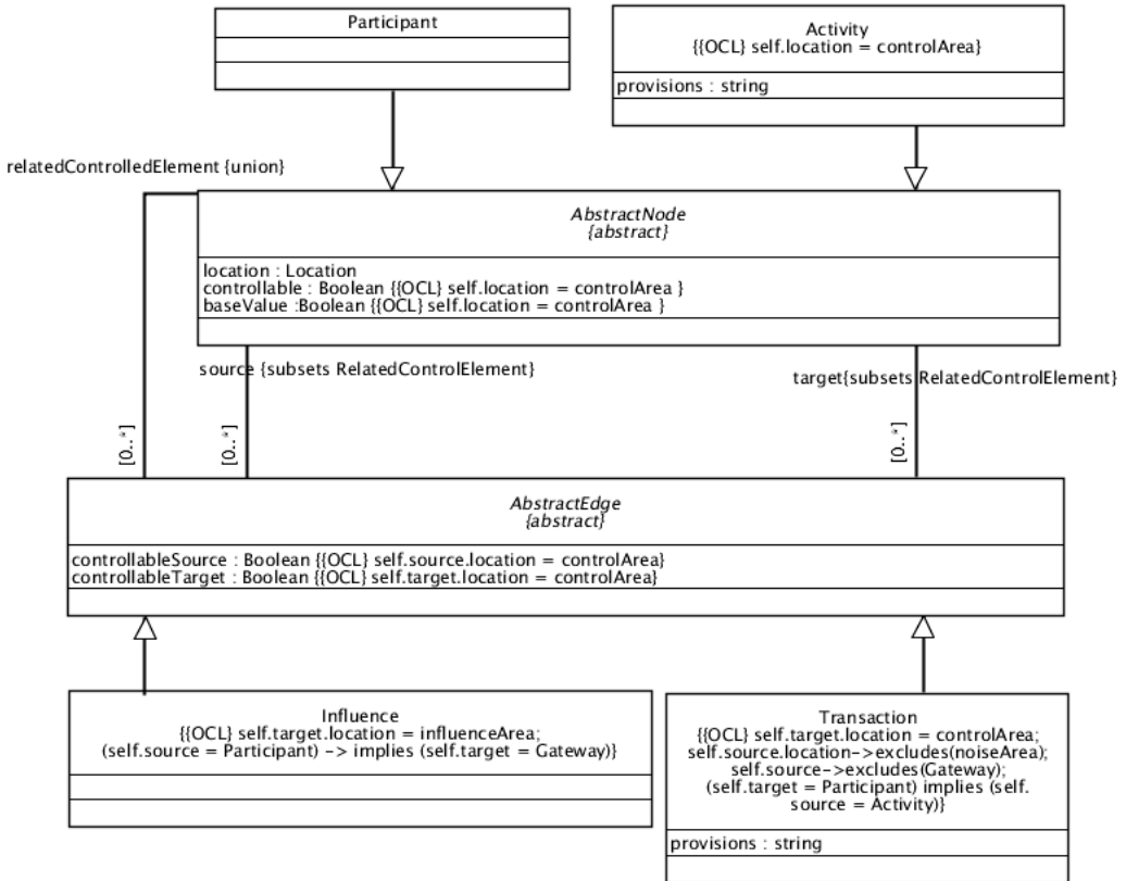
Figure 24: Core nodes and edges
