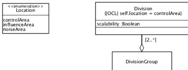
Figure 26: Location and divisions
