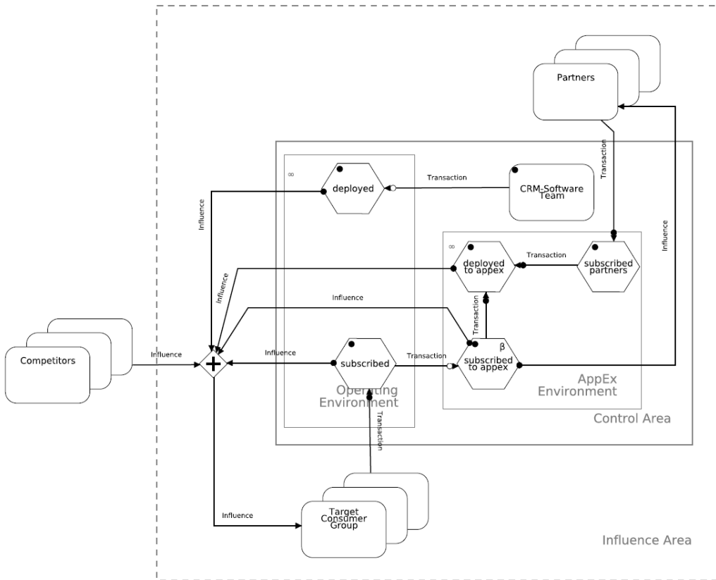
Figure 31: Salesforce, growth phase 2, screenshot from Dyno-editor
