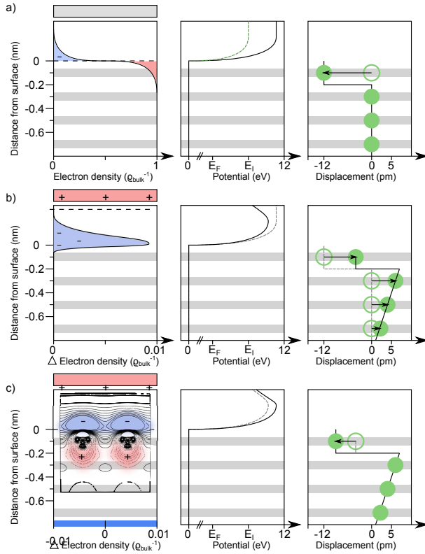
Figure 7.1: Metal surface (bottom electrode) in the homogeneous electric field of a thin (charged) plate (top electrode), separated by a vacuum barrier. The gray horizontal bars give the positions of the ion cores. a) E = 0 , jellium model: the finite wavelength of the electrons leads to a surface dipole ( e^- excess blue, deficiency red). This is reflected in an increase of the potential barrier for the electrons and a considerable displacement of the ion cores depicted in green (dashed lines describe the situation before). b) E > 0 , classical: the screening charge (here: negative, blue) is superpositioned with the surface dipole from a) (not shown for simplicity). The metal surface is attracted by the electrode, which leads to an outward displacement of the atomic cores. c) E > 0 , discrete lateral distribution of positive ions: besides the classical screening charge above the topmost atomic layer (blue), also in between the atoms charges are redistributed [91]. This additional dipole-like charge adds up to the work function and induces further displacements of the atoms.
