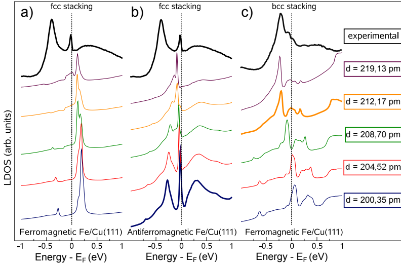
Figure 4.4: Scanning tunneling spectroscopy measurements in comparison with first-principles calculations of the LDOS for different magnetic scenarios. Three possible configurations were considered: (a) FM fcc, (b) AFM fcc and (c) FM bcc stacking. Additionally, different surface interlayer distances were considered for each configuration. The (dI/dU)/T spectrum obtained on the fcc phase (thick black line, top) does not fit the calculated LDOS for the FM fcc stacking irrespective of the interlayer distance (a). It only agrees with the calculated LDOS for an AFM configuration, in particular for an interlayer distance of 200 pm (blue curve) (b). The experimental spectrum on the bcc (c) phase agrees best with the theoretical LDOS for the FM configuration and an interlayer distance of 212 pm (yellow curve).
