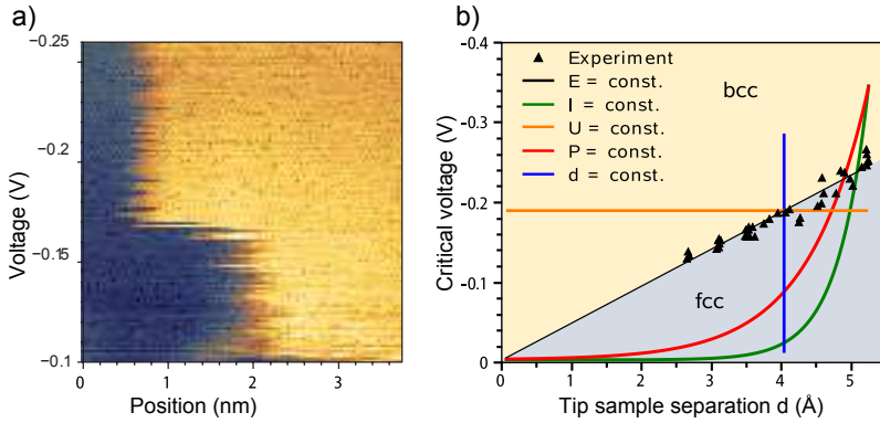
Figure 4.6: Controlling the structure of 2 ML Fe nano-islands with the local electric field. a) A single line across the fcc-bcc domain boundary was scanned with the STM while the voltage U was decreased scan line by scan line. At a critical voltage ( -0.16 V), a transition from fcc to bcc occurs. This experiment has been carried out at different tunneling currents (in a range from 150 pA to 28 nA), that is, with different tip-sample separations. b) By plotting the critical gap voltage against the corresponding tip-sample separation z , the boundary (black triangles) in the phase diagram is obtained. The experimental results can be compared with possible distance dependencies of the critical voltage (colored lines) resulting from different models (for details see main text): E = \text{const.} (black line), I = \text{const.} (green line), U = \text{const.} (yellow line), P = \text{const.} (red line), z = \text{const.} (blue line). The curves are all fitted freely to the experimental data.
