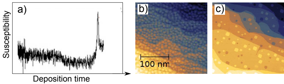
Figure 6.9: a) Magnetic susceptibility measured during deposition of Ni/Cu(100). b) Typical STM topography obtained on a Ni film deposited at room temperature. c) Topography of the annealed surface (same size as in b)) showing reduced surface roughness.
