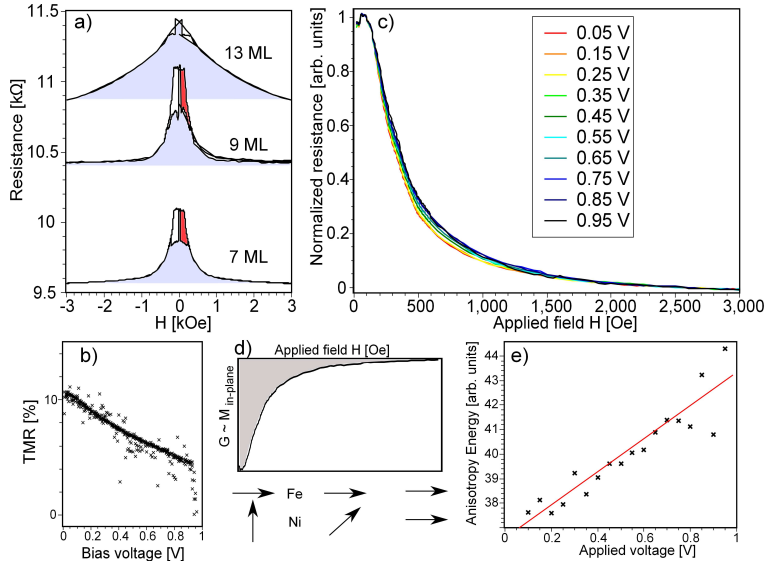
Figure 6.8: a) Resistance measured as a function of magnetic field. A 13 ML thick Ni film displays a continuous but slow decrease of the resistance with increasing field, indicative of a dominant out-of-plane anisotropy. Ni films with thicknesses of 9 ML and 7 ML show a small plateau at low magnetic fields and an abrupt decrease of the resistance with increasing magnetic fields, indicative of an in-plane easy axis of the magnetization at low magnetic fields. For all three curves, the symmetric contribution is shown in gray, the antisymmetric part is shown in red. Note that, more precisely, it is the conductances that add up. b) TMR ratio as a function of applied voltage for the 11 ML thick Ni film. c) Normalized resistance versus magnetic field, measured at applied bias voltages varied from 0.05 V to 0.95 V for a 11 ML thick Ni layer. d) Same measurement as c); variation of the conductance as a function of the applied field in combination with a possible orientation of the magnetization directions. The gray area is proportional to the out-of-plane anisotropy energy. e) Relative change of the magnetic anisotropy energy as a function of applied voltage, calculated from the data presented in c).
