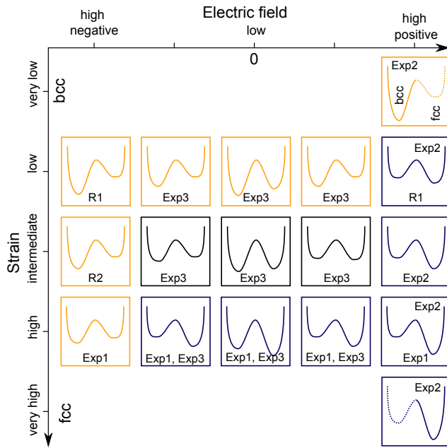
Figure 4.12: Electric field and strain dependence of the energy landscape of 2 ML Fe/Cu(111). The left minimum corresponds to the bcc lattice, the right one to the fcc lattice. Five different electric field regimes and five different strain regimes are distinguished. The energy landscapes qualitatively combine the experiments described above. Configurations that lead to AFM fcc and FM bcc are drawn in blue and in orange, respectively. Dotted parts are guesses following Fig. 4.10b).
