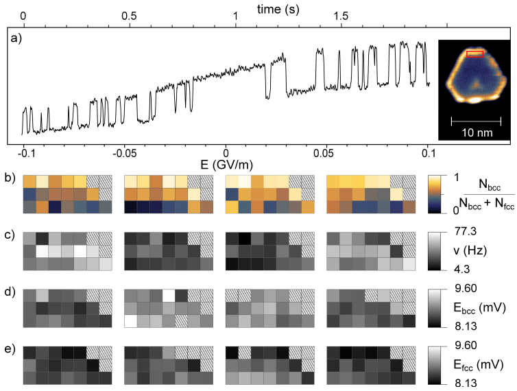
Figure 4.11: Combined electric-field and strain-dependent measurement of the switching parameters. a) Typical dI/dU curve as a function of time and applied electric field. Maps of the relative population of the bcc state (b), the switching frequency (c) and the energy barriers (d) and e)) on a grid of 7 \times 3 pixels (corresponding to 2.71 \times 0.78 \text{ nm}^2 ). The maps are placed below the corresponding electric field range in a). The domain boundary is located at the central row of the grid. Measurement points that showed only very few transitions are hatched.
