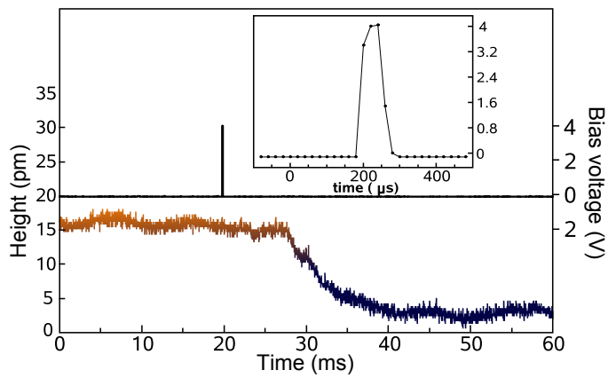
Figure 4.14: Applied bias (black line) and measured height (colored line) at fixed tip position. A pulse of 4 V and 60 \mu\text{s} was applied (see inset).
