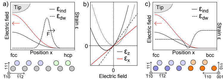
Figure 7.2: a) One-dimensional model of the fcc-hcp domain boundary in 1 ML Fe/Ni(111) in the electric field of an STM tip: the sphere model shows a (\bar{1}10) plane across the domain boundary between the fcc (blue) and hcp (green) Fe lattice on Ni (gray). The strain variation \epsilon_{dw} due to the misfit dislocation is depicted with the dashed black line. The lateral variation of the intensity of the electric field (perpendicular to the surface) of the STM tip is drawn in red. It results in a lateral variation of the in-plane strain \epsilon_{ind} (solid black line). A net force F on the domain wall results. b) Qualitative electric field dependence of lattice relaxations of the topmost atomic cores in a metal surface: the vertical displacement due to the electrostatic attraction scales with E^2 (black dotted line), while the stretch (black dashed line) scales linearly with E . The total vertical displacement, \epsilon_z , is shown by the black solid line. The value of the lateral strain \epsilon_x is shown by the red line. c) Similar to a), for the case of a boundary between fcc (blue) and bcc (orange) domains in 2 ML Fe/Cu(111). Here the bcc lattice is shown as an expanded fcc lattice (which is energetically not correct).
