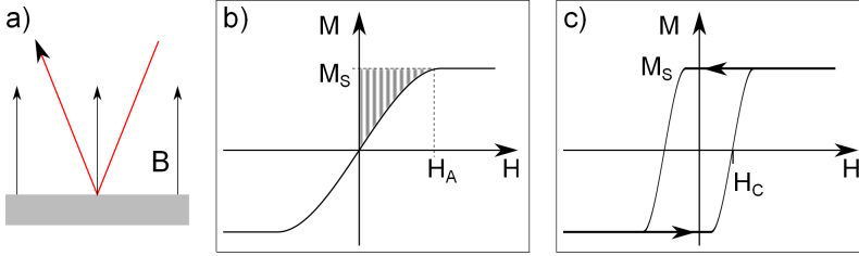
Figure 2.1: a) Polar MOKE configuration with the incident light (red) probing the out-of-plane component of the magnetization in a magnetic field perpendicular to the surface. b) Hysteresis loop of a sample with in-plane easy axis of magnetization measured with polar MOKE. The hatched area is equivalent to the anisotropy energy. c) Hysteresis loop with out-of-plane easy axis.
