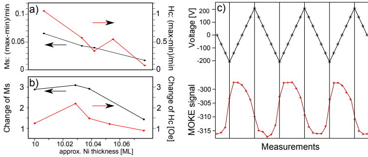
Figure 6.6: Comparison of MEC in Ni films for four different thicknesses close to the SRT: a) relative and b) absolute changes of the coercivity and the saturation magnetization. c) Polar MOKE signal recorded without applied magnetic field as a function of the applied voltage. The thickness of the Ni film is about 10 ML.
