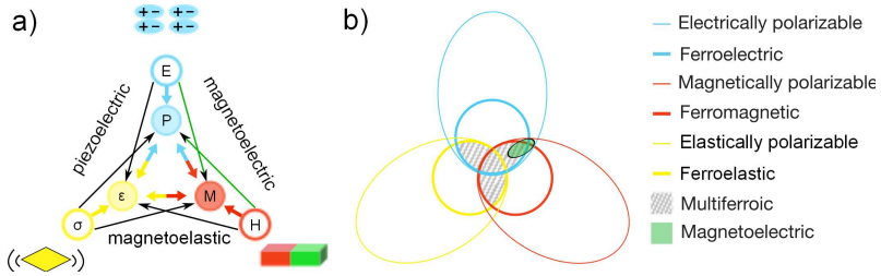
Figure 2.5: a) Interaction triangle of electric field E , stress \sigma , magnetic field H and the corresponding order parameters electric polarization P , elastic deformation \epsilon and magnetization M (after [6]). Particularly interesting is the possible influence of an applied electric field on the magnetization (shown as green arrows). b) Classification of polarizable materials: in multiferroic materials (hatched area), at least two ferroic orders (thick colored circles) coexist; MEC could appear in any material which is both magnetically (thin red circle) and electrically polarizable (blue thin circle), and it is not necessarily limited to ferroic materials (after [26]).
