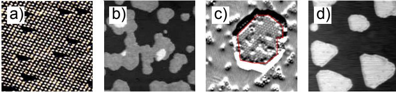
Figure 5.1: a) Atomically resolved STM topography of the bare Ni(111) single crystal surface, 7 \times 7 \text{ nm}^2 . b), d) 60 \times 60 \text{ nm}^2 topography of similar amounts of Fe deposited at about 30^\circ\text{C} . b) Fe/Ni(111) prepared in the normal way, which led to a strongly contaminated surface and irregular island growth. c) \sqrt{2} \times \sqrt{2} superstructure induced by adsorbates on an Fe island (enclosed in red) and on the Ni surface. d) Optimized preparation with reduced surface contamination, for details see text.
