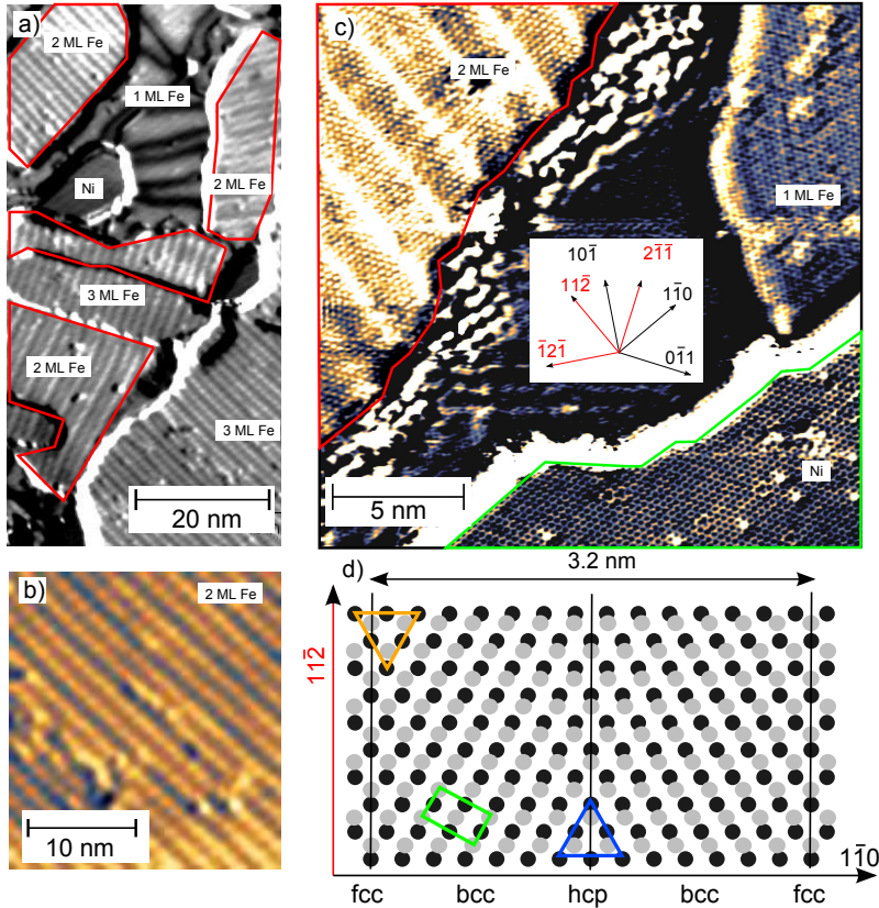
Figure 5.3: a) Fe/Ni(111) films thicker than 1 ML show a stripe pattern perpendicular to the closed-packed \langle 110 \rangle directions. The lattice directions in c) are given for the fcc lattice and hold for all STM images presented. The 2 ML Fe films are enclosed with a red line. b) A dI/dV map at -240 mV shows three different intensities of the stripes. c) dI/dz map on the bare Ni surface (green), 1 ML Fe and 2 ML Fe (red) with atomic resolution. d) Atomic model of 2 ML Fe/Ni(111) for the observed stripe pattern. The relative atomic distances of the top layer (gray circles) are taken from the measurement in c). The expansion of the top layer by 7.5% in the [1\bar{1}0] direction leads to a periodicity of 13 atoms which corresponds to 3.2 nm. The bcc lattice (green rectangle) is characterized by a twofold bridge-stacking (see Fig. 4.1), while the two possible threefold hollow sites correspond to fcc (orange triangle) and hcp domains (blue triangle).
