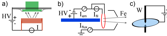
Figure 3.2: a) Sample holder used for heating hat-shaped single crystals (green) by electron bombardment. b) Evaporation of Fe from a rod (blue) by electron bombardment, for details see text. c) Electrochemical etching of a sharp tip from a tungsten wire immersed in a soap film of NaOH.
