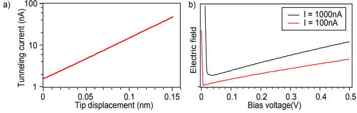
Figure 2.4: a) Measured increase of I as a function of z in order to determine the work function. b) Electric field as a function of applied voltage in the constant current mode for two different tunneling currents following the approximation given in the text.
