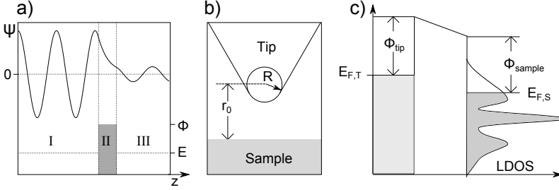
Figure 2.3: a) Real part of the electron wave function and energy for tunneling through a one-dimensional barrier. b) Configuration of tip and sample in the Tersoff-Hamann model. c) Tunneling in the STM setup with a constant tip LDOS: the barrier is formed by the work functions of tip and sample.
