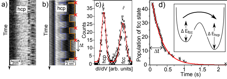
Figure 5.7: a) Switching the domain boundary left and right when scanning across an hcp domain at a constant field of 7.6 \text{ GV/m} ( dI/dU at 3.7 \text{ V} ). b) Switching left by field pulses of 1.4 \text{ GV/m} and right by scanning at 1.0 \text{ GV/m} across an hcp domain (blue) ( dI/dU at -240 \text{ mV} ). c) In a histogram of the differential conductance, only two stable states are found. d) Exponential decay of the hcp state with a lifetime of 0.3 \text{ s} .
