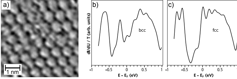
Figure 4.3: a) 3.7 \times 3.7 \text{ nm}^2 high-resolution STM reveals a 2 \times 2 superstructure on the hydrogen-covered Fe island. b) dI/dU spectra on the two phases of a hydrogen-covered Fe island.
