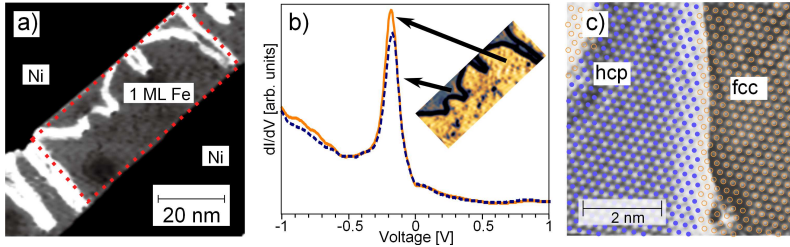
Figure 5.2: Fe/Ni(111): a) STM topography of a 1 ML Fe film (light gray) at a Ni step edge (black). White lines can be seen on the Fe terrace. b) . In a dI/dV map at -130 mV (see inset, position indicated by red rectangle in a)), two different intensities divide the 1 ML Fe terrace into domains. dI/dV spectra outside the domain on the Fe terrace (solid orange) and inside the domain (dashed blue) show different LDOS for the two phases. c) Atomic resolution dl/dz map showing a coexistence of hcp and fcc lattices with light domain walls. The overlaid hexagonal grid is adjusted to the fcc lattice and colored orange on the fcc area and blue on the hcp area.
