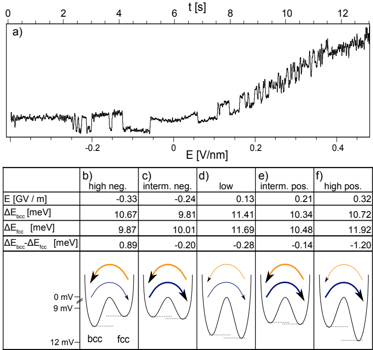
Figure 4.9: Electric field dependence of the switching parameters on the fcc domain close to the domain boundary (later called 'high strain'): a) Typical dI/dU intensity as a function of time and applied electric field. Five different electric field regimes were distinguished, for each of them a more precise measurement of the switching parameters was carried out, shown in b) to f): Energy diagrams for five different electric fields, derived from a total of about 750 transitions. The arrows indicate the different transition probabilities.
