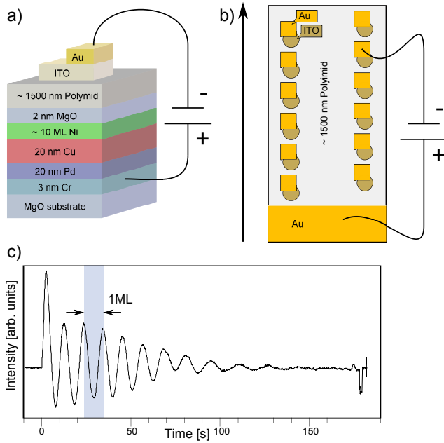
Figure 6.2: a) Stacking of the multilayer grown by MBE and the spin-coated polyimide as it was used for MOKE measurements. b) Top view on the 20 \times 10 mm sample with the thickness of the Ni layer increasing along the arrow. Each Au/ITO junction of 1 \times 1 mm covers a different Ni thickness. c) RHEED oscillations of the growth of Ni/Cu.
