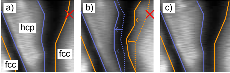
Figure 5.5: Reproducible switching of the crystallographic structure of 1 ML Fe/Ni(111) imaged on 6.25 \times 6.25 \text{ nm}^2 ( dI/dV map at -190 \text{ mV} ). a) The initial hcp domain is indicated by a blue line, the fcc domain by a orange line, domain boundaries appear dark. An electric field pulse is applied on the position marked with the red cross after the acquisition of the image. The new configuration with a smaller hcp domain is imaged in b) with the initial position of the domains indicated by dashed lines. A second pulse brings the system back to the initial state (c).
