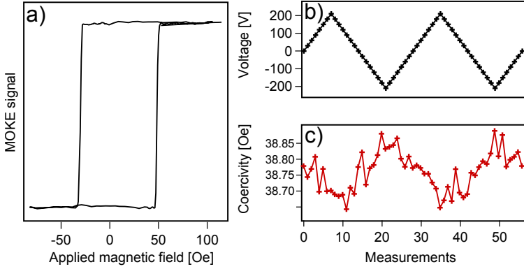
Figure 6.4: Influence of an applied electric field on the coercive field of 13 ML Ni/Cu(100). a) Hysteresis loops are almost identical for all voltages. b), c) The coercivity varies with the applied electric field by about 0.6 %. The coercive field variation is averaged to show two periods of voltage variation.
