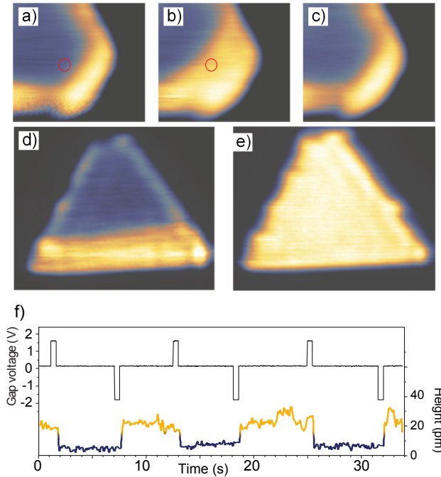
Figure 4.5: a) to c) Three consecutive 6 \times 6 \text{ nm}^2 STM topographies show switching of a small area of about 1 \times 2 \text{ nm}^2 on the edge of an island from AFM fcc (a) to FM bcc (b) and back (c). Electric field pulses of 5.5 \text{ GV/m} were applied on the positions indicated with a red circle. A small island can be switched from dominant fcc (d) to full bcc (e). f) Applied voltage ( \propto E ) and apparent height recorded simultaneously.
