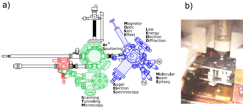
Figure 3.1: a) Vacuum chamber at KIT: preparation chamber with basic surface preparation and analysis tools (blue), STM chamber with He cryostat (green) and two-chamber load lock (red); from [36]. b) View into the STM.
