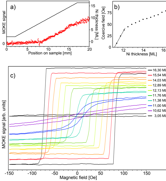
Figure 6.3: a) Cross section of the Ni wedge: thickness calculated from the deposition rate (black line) and saturation magnetization measured with polar MOKE in a magnetic field of 3000 Oe applied perpendicularly to the surface (red crosses). At 7.8 ML, the MOKE signal vanishes. b) Coercive field as a function of the thickness of the Ni layer. c) Hysteresis curves measured with polar MOKE at different Ni thicknesses.
