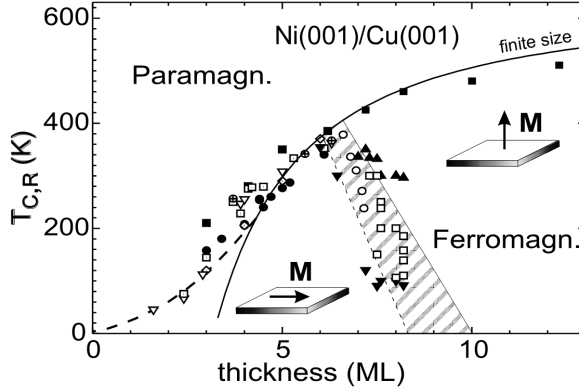
Figure 6.1: Phase diagram of Ni/Cu(100) from [69]
