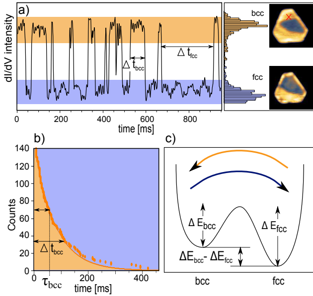
Figure 4.8: Basic experiment to determine the dynamic switching parameters: a) Recorded dI/dU signal at fixed applied electric field and on a fixed position on the island. Examples for residence times \Delta t_{bcc} and \Delta t_{fcc} are indicated. The histogram on the right side shows two different intensities and excludes the possibility of intermediate states. b) Exponential decay of the bcc states into fcc states with a lifetime of \tau_{bcc} = 60 ms. The experimental data (orange dots) can be fitted by a single exponential (orange line). The inset topographies ( 11 \times 11 nm) show the lateral extension of the fcc (blue) and bcc (orange) domains within the island. The position where the dI/dU intensity has been recorded is marked by a red cross. c) Energy diagram of the bistable switching between bcc and fcc.
