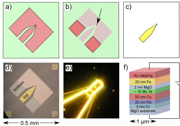
Figure 6.7: a) to c) Three main steps of preparation of an MTJ by lithography. d) Optical microscopy of a single MTJ as prepared by EBL: the gray contacts are connected to the bottom electrode, the contact in the middle (Au, yellow) is bridged to the top of the pillar-shaped TMR junction. e) Dark field microscopy of the pillar (about 1 \mu\text{m}^2 in diameter) covered by the Au bridge. f) Stacking of the MTJ with the Ni wedge as bottom electrode and a 20 nm Fe layer as top electrode. Voltage is applied to the top electrode.
