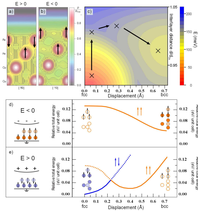
Figure 4.7: Surface relaxations of Fe/Cu(111) in an electric field. a), b) Normalized electronic charge density in 2 ML Fe/Cu(111) under positive (a) and negative (b) electric fields of 1 \text{ GV/m} . The electric field is modeled by a charged counter electrode placed 0.4 \text{ nm} above the surface. The electron charge density is attracted (repelled) by the positively (negatively) charged electrode, causing a vertical compression (expansion) of the Fe bilayer which favors AFM (FM) order. The areas of 0.575 \rho_{max} and 0.6 \rho_{max} are hatched horizontally and vertically, respectively. c) Energy landscape of the top-layer Fe atoms as a function of interlayer distance and lateral displacement shows minimum for the fcc and for the bcc lattice. An electric-field-induced transition from fcc to bcc might follow the path indicated with the black arrows. d), e) Energy landscape for the top-layer Fe atoms as a function of lateral displacement under negative (d) and positive (e) electric fields, simulated for FM (orange) and AFM (blue) order. In a negative (positive) electric field, the lattice adopts the bcc FM (fcc AFM) state and the fcc (bcc) state is unstable. The inset recalls the atomic configuration of fcc and bcc lattices in side and top view. On the left, the corresponding configuration of the STM junction is depicted.
