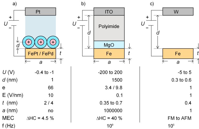
Figure 2.6: Three important experiments on MEC in metallic thin films: a) Change of coercive field in FePd and FePt films by an electric field applied through a double layer in an electrolyte, Weisheit, Givord et al. (2007), b) Large electric-field-induced change of anisotropy in a MgO/Fe junction, Maruyama & Suzuki et al (2009), c) MEC in STM presented in our work (published in 2010). Comparison of characteristic parameters: applied voltage U , thickness of insulator d , dielectric constant \epsilon , electric field E , thickness of the magnetic film t , size of the influenced area a , MEC (change of coercive field in a) and b), transition between FM and AFM in c)) and maximum switching frequency f .
