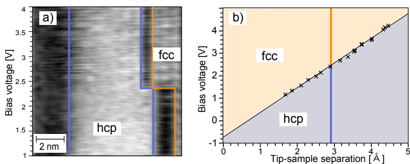
Figure 5.6: Finding the critical parameters for the transition: a) The same line across an hcp domain (blue lines) is repeatedly scanned while the voltage is ramped. Above a certain critical voltage (here 2.3 V), the structure partially changes from hcp to fcc, and the domain boundary (dark) is shifted to the right. Repetition of this measurement at different tip-sample separations results in the phase diagram shown in b). The measurement described in a) corresponds to the dashed blue and the solid orange line giving one data point (black cross). The linear relation between the critical voltage and the tip-sample separation corresponds to a critical electric field of about 10^{\text{GV/m}} .
