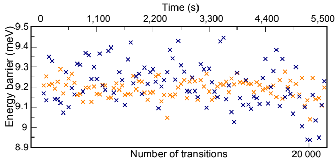
Figure 4.13: Lifetimes of the fcc and the bcc state calculated for repeated switching during 1 h.
