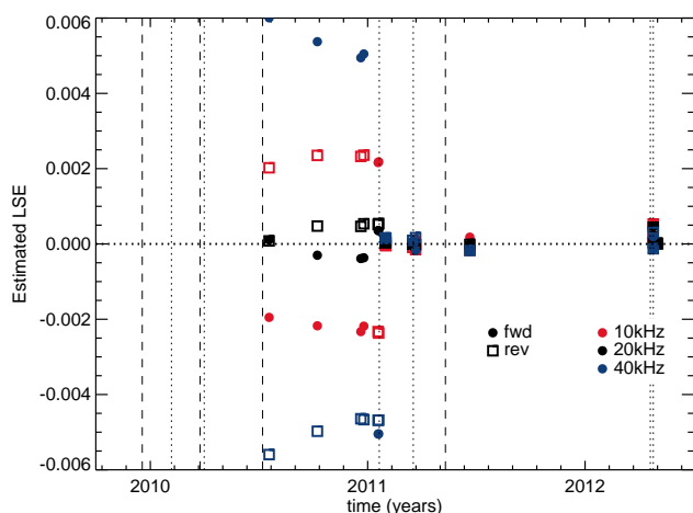
Fig. 5. Lauder 125HR LSE time series determined from analysis of tungsten lamp spectra acquired with narrow bandpass optical filters (NDACC, TCCON) since July 2010. The lamp sequences acquired in January 2011 have been artificially reshuffled for clarity: estimates acquired with the NDACC HF filter appear plotted just prior to 1 January 2011, followed by two realisations with the TCCON filter. The TCCON filter has been used exclusively to monitor the LSE monitoring following the laser board exchange (20 January 2011). Instrument changes are shown with vertical lines (refer to the caption of Fig. 4 for details).
