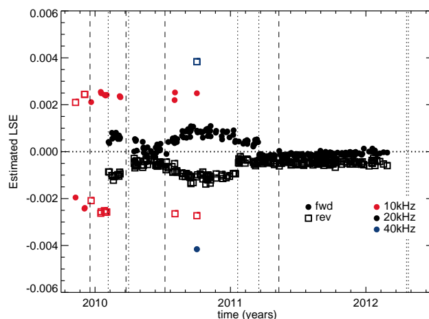
Fig. 4. Lauder 125HR LSE time series determined from resampling analysis of solar interferograms using the 7290\text{--}7360\text{ cm}^{-1} interval. Instrument changes relevant to the LSE and/or its determination are shown with dashed lines: change from 10 to 20 kHz sample rate for routine acquisition (February 2010), increased phase resolution (April 2010), laser board and diodes exchange (January 2011) and reminimisation of laser sampling error at 20 kHz after beam splitter exchange (March 2011). Instrument realignments are shown with dotted lines.
