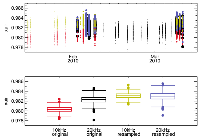
Fig. 8. The upper panel shows Lauder 125HR X_{\text{air}} retrievals from original 10 and 20 kHz data (red and black points respectively), acquired between 18 January and 18 March 2010 at solar zenith angles of 40–60°. The corresponding resampled 10 kHz retrievals are shown in yellow and resampled 20 kHz retrievals are shown in purple. To aid comparison, the lower panel shows box and whisker summaries of the distribution of X_{\text{air}} retrieved at 10 and 20 kHz before and after resampling (these summaries are for the measurement subintervals when both sample rates were used, and are shown with the larger sized symbols in the upper panel). There is clear evidence of a low bias of 0.2 % in the original 10 kHz X_{\text{air}} retrievals, relative to the 20 kHz retrievals. After resampling, the distribution of X_{\text{air}} retrieved at 10 kHz lies entirely within the range of the 20 kHz X_{\text{air}} distribution, and central 50 % of two distributions (the boxes) are essentially co-incident (the medians differ by 0.01 % and the lower fourths differ by 0.03 %).
