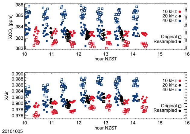
Fig. 7. Cycling sample rate experiments undertaken on the Lauder 125HR with the ECL03 version of the laser board on 5 October 2010. Retrievals from original interferograms are illustrated with squares for three sample rates 10 kHz (red), 20 kHz (black) and 40 kHz (blue) showing a marked sample rate dependence. Retrievals from resampled interferograms are shown with filled circles. Resampling reduces discrepancies between the sample rates to less than 0.1 %.
