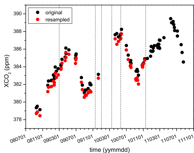
Fig. 10. Izaña 125HR time series of daily mean X_{\text{CO}_2} from 2008 to 2011 for original and resampled measurements. The beginning of new sub-periods with different X_{\text{air}} due to instrumental interventions or breakdowns are indicated with vertical dashed lines: electrical low-pass-filter change (March 2009), laser board exchange and red-filter installation (November/December 2009), loss of power and very cold temperatures (January–March 2010), electrical low-pass-filter change (May 2010), installation of ECL04 laser board and v02 diodes (November 2010). The plot indicates a reduction of X_{\text{CO}_2} for resampled measurements, which is mostly due to changes in the \text{O}_2 retrieval.
