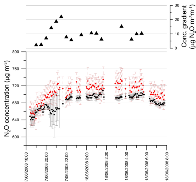
Fig. 10. Temporal variation of the N 2 O concentrations in ambient air (17–18 June 2008) at both heights (0.5 m: edge-oriented squares, 2.7 m: side-oriented squares) including the statistical errors (random absolute error as columns around the measurement value in both directions) and concentration gradients.
