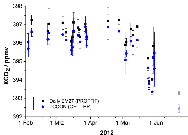
Fig. 9. Daily means of XCO 2 values of the EM27 and the TCCON instrument. The last day is preliminary only.
