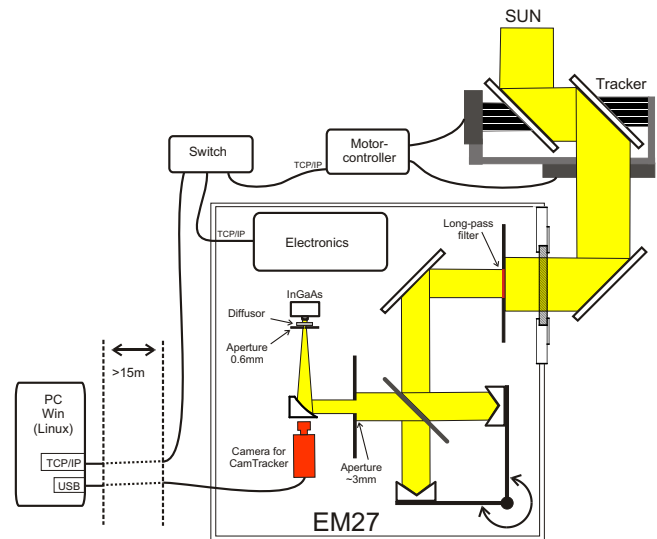
Fig. 3. Schematic drawing of our measurement setup and the EM27 spectrometer. The camera is not in the same plane as the mirror, instead it observes the field stop by a small angle from above.
