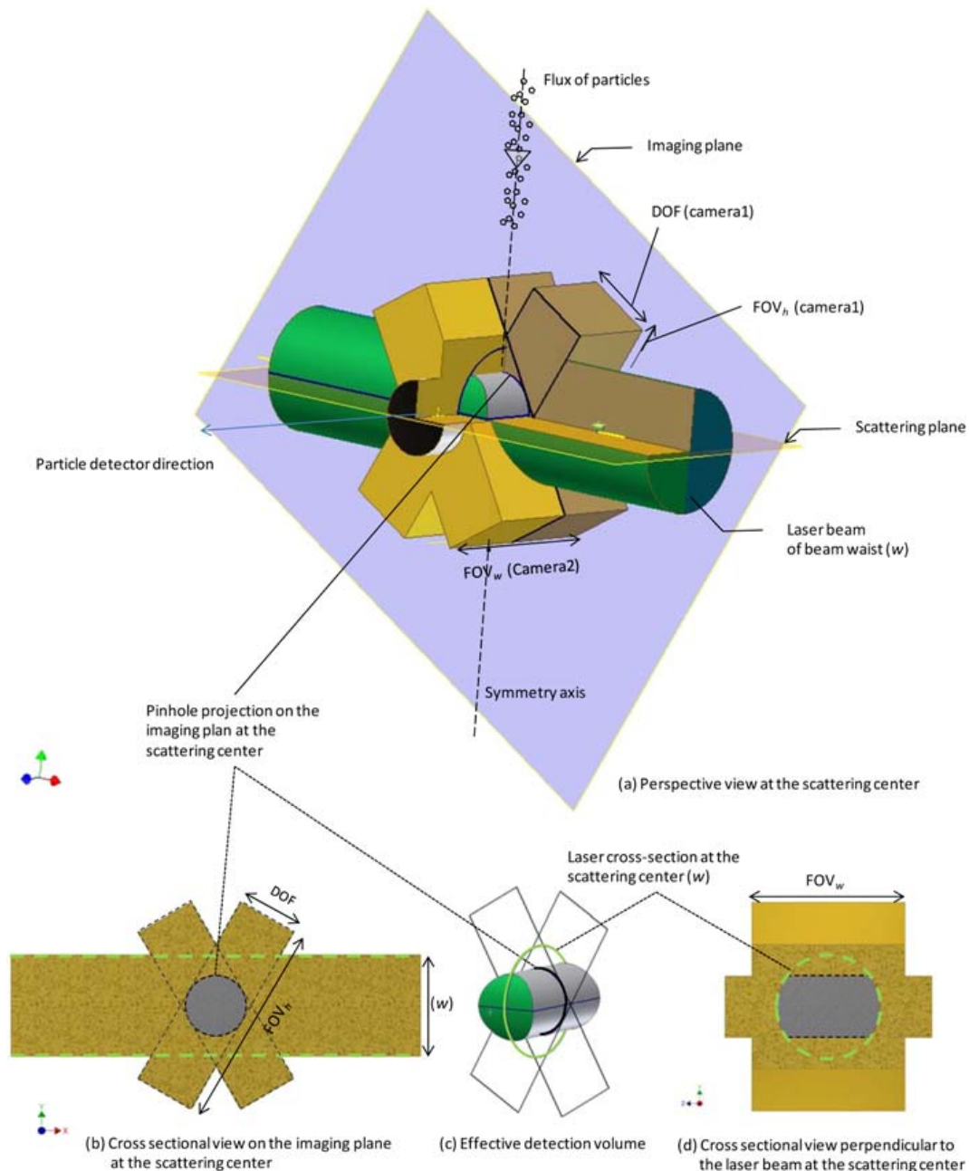
Fig. 2. The intersection of the laser beam, the FOV \times DOF and the projection of the pinhole (placed in the particle detector optics) at the scattering center. (a) A perspective view, (b) a cross sectional view of on the imaging plane at the scattering center, (d) a cross sectional view perpendicular to the laser beam at the scattering center, and (c) the effective detection volume of PHIPS. DOF: Depth-of-field, FOV_h : Field-of-view height, and FOV_w : Field-of-view width. DOF (camera2), FOV_h (camera2) and FOV_w (camera1) are not indicated on the drawing for clarity.
