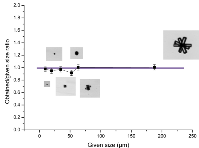
Fig. 6. The ratio of the evaluated particle sizes (using the developed inflection point algorithm) to those given as standard values for standard ice analogues.
