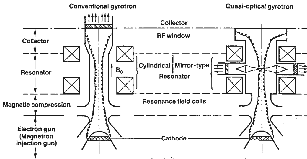
Fig. 2: Principle of a conventional gyrotron with cylindrical resonator and of a quasi-optical gyrotron with mirror resonator [77,78].
