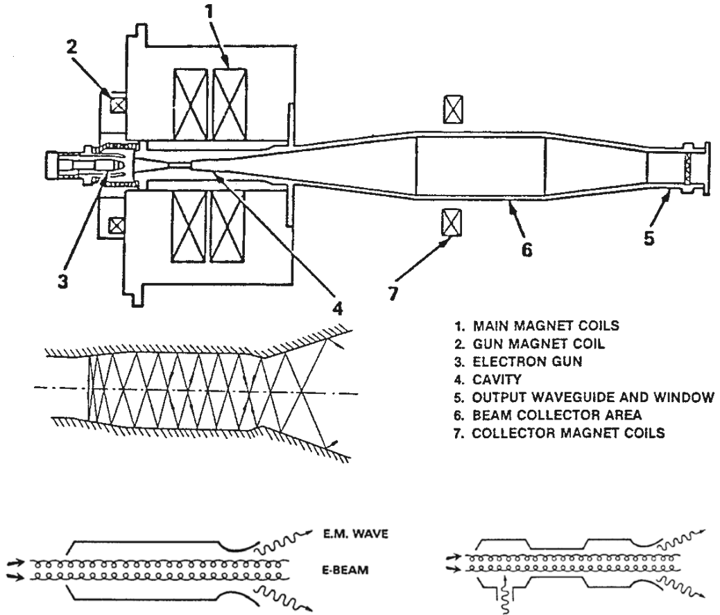
Fig. 1: Schematic of VARIAN CW gyrotron oscillator [14,19] and scheme of irregular waveguide cavities of gyromonotron oscillator (left) and two-cavity gyrokystron amplifier [274,275].
