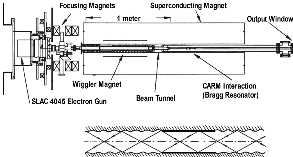
Fig. 7: Schematic of the long-pulse MIT CARM oscillator experiment [290] and scheme of a Bragg resonator [259].
