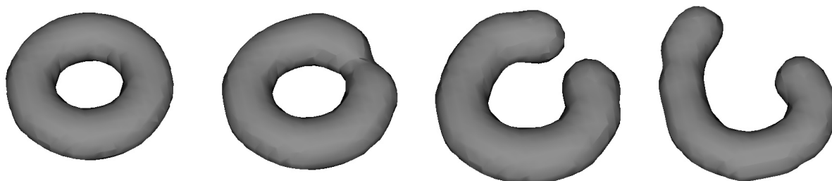
Figure 7. Sequence of shapes for the rotating torus when an external potential causes a break-up. The external potential acts at the right-hand side of the torus.
