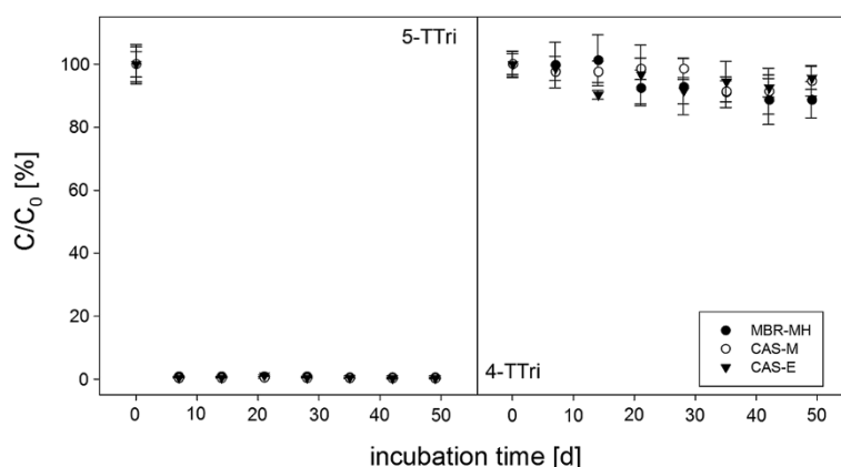
Figure 1 Biodegradation behavior of aerobic 4- and 5-TTri. Aerobic 5-TTri biodegradation behavior in the three ASC (initial concentration is given in Table 2). Shown are mean values of 5-TTri concentrations of duplicate experiments with error bars indicating standard deviations ( n = 2 ). Aerobic 4-TTri biodegradation behavior in the three ASC (initial concentration is given in Table 2). Shown are mean values of 4-TTri concentrations of duplicate experiments. MBR, membrane bioreactor; CAS, conventional activated sludge treatment.
