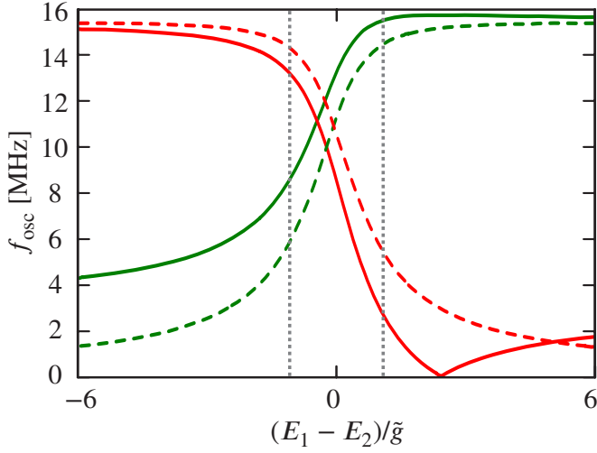
Figure 5.20: The calculated coupling strength in terms of \tilde{g} between the qubit and both branches with v_{2,\perp} = 0 (dashed) and v_{2,\perp} = 3 MHz (solid) ( v_{1,\perp} = 15.4 MHz). The region between the dotted lines corresponds to the measured range assuming that \tilde{g} = g_{\perp} . As can be recognized, at some TLS1-TLS2 detuning the qubit-upper branch coupling equals zero.
