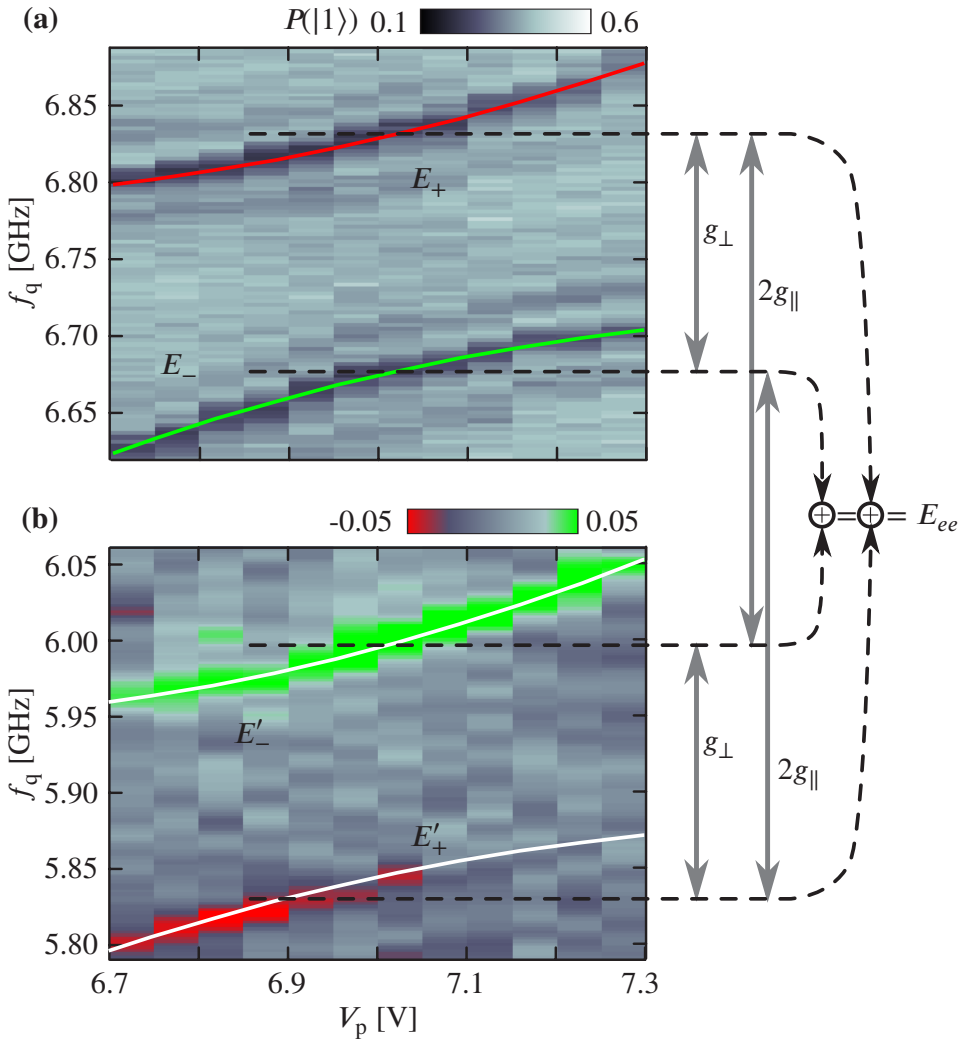
Figure 5.15: Some relevant parameters can be estimated directly from the right TLS1-TLS2 anti-crossing (a) and the corresponding energies to fully excite the TLS1-TLS2 system (b). The size of the anti-crossings equals g_\perp while the energetical difference between them corresponds to 2g_\parallel . Adding up the energies as shown by black arrows results in E_{ee} which equals twice the unperturbed TLS energies E_i .
