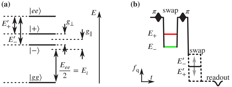
Figure 5.13: (a) The level structure at the right TLS1-TLS2 anti-crossing is shown. Measuring the frequencies E'_\pm = E_{ee} - E_\pm allows to determine the energies of the unperturbed TLSs E_1 and E_2 and the coupling strengths g_\perp and g_\parallel directly. (b) The pulse sequence to measure E_{ee} is shown schematically. After exciting the qubit, its excitation is swapped to one of the |\pm\rangle states. Afterwards, the SPS protocol should reveal the energies E'_\pm .
