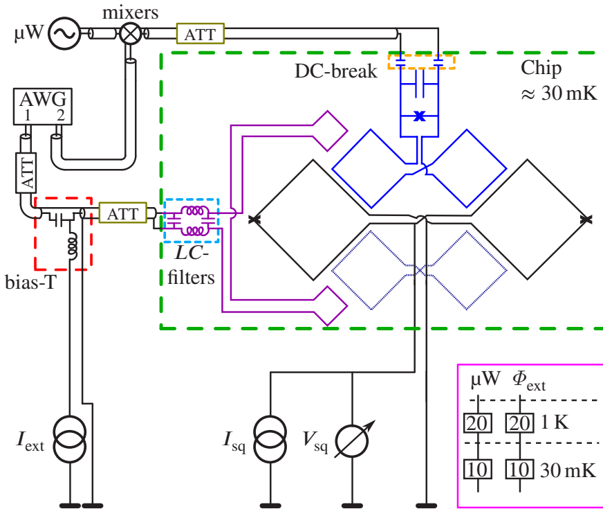
Figure 3.4: Sketch of the experimental setup. The green dashed box symbolizes the chip at a temperature of \approx 30\text{ mK} . The qubit is controlled by microwaves, which are pulsed by using a continuous microwave source ( \mu\text{W} ) and two mixers in series connected to a channel of our AWG, and by the external flux bias which is partially also controlled by our AWG. The microwave and the flux bias coaxial lines have attenuators at the 1 K ( -20\text{ dB} ) and 30 mK ( -10\text{ dB} ) levels as sketched in the purple box. The readout is performed by measuring the switching current of the dc-SQUID. At the 1 K level a current divider (factor 50) and a low pass filter (cut off at 100 kHz) are installed.
