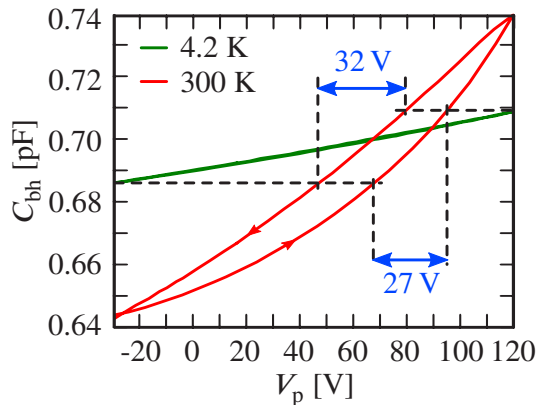
Figure 5.2: The calibration of the piezo actuator at 4.2 K. Measuring and comparing the voltage ranges for corresponding capacitances formed by the gold plated ball and the housing yields a reduction factor of \approx 5 of the piezo constant between room and liquid helium temperature.
