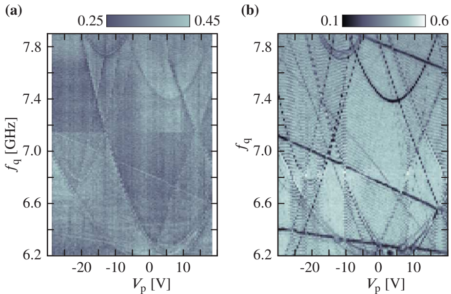
Figure 5.9: A comparison between the two spectra taken according to MPS (a) and SPS (b) . SPS is not only much more precise and has a much higher contrast, but it also only takes approximately one third of the time needed for MPS.
