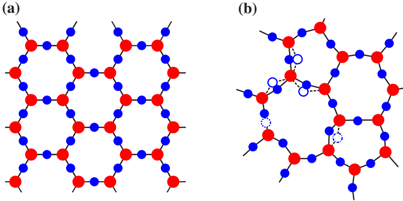
Figure 4.2: (a) A crystalline structure of SiO 2 is shown, with silicon atoms colored in red and oxygen in blue. (b) An amorphous glass might have not only “simple” defects, but also atoms, or a small group of atoms, having two stable positions with a nonzero tunneling probability between them. Nevertheless, the stoichiometric coefficients have to stay constant. (Picture taken from [Hun07])
