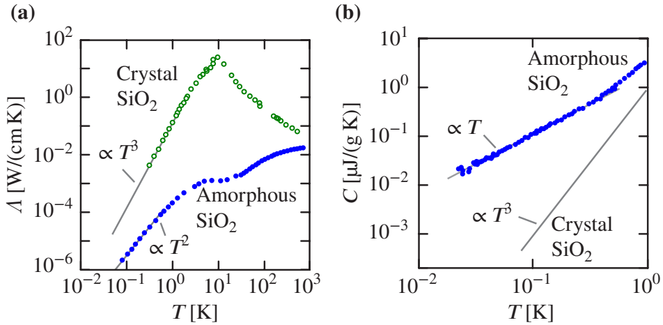
Figure 4.1: According to the Debye model, the thermal conductivity \Lambda (a) and the heat capacity C (b) of solids at low temperatures scales as T^3 . Point-like defects, due to the long phonon wavelengths, should not play a role. Zeller and Pohl [ZP71] (a) showed the first clear discrepancy between the Debye model and the characteristics of amorphous solids, which, among others, was also confirmed by [Las+75].
