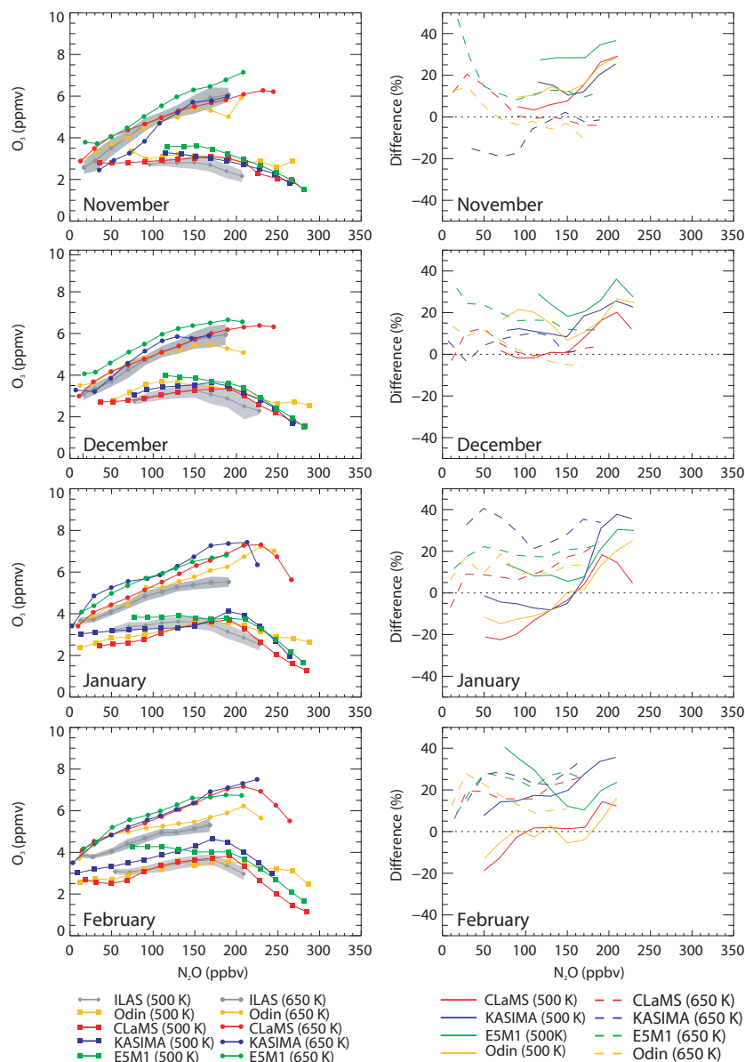
Fig. 8. As Fig. 7, but using ILAS/ILAS-II as the reference (Northern Hemisphere polar regions). Left: Comparison of monthly averages of \text{N}_2\text{O} and \text{O}_3 derived from CLaMS, KASIMA, E5M1 and Odin/SMR (colored curves) with ILAS/ILAS-II (grey) at 500 \pm 25 K (squares) and 650 \pm 25 K (circles). The grey shaded area marks the range of the standard deviations of the monthly averages of \text{O}_3 derived from ILAS/ILAS-II. Right: Differences in percentage of the \text{O}_3 averages of CLaMS, KASIMA, E5M1, and Odin/SMR from ILAS/ILAS-II at 500 \pm 25 K (solid curves) and 650 \pm 25 K (dashed curves). A positive difference means an overestimation of ozone while a negative difference means an underestimation of ozone.
