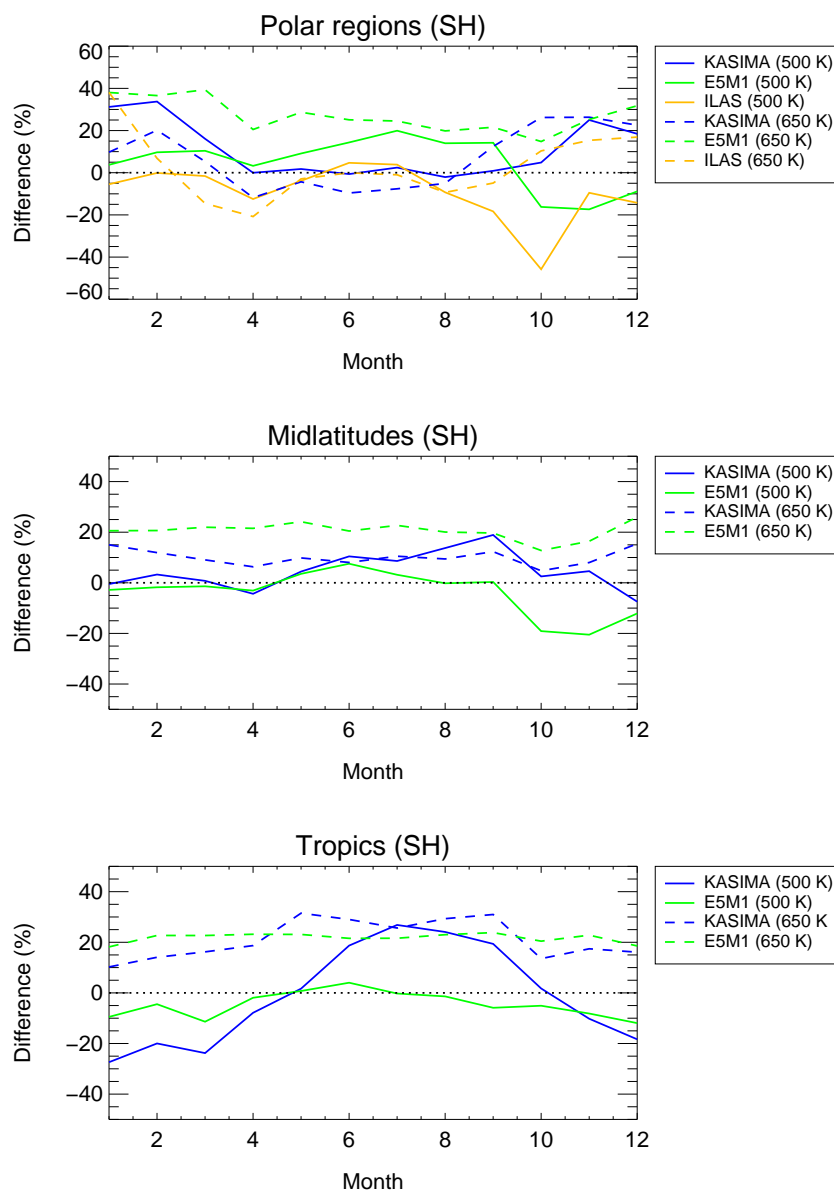
Fig. 11. The averaged differences in percentage between the monthly averaged \text{O}_3 mixing ratios derived from the model simulations of KASIMA (blue) and E5M1 (green) and ILAS/ILAS-II (yellow) measurements, respectively, from the monthly averaged \text{O}_3 mixing ratios derived from Odin/SMR measurements at 500 \pm 25 K (solid curves) and 650 \pm 25 K (dashed curves) are shown for every month of the year and separated by latitude region (Southern Hemisphere).
