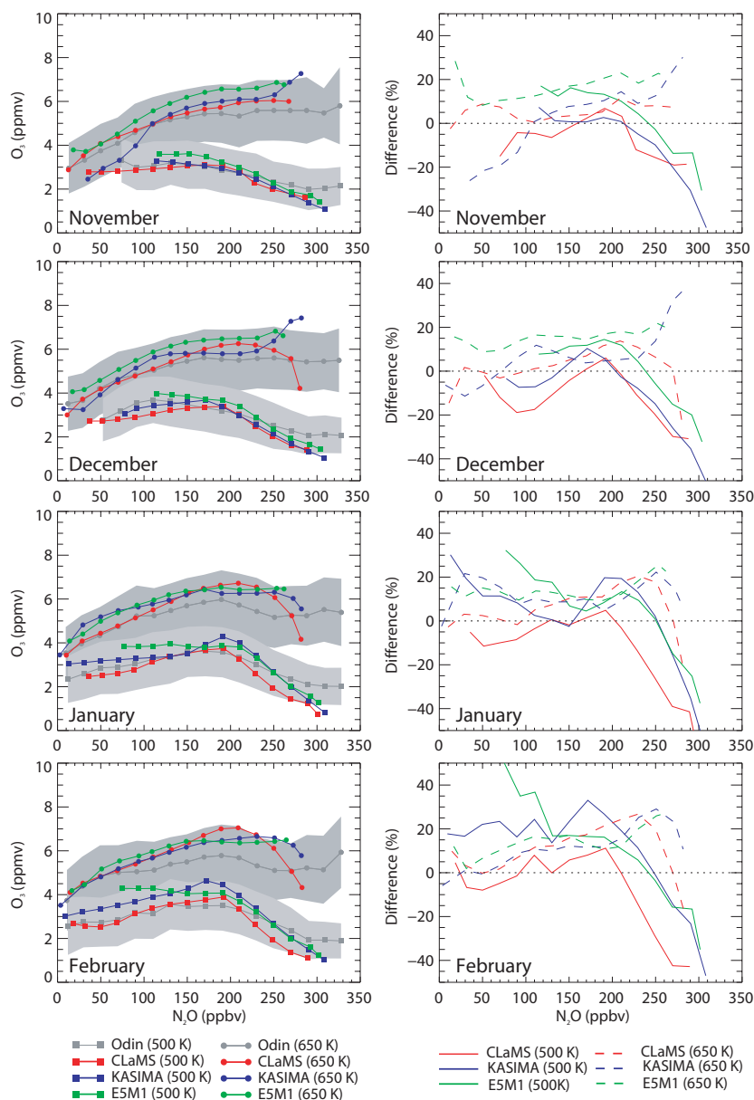
Fig. 4. Northern Hemisphere, all latitudes. Left: Comparison of monthly averages of \text{N}_2\text{O} and \text{O}_3 derived from CLaMS, KASIMA and E5M1 (colored curves) with Odin/SMR (grey) at 500\pm 25 K (squares) and 650\pm 25 K (circles). The grey shaded area marks the range of the standard deviations of the monthly averages of \text{O}_3 derived from Odin/SMR. Right: Differences in percentage of the \text{O}_3 averages of CLaMS, KASIMA and E5M1 from Odin/SMR at 500\pm 25 K (solid curves) and 650\pm 25 K (dashed curves). A positive difference means an overestimation of ozone while a negative difference means an underestimation of ozone.
