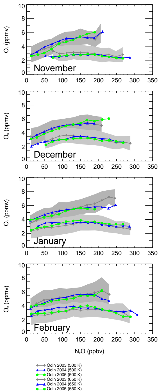
Fig. 2. Comparison of monthly averages of N_2O and O_3 derived from Odin/SMR for the years 2004 (blue triangles) and 2005 (green circles) with monthly averages of N_2O and O_3 derived from Odin/SMR for the year 2003 (grey diamonds) at 500\pm 25 K and 650\pm 25 K (Northern Hemisphere polar regions). The grey shaded area marks the range of the standard deviations of the monthly averages of O_3 derived from Odin/SMR data for the year 2003. Here and in the following figures the N_2O data is binned by 20 ppbv N_2O .
