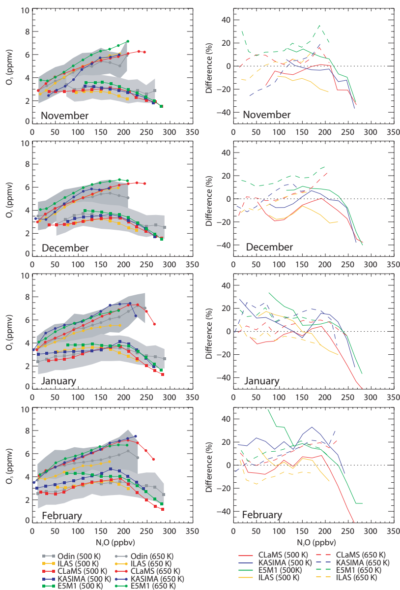
Fig. 7. Northern Hemisphere, polar regions. Left: Comparison of monthly averages of \text{N}_2\text{O} and \text{O}_3 derived from CLaMS, KASIMA, E5M1 and ILAS/ILAS-II (colored curves) with Odin/SMR (grey) at 500\pm 25 K (squares) and 650\pm 25 K (circles). The grey shaded area marks the range of the standard deviations of the monthly averages of \text{O}_3 derived from Odin/SMR. Right: Differences in percentage of the \text{O}_3 averages of CLaMS, KASIMA, E5M1 and ILAS/ILAS-II from Odin/SMR at 500\pm 25 K (solid curves) and 650\pm 25 K (dashed curves). A positive difference means an overestimation of ozone while a negative difference means an underestimation of ozone.
