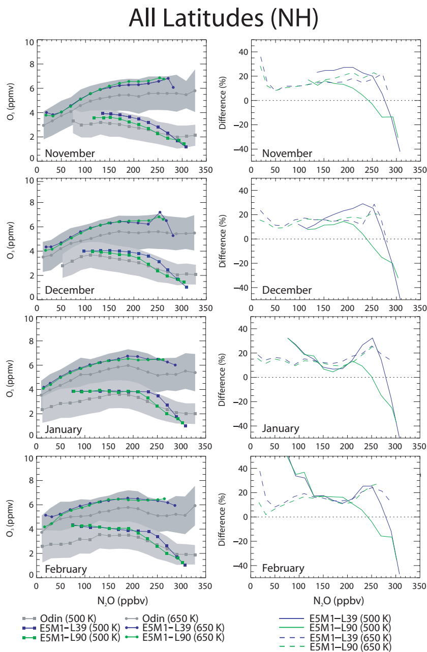
Fig. 9. As Figure 4, but showing (left) the impact of different vertical resolutions (Northern Hemisphere). Left: The comparison of monthly averages of \text{N}_2\text{O} and \text{O}_3 derived from E5M1 T42L90MA and E5M1 T42L39MA simulation (colored curves) with Odin/SMR (grey) at 500\pm 25 K (squares) and 650\pm 25 K (circles). The grey shaded area marks the range of the standard deviations of the monthly averages of \text{O}_3 derived from Odin/SMR. Right: Differences in percentage of the \text{O}_3 averages of E5M1 T42L90MA and E5M1 T42L39MA simulation from Odin/SMR at 500\pm 25 K (solid curves) and 650\pm 25 K (dashed curves). A positive difference means an overestimation of ozone while a negative difference means an underestimation of ozone.
