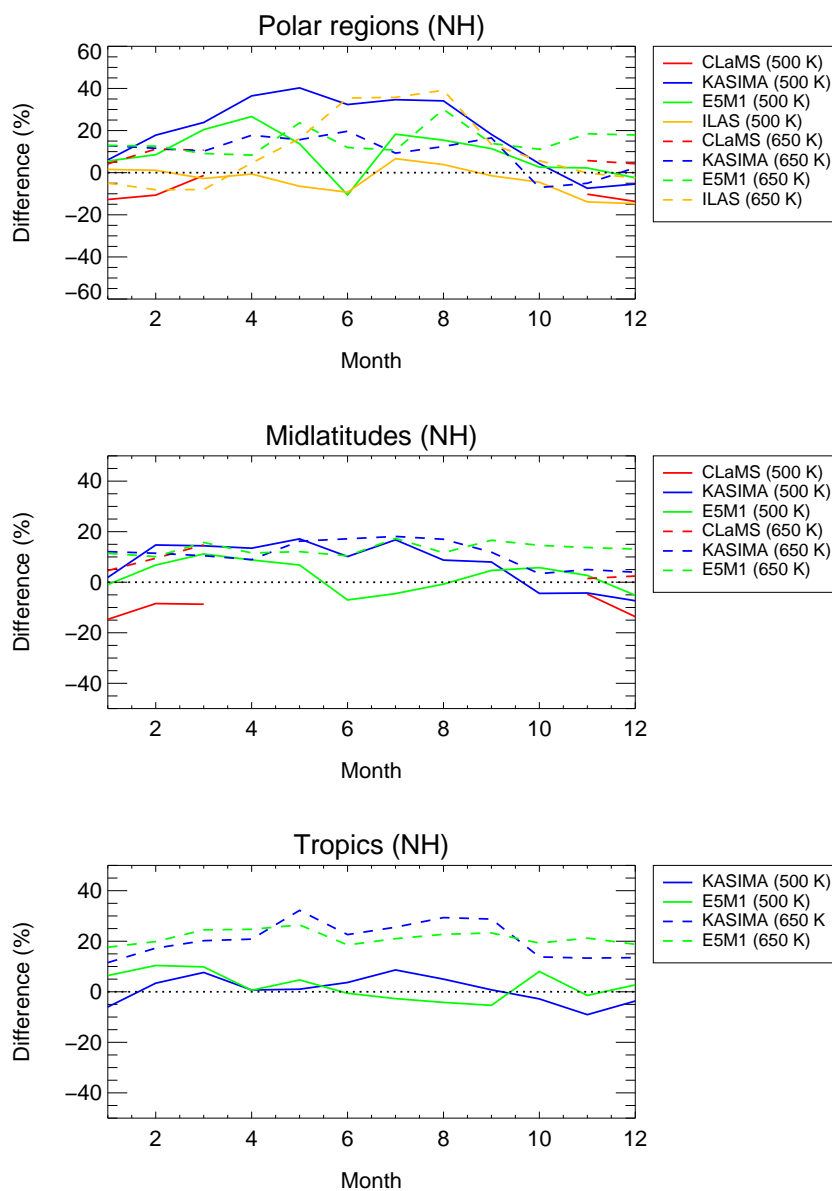
Fig. 10. The averaged differences in percentage between the monthly averaged O_3 mixing ratios derived from the model simulations of CLaMS (red), KASIMA (blue), E5M1 (green) and ILAS/ILAS-II (yellow) measurements, respectively, from the monthly averaged O_3 mixing ratios derived from Odin/SMR at 500 \pm 25 K (solid curves) and 650 \pm 25 K (dashed curves) are shown for every month of the year and separated by latitude region (Northern Hemisphere).
