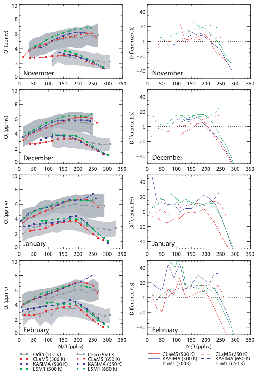
Fig. 6. Northern Hemisphere, midlatitudes. Left: Comparison of monthly averages of \text{N}_2\text{O} and \text{O}_3 derived from CLaMS, KASIMA and E5M1 (colored curves) with Odin/SMR (grey) at 500\pm 25 K (squares) and 650\pm 25 K (circles). The grey shaded area marks the range of the standard deviations of the monthly averages of \text{O}_3 derived from Odin/SMR. Right: Differences in percentage of the \text{O}_3 averages of CLaMS, KASIMA and E5M1 from Odin/SMR at 500\pm 25 K (solid curves) and 650\pm 25 K (dashed curves). A positive difference means an overestimation of ozone while a negative difference means an underestimation of ozone.
