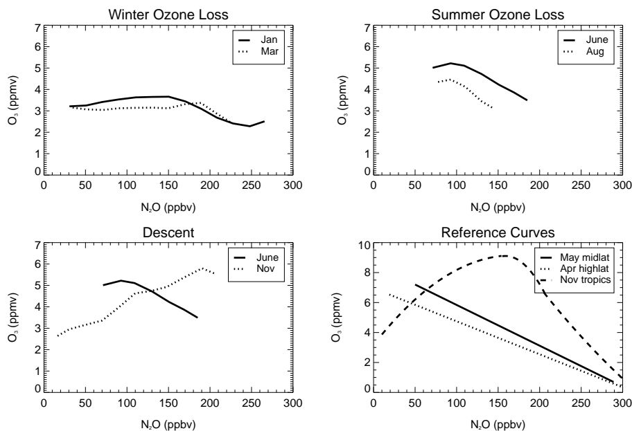
Fig. 1. Schematic of the change of the N 2 O and O 3 distribution in the Northern Hemisphere polar region due to photochemical winter ozone loss at a selected altitude level of 20 \pm 2.5 km which agrees with \approx 450 K (top:left) and photochemical summer ozone loss at a selected altitude level of 25 \pm 2.5 km which agrees with \approx 550 K (top:right) and diabatic descent at a selected altitude level of 25 \pm 2.5 km which agrees with \approx 550 K (bottom:left) based on ILAS/ILAS-II data as well as reference curves (bottom:right) for the midlatitudes (May, ATMOS Shuttle 1985, solid line), highlatitudes (April, ATMOS Shuttle 1993, dotted line) and tropics (November, ATMOS Shuttle 1994, dashed curve) based on ATMOS shuttle measurements. These reference curves were derived from measurements made in the altitude region from 12–80 km. Note, while the curves in Fig. a–c are for a certain altitude level, the reference curves in Fig. d are derived from all measurements made at a certain latitude region. See text for further details.
