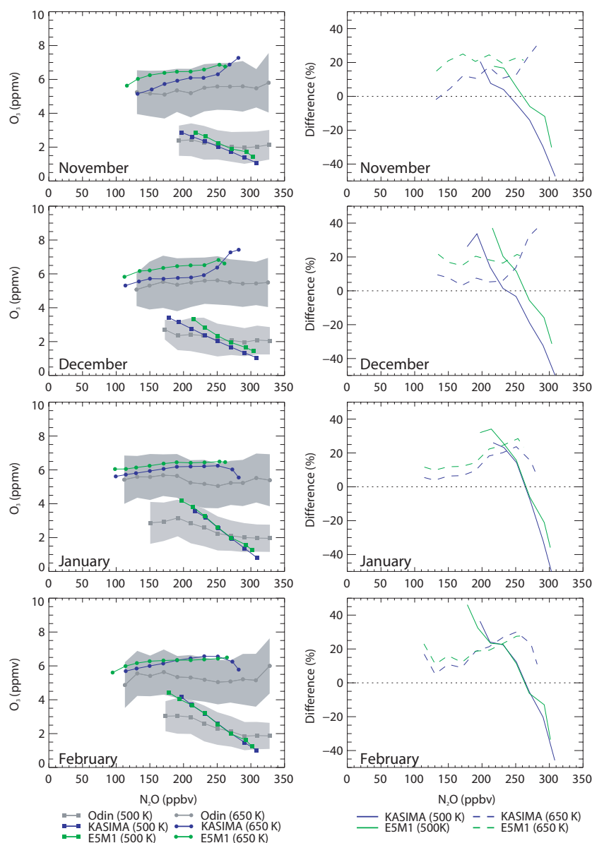
Fig. 5. Northern Hemisphere, tropics. Left: Comparison of monthly averages of N_2O and O_3 derived from KASIMA and E5M1 (colored curves) with Odin/SMR (grey) at 500\pm 25 K (squares) and 650\pm 25 K (circles). The grey shaded area marks the range of the standard deviations of the monthly averages of O_3 derived from Odin/SMR. Right: Differences in percentage of the O_3 averages of KASIMA and E5M1 from Odin/SMR at 500\pm 25 K (solid curves) and 650\pm 25 K (dashed curves). A positive difference means an overestimation of ozone while a negative difference means an underestimation of ozone.
