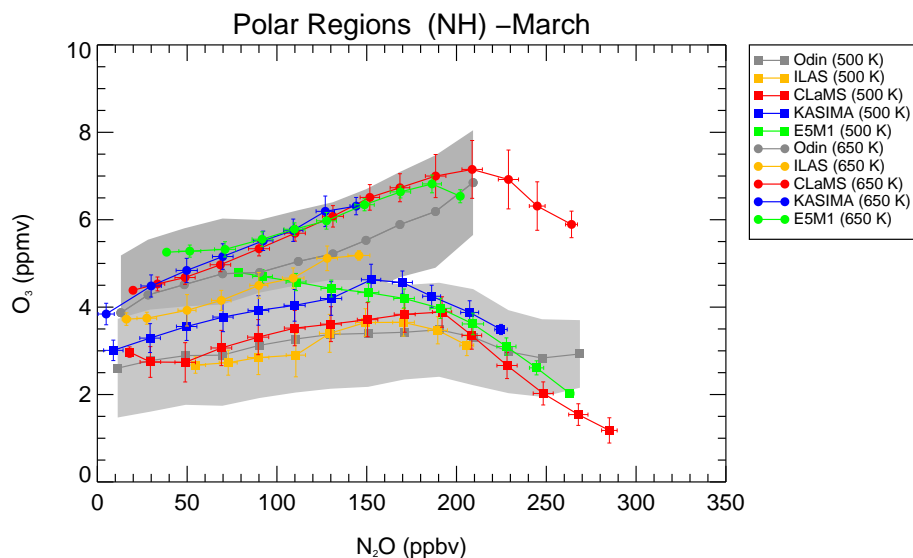
Fig. 3. Monthly averages of \text{N}_2\text{O} and \text{O}_3 derived from CLaMS, KASIMA, E5M1, ILAS/ILAS-II (colored curves) and Odin/SMR (grey) at 500\pm 25 K (squares) and 650\pm 25 K (circles) for the Northern Hemisphere (March). The grey shaded area marks the range of the standard deviations of the monthly averages of \text{O}_3 derived from Odin/SMR. Standard deviations of the models and ILAS/ILAS-II are given as error bars.
