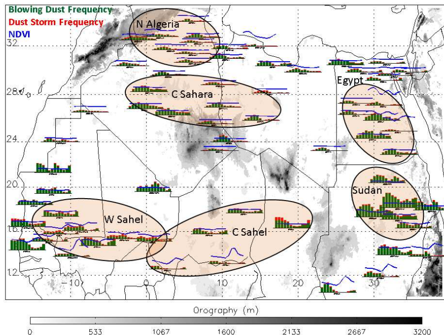
Fig. 7. Mean seasonal cycle. Monthly mean FDE, split into BDF (green bars) and DSF (red bars) (for definitions, see Sect. 2.1.1), as well as monthly mean NDVI (blue lines) calculated for a 24 km × 24 km box centred on each station. The x axis runs from January to December. The y axis scale is 0–40 % for FDE and 0–5000 for NDVI. Areas of grouped stations, discussed in Sect. 3.2.1, are shown with shaded black ellipses and labels.
