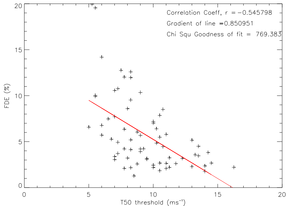
Fig. 6. Scatter of annual mean frequency of dust events (FDE) against annual mean T50 (for definition, see Sect. 2.2.1) for each of the 70 individual stations for the period 1984–2012. Correlation coefficient, gradient of best-fit line and goodness of fit test are given in the top right corner.
