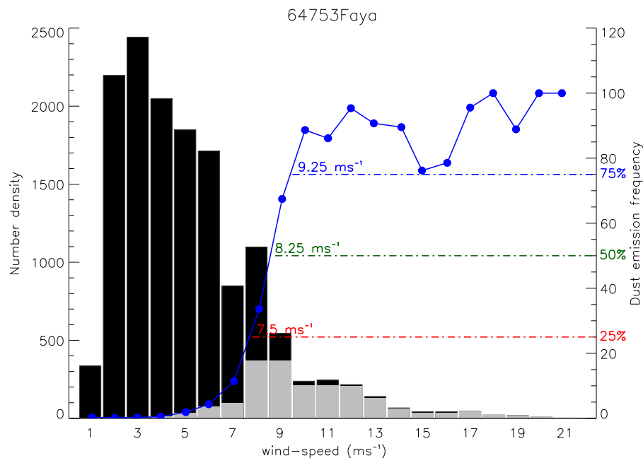
Fig. 3. Example wind climatology for Faya (WMO no. 64753) in Chad (see Fig. 1 for location). Number distribution of surface wind-speed for the time period 1984–2012. Black bars and grey bars give the distribution of all winds and those associated with dust emission only, respectively. Dust emission frequency ( (\text{grey/black}) \cdot 100 ) for each wind-speed bin is given by the blue dots. T25, T50 and T75 threshold values are given in red, green and blue, respectively.
