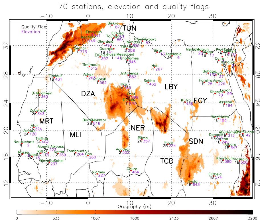
Fig. 1. Geographical overview. Map of observation stations used in the study, with quality flags in black (see Sect. 2.1.1) and elevation in purple. Country codes, as defined by ISO (International Organization for Standardization): DZA = Algeria, TUN = Tunisia, MRT = Mauritania, MLI = Mali, NER = Niger, LBY = Libya, EGY = Egypt, TCD = Chad and SDN = Sudan. Colour shading gives the orography in m.
