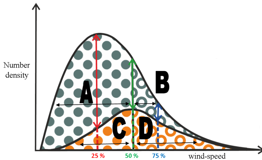
Fig. 2. Schematic to illustrate the estimation of emission thresholds. Orange shading indicates the number density function of wind-speeds associated with dust emission reports and grey shading represents wind-speeds for all observations. The arrows signify the wind-speed at which dust emissions make up 25, 50 and 75 % (red, green and blue respectively) of all reports. Areas A and B are represented by grey dots and circles, C and D with orange dots and circles. For a detailed discussion of this schematic, see Sect. 2.2.1.
