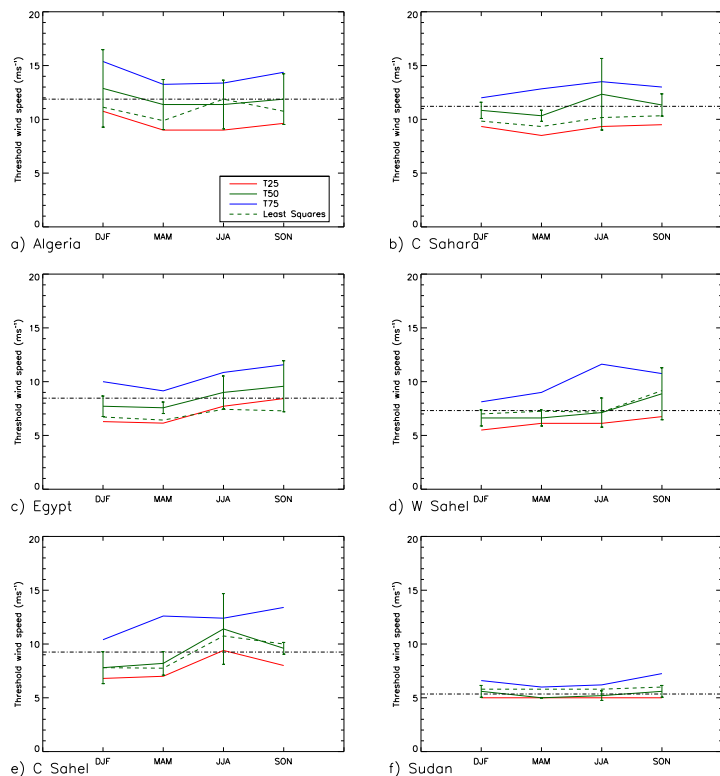
Fig. 8. Seasonal threshold values averaged over six station groups (see Sect. 3.2.1 for definition): (a) N Algeria, (b) C Sahara, (c) Egypt, (d) W Sahel, (e) C Sahel and (f) Sudan according to the legend in the top left panel (for definition of thresholds, see Sect. 2.2.1). The dashed black lines indicate the annual mean T50. Seasons are December, January, February (DJF), March, April, May (MAM), June, July, August (JJA) and September, October, November (SON).
