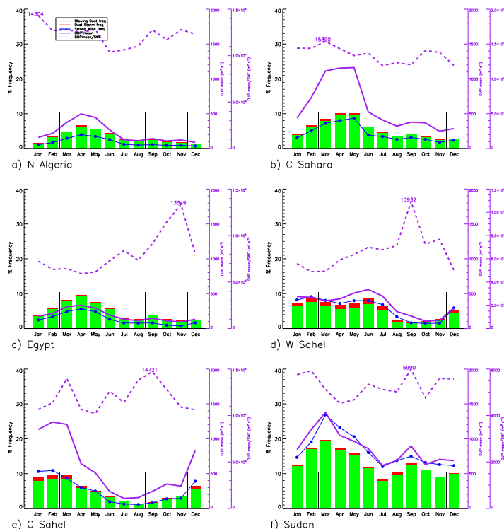
Fig. 9. Mean seasonal cycle for the six station groups (see Sect. 3.2.1 for definitions): (a) N Algeria, (b) C Sahara, (c) Egypt, (d) W Sahel, (e) C Sahel and (f) Sudan. Monthly frequency of FDE, split into BDF (green bars) and DSF (red bars), as well as SWF (blue line), DUP mean (solid purple) and DUP Intensity (DUP mean/SWF, dashed purple, maximum values given), all computed using the seasonally varying T50 (for definitions of parameters, see Sect. 2.2.1). Thin vertical black lines indicate seasonal boundaries where thresholds change. Note the different vertical axes for DUP intensity.
