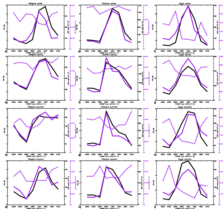
Fig. 11. Diurnal cycles of FDE (solid black), DUP mean (solid purple) and DUP Intensity (dashed purple) for N Algeria (column 1), C Sahara (column 2) and Egypt (column 3) for DJF (row 1), MAM (row 2), JJA (row 3) and SON (row 4) (see Sect. 3.2.1 for definition of regions). For definitions of parameters, see Sect. 2.1.1.
