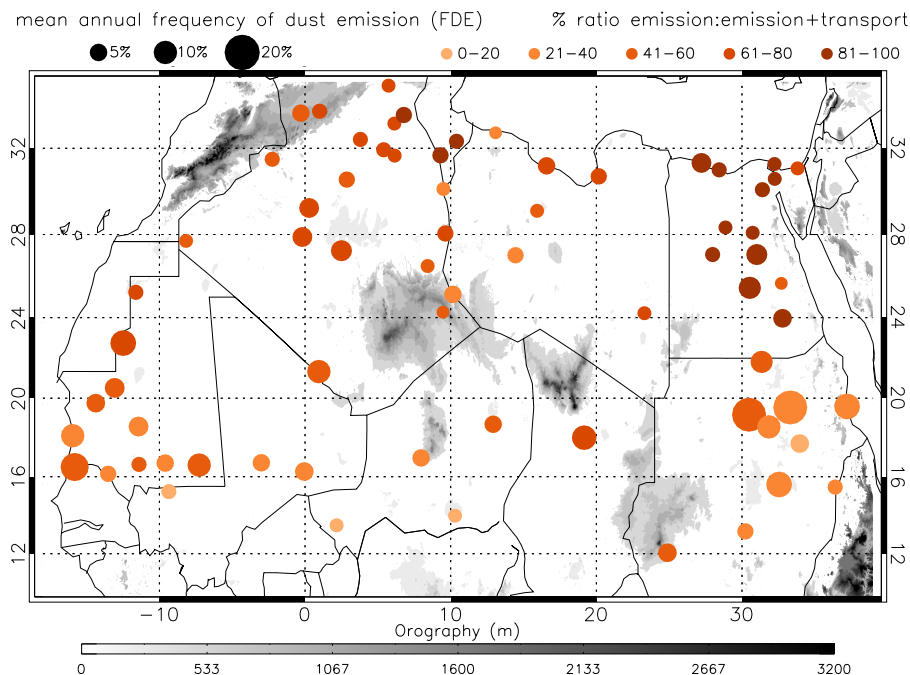
Fig. 4. Annual emission climatology. Spatial distribution of mean annual FDE (dot size) and % ratio of emission to all dust events (including transported events) (dot colour) at 70 stations in northern Africa for the time period 1984–2012.
