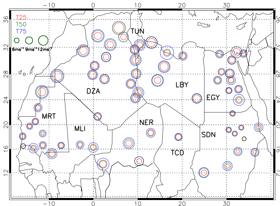
Fig. 5. Geographical distribution of emission thresholds. Shown are annual values of T25, T50 and T75 (for definitions, see Sect. 2.2.1) in red, green and blue, respectively. Country codes, as defined by ISO (International Organization for Standardization): DZA = Algeria, TUN = Tunisia, MRT = Mauritania, MLI = Mali, NER = Niger, LBY = Libya, EGY = Egypt, TCD = Chad and SDN = Sudan.
