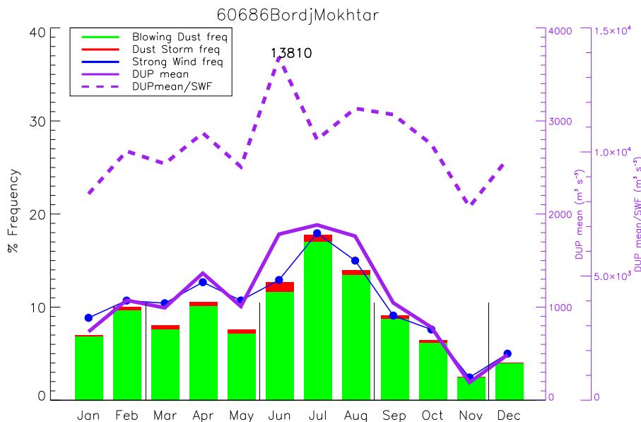
Fig. 10. As Fig. 9 but for Bordj Mokhtar (WMO number 60686).
