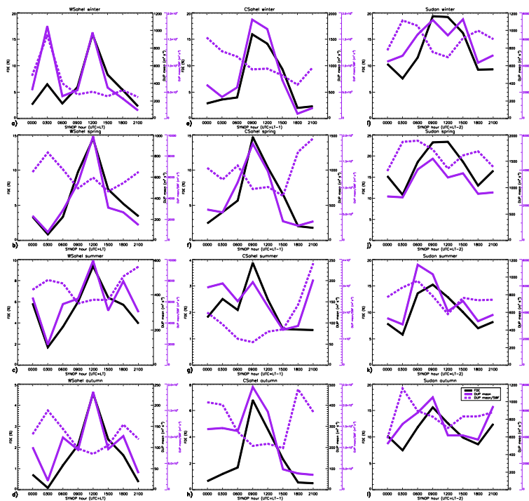
Fig. 12. As Fig. 11 but for W Sahel (column 1), C Sahel (column 2) and Sudan (column 3).
