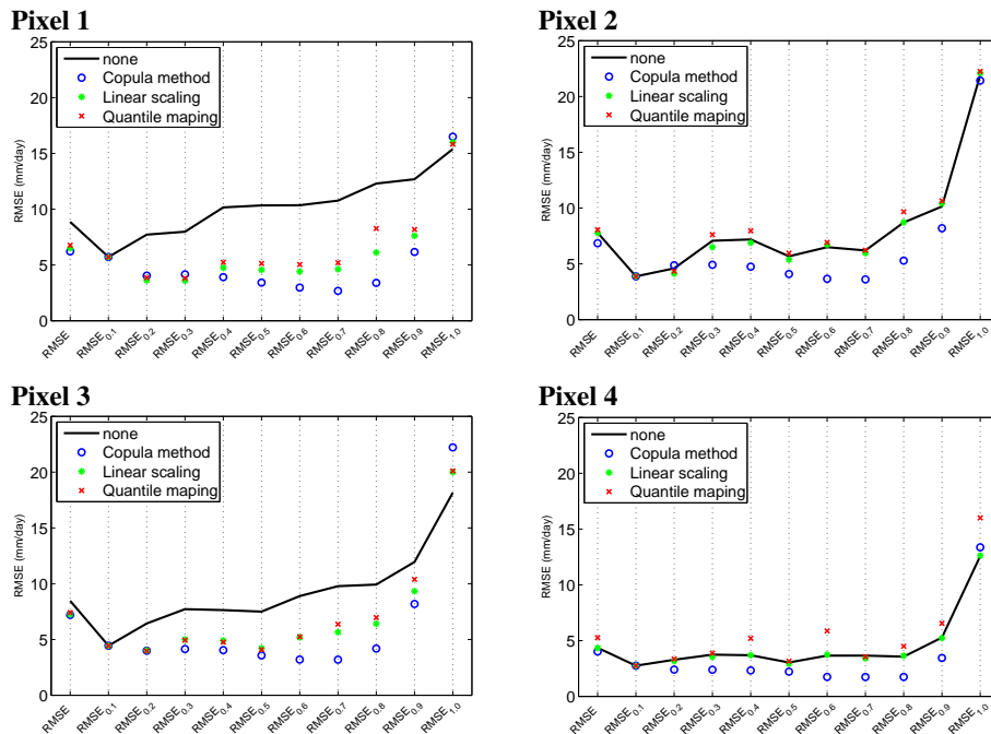
Figure 11. Root mean square errors (RMSE) and the root mean square errors for specific probability intervals ( RMSE_{0.1} , RMSE_{0.2} , ..., RMSE_{1.0} for different methods). The selected four pixel are the same as Fig. 10. The black solid line indicates the errors without correction. The results are derived from the validation period from 1986 to 2000.
