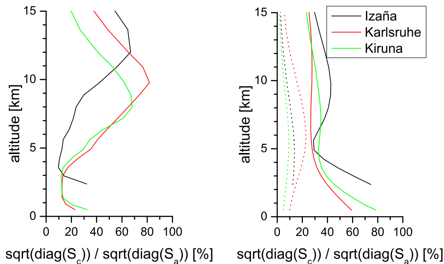
Fig. 6. Level of comparability between both remote sensing datasets at the three different locations. Left panel: H 2 O profile product (product type 1), \mathbf{S}_c calculations according to Eq. (9); Right panel: consistent humidity and \delta D data (product type 2), solid lines for \mathbf{S}_c calculations according to Eq. (9) and dashed lines for \mathbf{S}_c^{\text{sm}} calculations according to Eq. (10).
