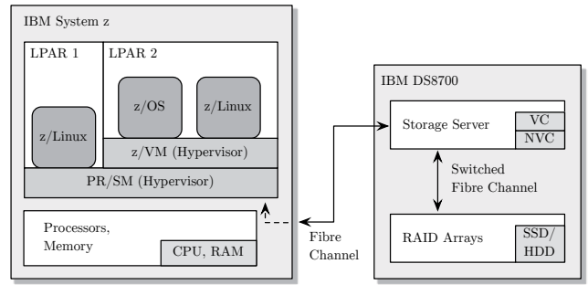
Figure 6: Conceptual design of IBM System z and DS8700
