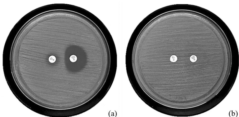
Fig. 4.1: D-test of an iMLS B S. cohnii ssp. urealyticum strain isolated from sewage before (a) and after mutation (b). “D-formation” around a 2 µg clindamycin containing disc adjacent to a disc spotted with 15 µg erythromycin by the “wild strain” (a) and acquired constitutive resistance against clindamycin by a culture that was pregrown in the presence of 5 µg clindamycin ml -1 (b)
