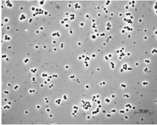
Abb. 2.5: Staphylococcus aureus ssp. aureus DSMZ 346
