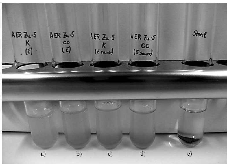
Fig. 3.6: Growth of erythromycin induced, iMLS B phenotype S. cohnii ssp. urealyticum in Mueller-Hinton broth (a) or Mueller-Hinton broth + 1 mg L -1 clindamycin (b) and of anhydroerythromycin-induced cells in Mueller-Hinton broth (c) or Mueller-Hinton broth + 1 mg L -1 clindamycin (d). Vial (e) was a sterile control.
