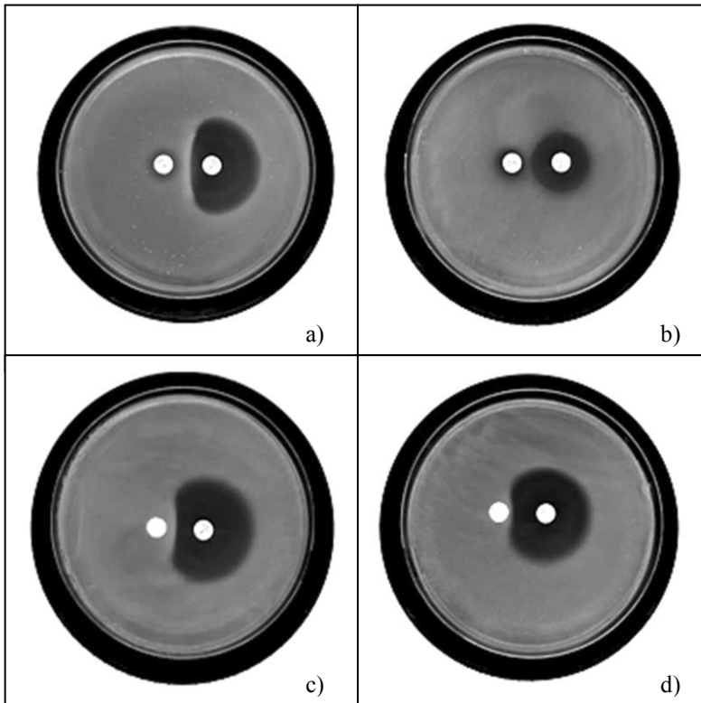
Fig. 3.2 a-d: D-tests with Staphylococcus isolates. 3.2a) D-test-positive S. cohnii ssp. cohnii with 15 µg erythromycin E (left disc) and 2 µg clindamycin CC (right disc). 3.2b) D-test-negative S. cohnii ssp. cohnii with 15 µg erythromycin E (left disc) and 2 µg clindamycin CC (right disc). 3.2c, d) D-test-positive S. cohnii ssp. cohnii with only 25 ng erythromycin E (3.2c) or 25 ng anhydroerythromycin (3.2d, left discs) and 2 µg clindamycin CC (right discs).
