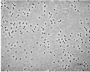
Abb. 2.4: Enterococcus faecalis DSMZ 12956
