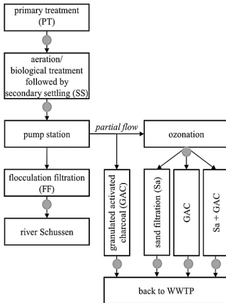
Fig. 5.1: Schematic overview of WWTP Eriskirch and the pilot station with ozonation followed by sand filtration (Sa) and/or granulated activated charcoal (GAC). The combination filter Sa+GAC was substituted in August 2013 against a GAC filter examining the effect of GAC solely without prior ozonation. Grey dots indicate sampling stations.
